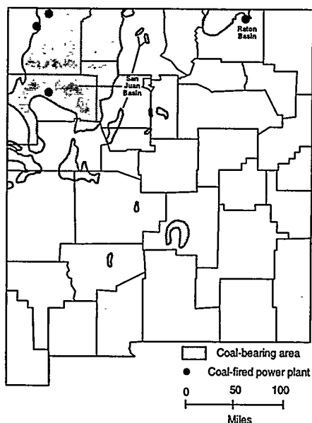
Figure 3. Coal-Bearing Areas of New Mexico
