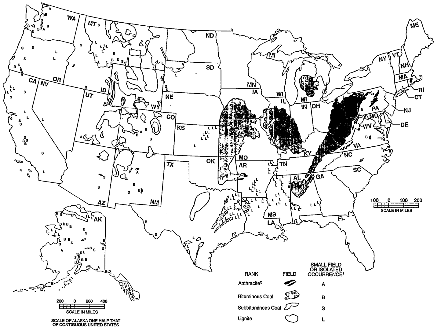
Figure 1. Coal-Bearing Areas of the United States
