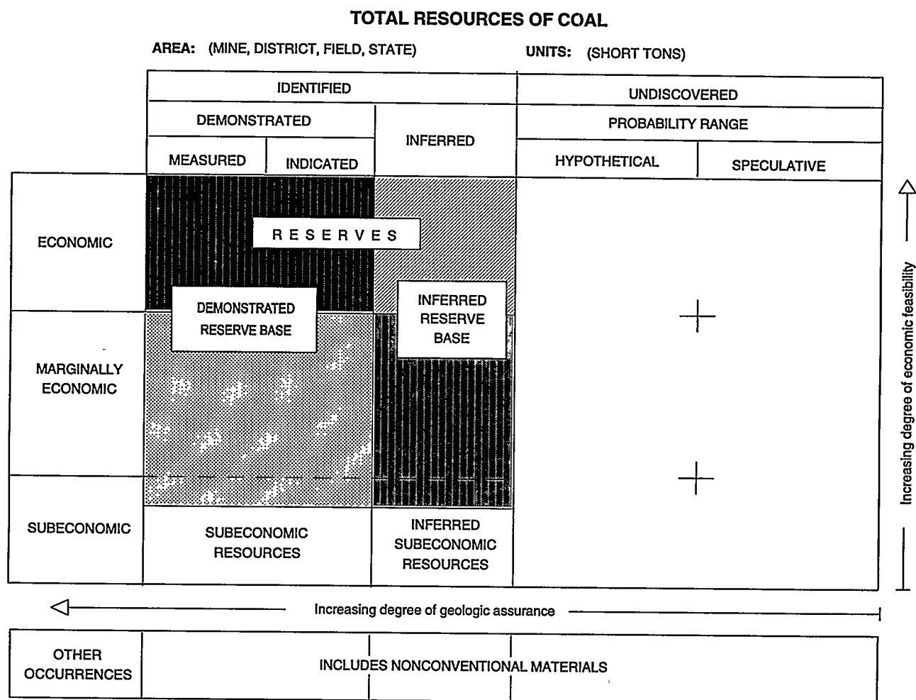
Figure A2. Classification of Coal Resources and Reserves
