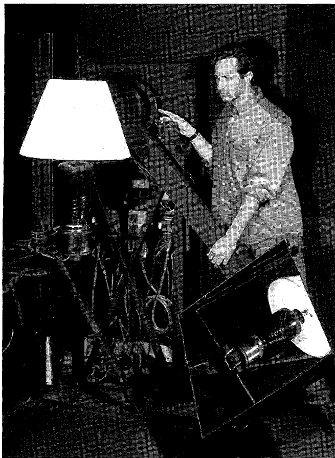
Figure 6. Researcher checks the alignment of LBL's recently completed mirror-based gonio-photometer. A gonio-photometer is used to measure the angular distribution of light (candlepower) emanating from a lighting fixture.
