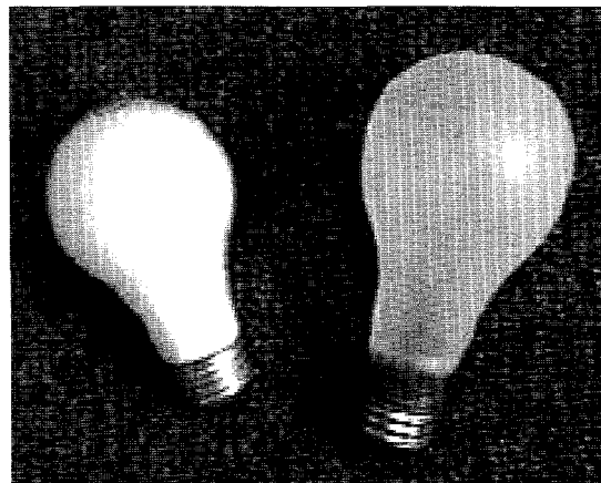
Figure 4. A standard 100-watt incandescent lamp (left) produces 1750 lumens and has a 750-hr life. The prototype selective reflector (SR) lamp built at LBL shown at the right also uses 100 watts but produces 2600 lumens and has a 3000-hr life.
