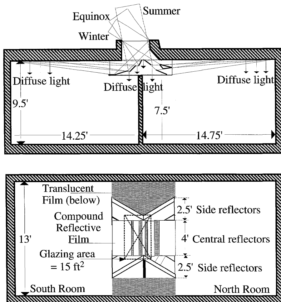
Figure 11. Design of the reflector system used in the prototype skylight for the Palm Springs Chamber of Commerce. This reflector system was designed to split the incoming daylight flux and redirect it to the ceiling plane of two separate rooms. The central reflector (center) optimizes daylight redirection for the noon hour throughout the year. The side reflectors (left and right "wings") optimize daylight redirection for late afternoon and early morning hours. The system uses a combination of several different 3M reflective films to maximize daylight reflection and redirection.
