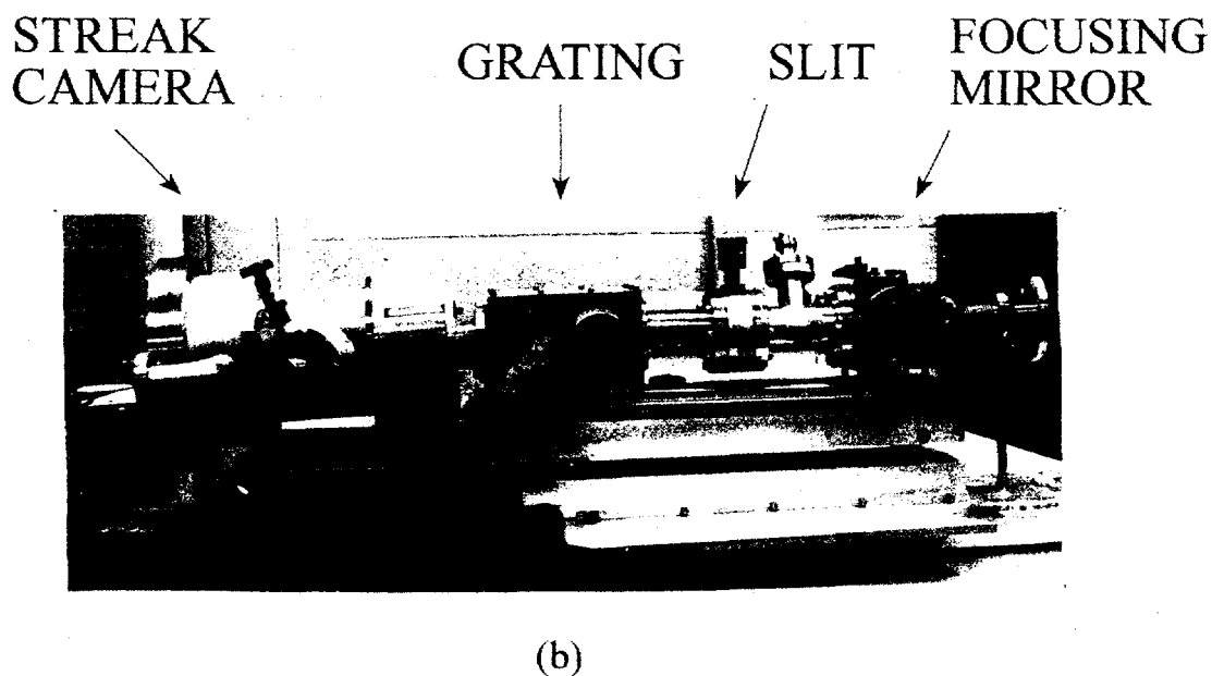
Fig. 1. Spectrograph shown before mounting on Omega Upgrade, with film holder (a) and streak camera (b).
