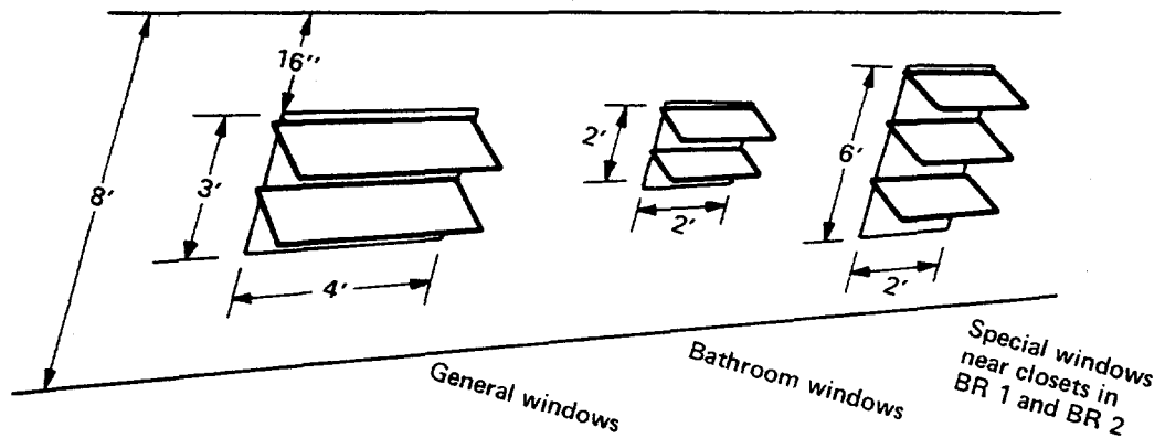
Figure 25 Recommended Window Types and Sizes
