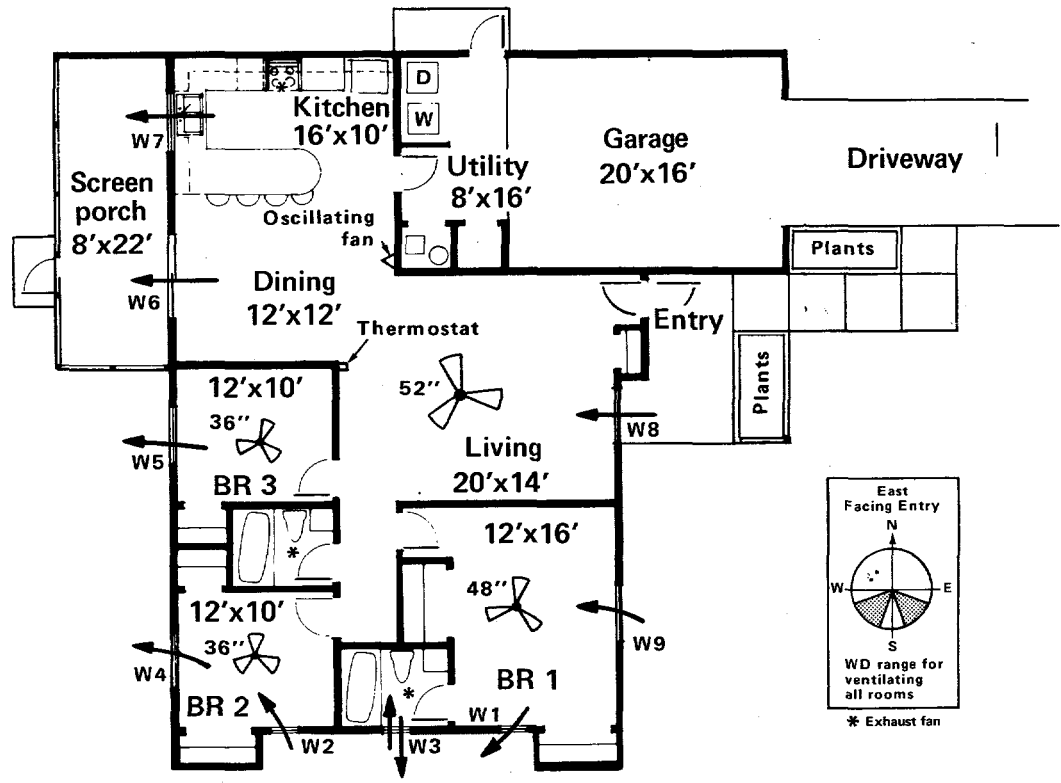
Figure 29 A House Plan for East-Facing Lots
