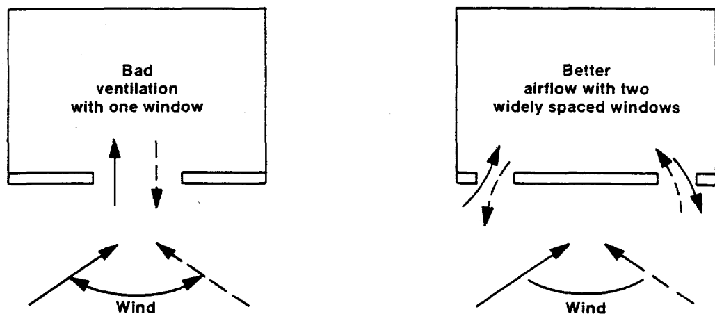
Figure 12 Two Windows Ventilate Better Than One in Rooms With One Outside Wall
