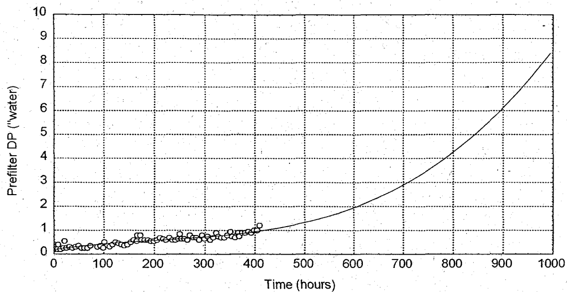
Figure 4 Run 3 HEPA Filter Performance
