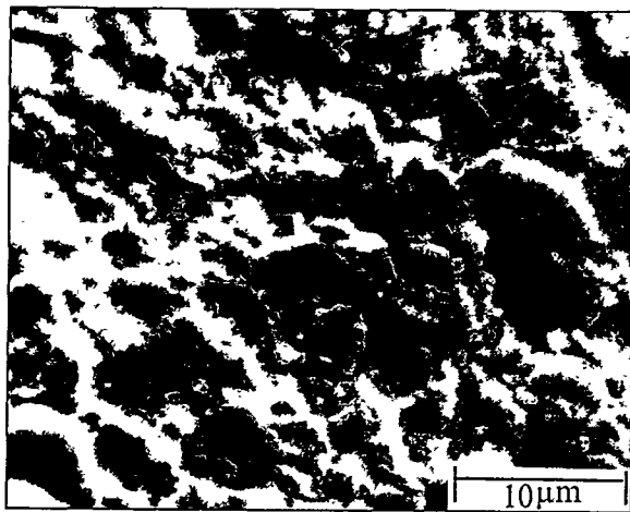
c) R/R_0 \sim 0.96
