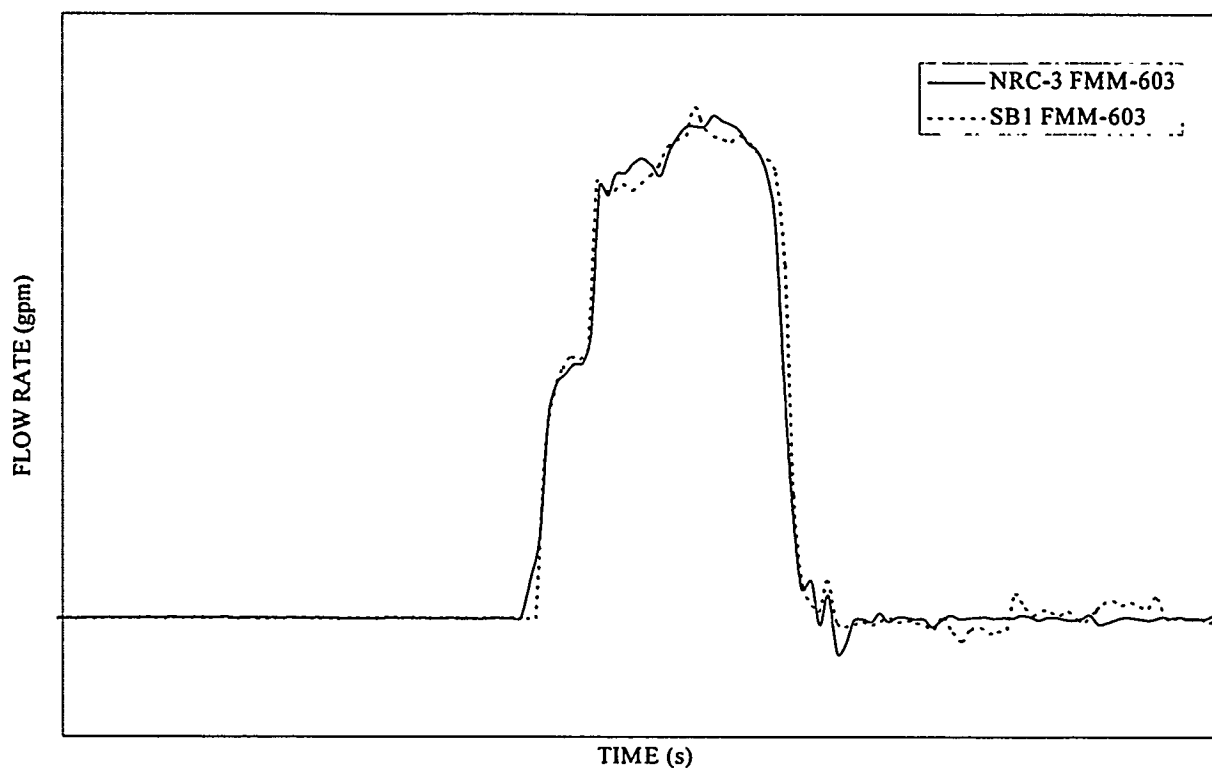
Figure 5. Comparison of NRC-3 (2/95) and SB1 (6/94) Accumulator Flows
