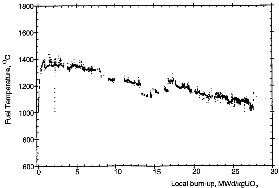
Fig. 3: Fuel centre temperatures at 25 kW/m in a Xe filled rod with 100 \mu\text{m} as fabricated gap. The gap conductance improvement due to gap closure outweighs fuel conductivity degradation.
