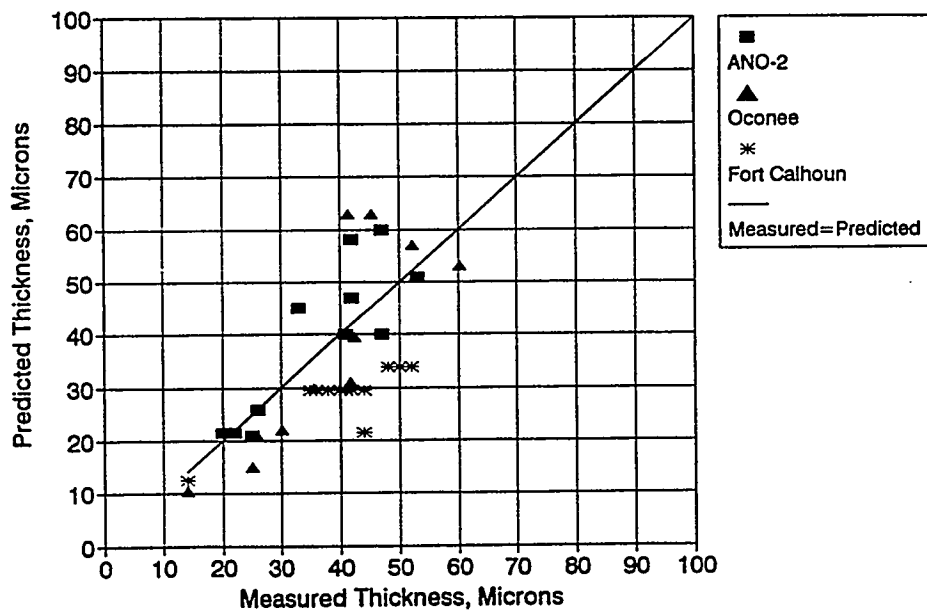
FIGURE 11. Comparison of Garzarolli Model (Reference 35) Predictions to Corrosion Data From High Burnup Fuel Rods
