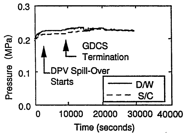
Fig. 24 TRAC Prediction of Pressure Response (DLB Case)
