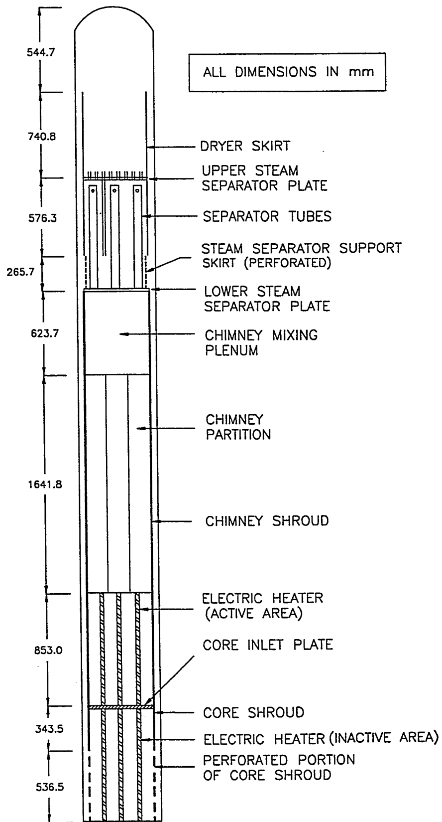
Fig. 4 Schematics of PUMA Reactor Pressure Vessel Internals
