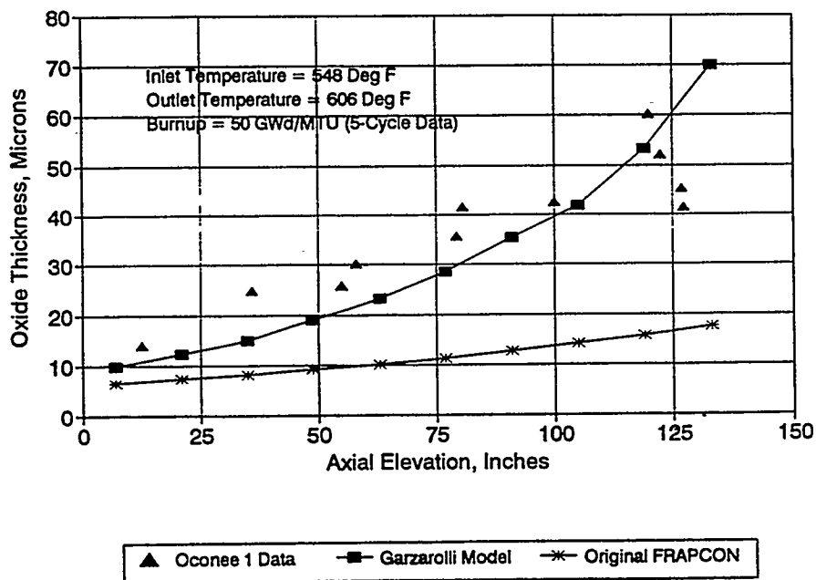
FIGURE 12. Comparison of Original and Garzarolli Corrosion Model (Reference 35) Predictions to Axial Corrosion Data From an Oconee-1 Cycle 5 Fuel Rod (Reference 25)
