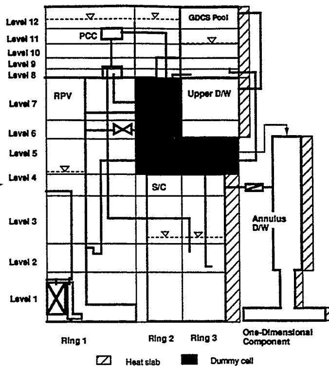
Fig. 21 TRAC Nodalization for GIRAFFE Analysis
