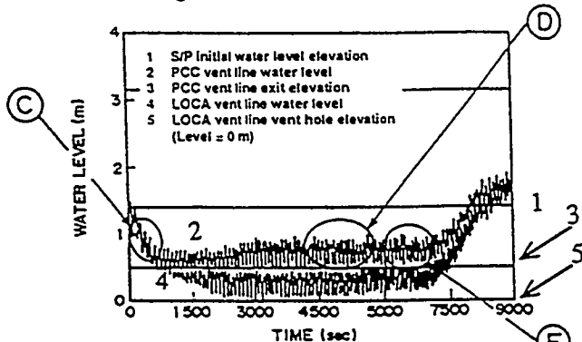
Fig. 7 PCC Vent and Main LOCA Vent Water Levels
