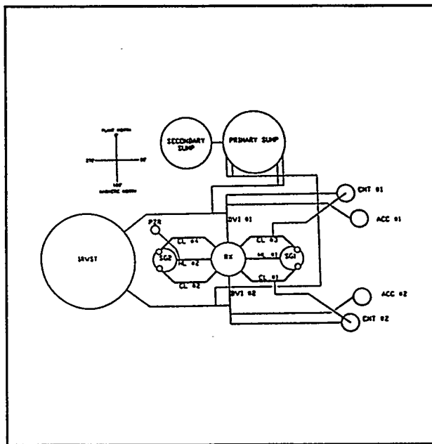
Figure 2. Line Diagram of APEX Test Facility
