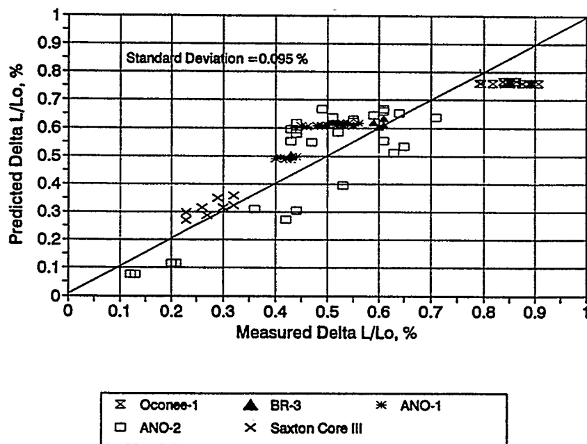
FIGURE 20. Comparison of Franklin Axial Growth Model (Reference 36) Predictions to PMR Data With Rod Average Fast Fluences up to 9 \times 10^{25} \text{ n/m}^2
