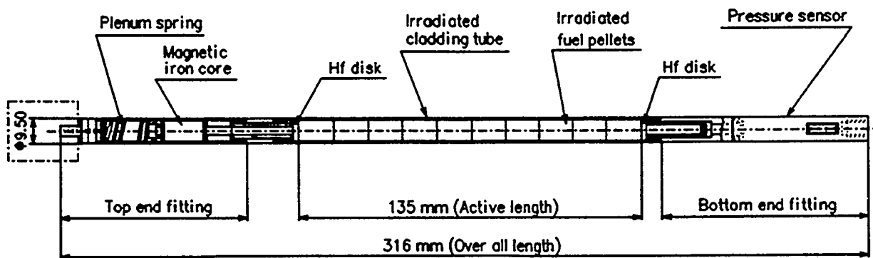
Fig. 4 Schematics of the HBO test fuel (segmented 50 MWd/kgU PWR fuel)
