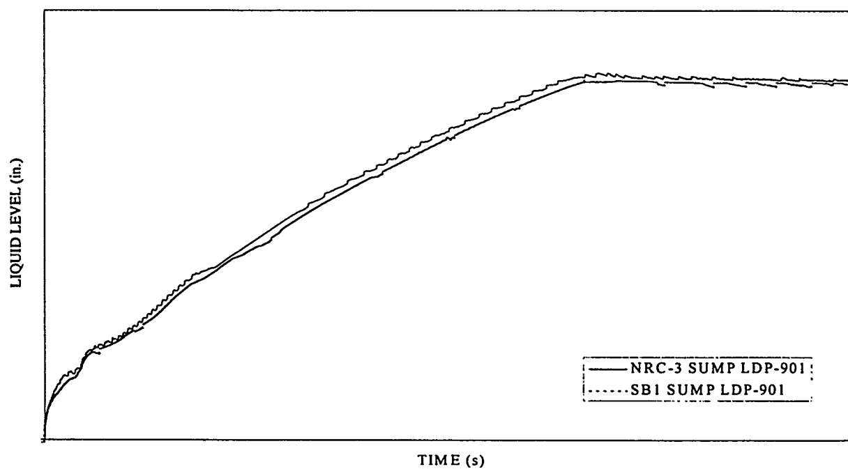
Figure 6. Comparison of NRC-3 (2/95) and SB1 (6/94) Primary Sump Liquid Levels
