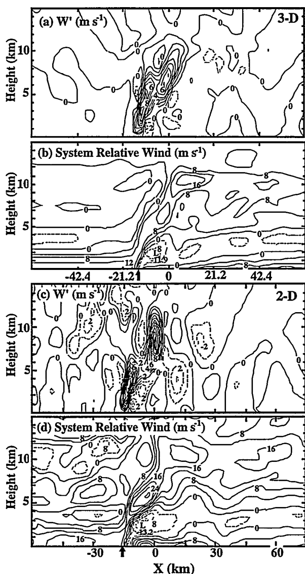
Fig. 5. Crosssections in the vertical-horizontal plane of induced vertical velocity and system-relative horizontal velocity in intervals of 1 and 4 \text{ m s}^{-1} , respectively, at 4 hour of simulation time. (a) and (b) 3-D simulation. (c), (d) 2-D simulation.
