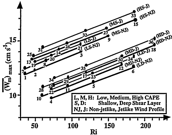
Fig. 3. Maximum stratiform ascent strength ((W_m)_{\max}) versus the bulk Richardson number (Ri) for varied convective available potential energy, wind shear intensity, shear depth, and shear profile pattern for multicellular storms. The numbers beside the dots represent the experiments, listed in Table 1.
