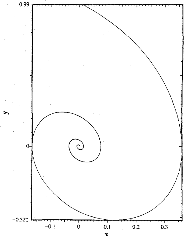
SPARK Plot of Trajectory of Damped Oscillator
