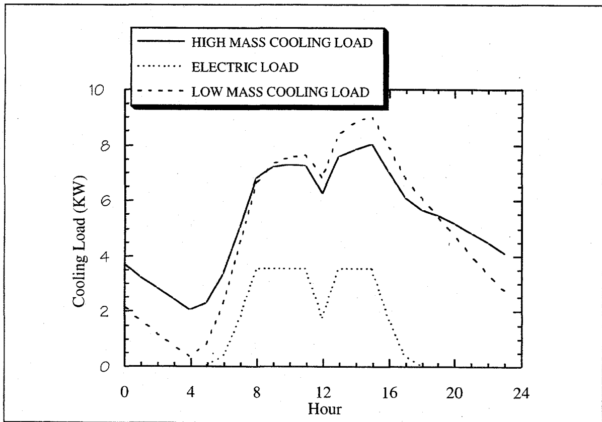
Figure 2. BLAST Sensible Zone Cooling Load for High and Low Mass Constructions
