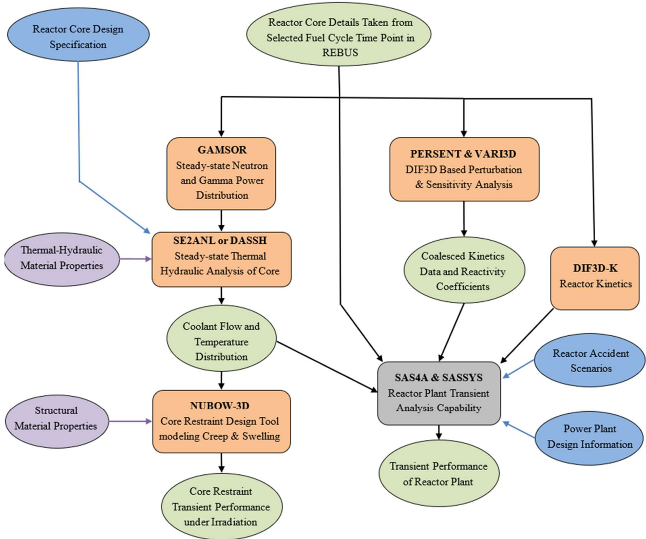
Figure 2.2. ARC Software Connections for Fast Spectrum Reactor Analysis
