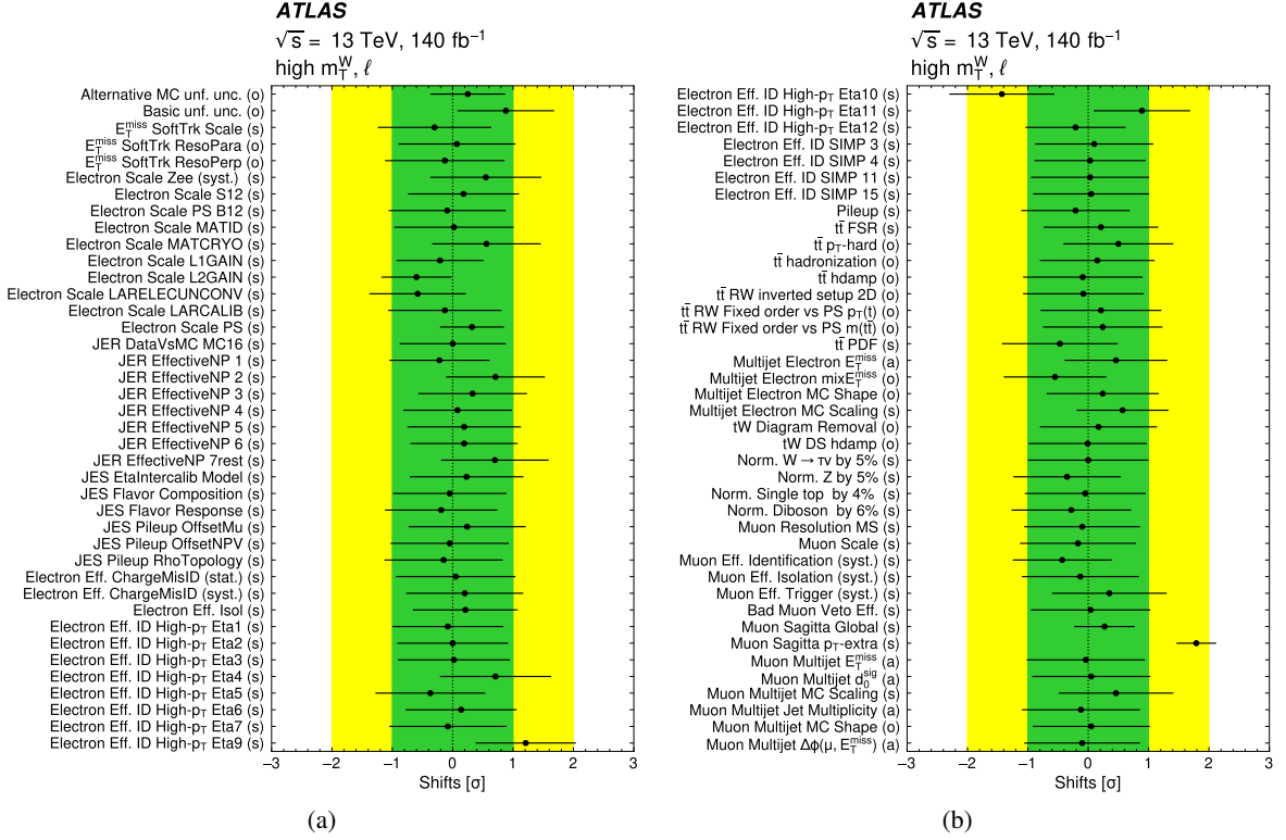
Figure 15: Shifts of the systematic uncertainty nuisance parameters after the combination of the double-differential electron and muon cross-sections. The systematic uncertainties are related to the unfolding procedure (“unf.”), the jet energy resolution/scale (“JER/JES”), the E_T^{\text{miss}} scale and resolution, the electron and muon scale, resolution and efficiency (“Eff.”), the multijet and t\bar{t} (where RW refers to a reweighting to NNLO) background estimates and normalization of small background processes (“Norm.”). The uncertainties are marked whether they are symmetric (“s”), asymmetric (“a”) or one-sided (“o”). The systematic uncertainties labeled with “Electron” or “Muon” are not correlated between the lepton flavours.
