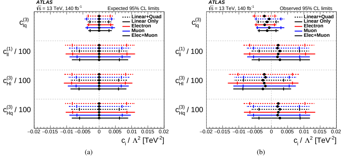
Figure 21: The (a) expected and (b) observed limits on Wilson coefficients at 95% CL. The results are shown for linear-only and linear+quadratic fits, for both the electron and muon channels, as well as their combination. The inner (outer) error bars indicate the limits when using the 68% (90%) CL for the PDF uncertainty.
