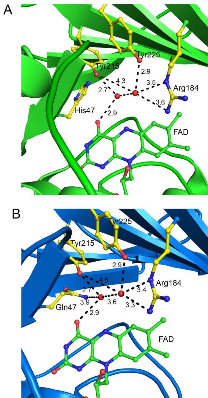
Figure 4. The conserved water network in NicC. A. The wild type NicC has two water molecules that mark the 2-MP binding site in the ligand structure. Carbon atoms are shown in yellow for the NicC residues and in green for the FAD coenzyme, oxygen atoms are shown red, and nitrogen atoms in blue. Distances are shown in Angstroms (Å) with dashed black lines. B. The same water molecules are also conserved in the H47Q NicC structure. Same coloring scheme as in A.
