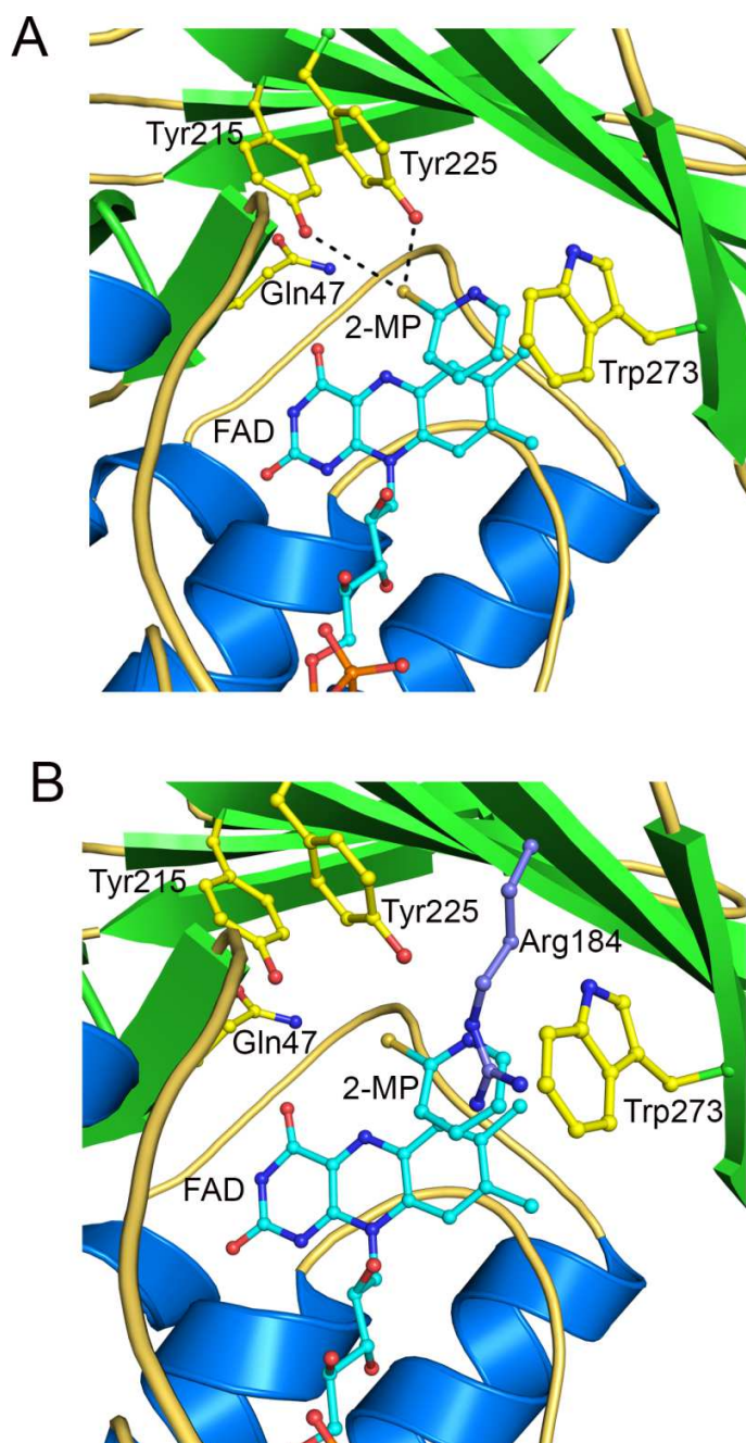
Figure 3. The H47Q NicC active site. A. Residues in the 2-MP binding pocket are highlighted. H47Q NicC protein residues are shown in ball and stick mode with yellow carbon atoms, red oxygen atoms, blue nitrogen atoms, orange phosphorous atoms, and dark yellow sulfur atoms. FAD and 2-MP are also shown in ball and stick mode with cyan carbon atoms. Potential interactions are highlighted with dashed black lines. B. The potential role of Arg184 in substrate binding is highlighted. An overlay of the H47Q NicC in the presence and absence of 2-MP is shown. Coloring as in Part A. In addition, the carbon atoms of Arg184 from the unliganded H47Q NicC structure are shown with purple carbon atoms and dark purple nitrogen atoms. The side chain of Arg184 is disordered in the liganded H47Q NicC structure.
