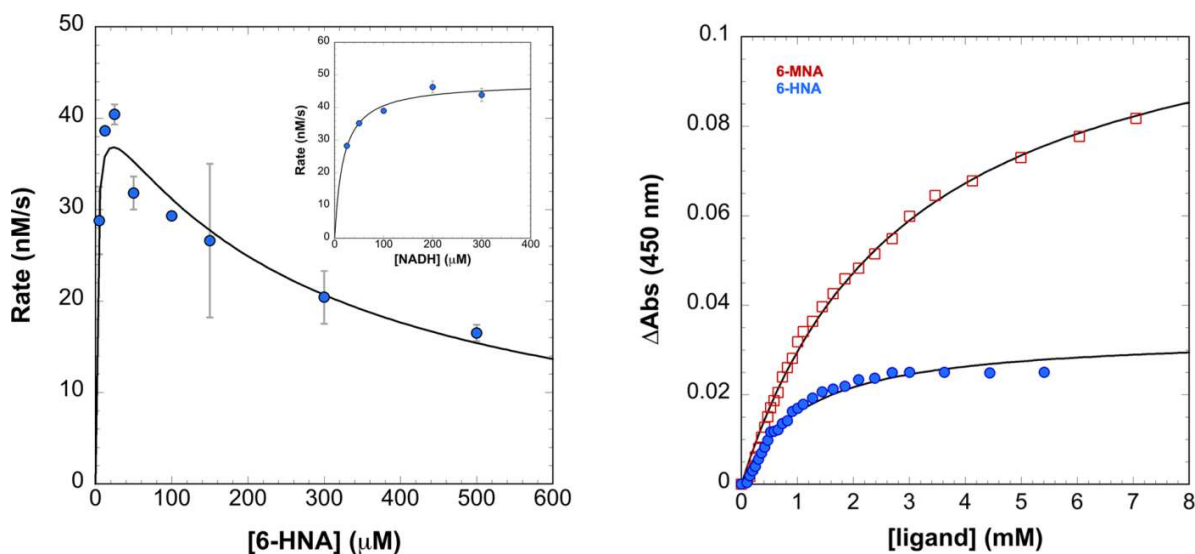
Figure 1. Catalytic activity of NicC with 6-HNA and the binding of 6-MNA. A. Steady-state kinetic analysis of NicC variant H47Q with 6-HNA indicates substrate inhibition. Data fits to V_{\max}/[E] = 0.86 \pm 0.08 \text{ s}^{-1} , K_M(6\text{-HNA}) = 2 \pm 1 \text{ } \mu\text{M} , and K_i(6\text{-HNA}) = 0.28 \pm 0.07 \text{ mM} . Inset shows initial rates measured with constant concentrations of 6-HNA of 20 \text{ } \mu\text{M} ( 10 \times K_M ) and enzyme ( 50 \text{ nM} ) with increasing concentrations of NADH ( 25 - 300 \text{ } \mu\text{M} ). Data fit with the Michaelis-Menten equation estimates a K_M(\text{NADH}) of 18 \pm 3 \text{ } \mu\text{M} and V_{\max}/[E] = 0.95 \pm 0.03 \text{ s}^{-1} . B. Equilibrium titrations of the H47Q variant of NicC ( 30 \text{ } \mu\text{M} ) with 6-HNA (blue circles) and 6-MNA (red squares) fit to the hyperbolic binding equation estimates a K_d for E·6-MNA of 2.9 \pm 0.1 \text{ mM} and K_d for E·6-HNA of 1.1 \pm 0.1 \text{ mM} .
