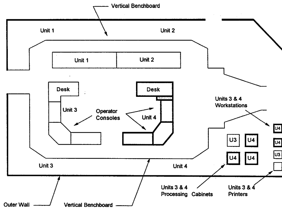
Figure 5-2: Unit 1-4 Control Room Layout as Currently Implemented
