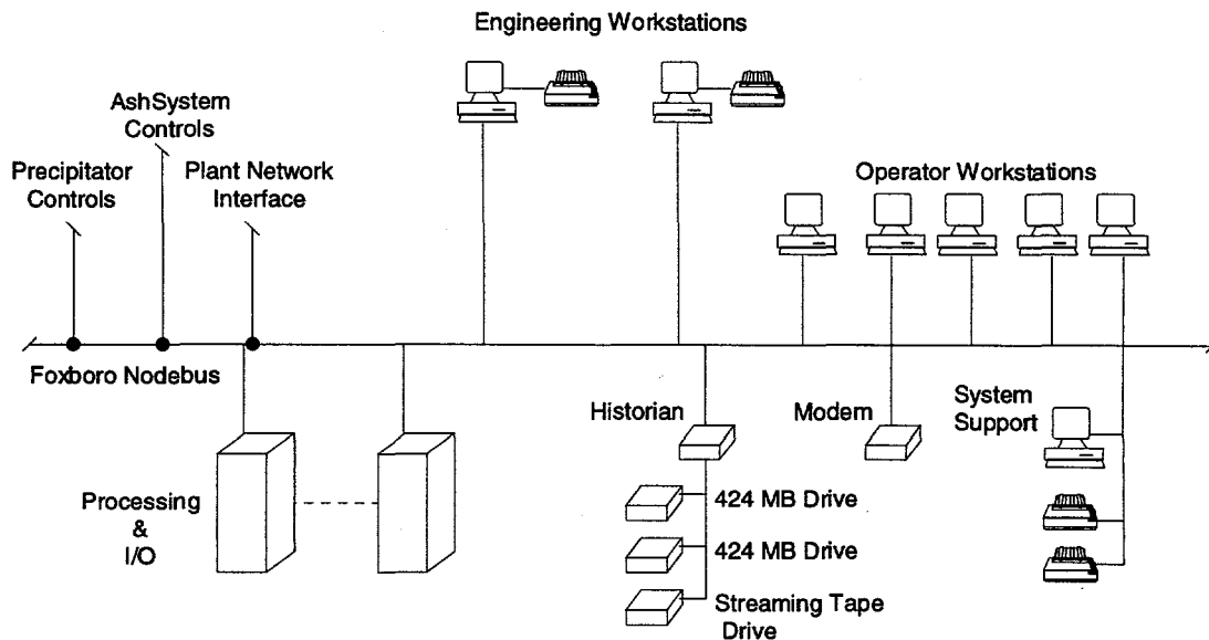
Figure 5-1: Unit 4 DCS Overview
