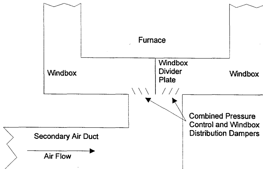
Figure 4-1: Advanced Overfire Air System
