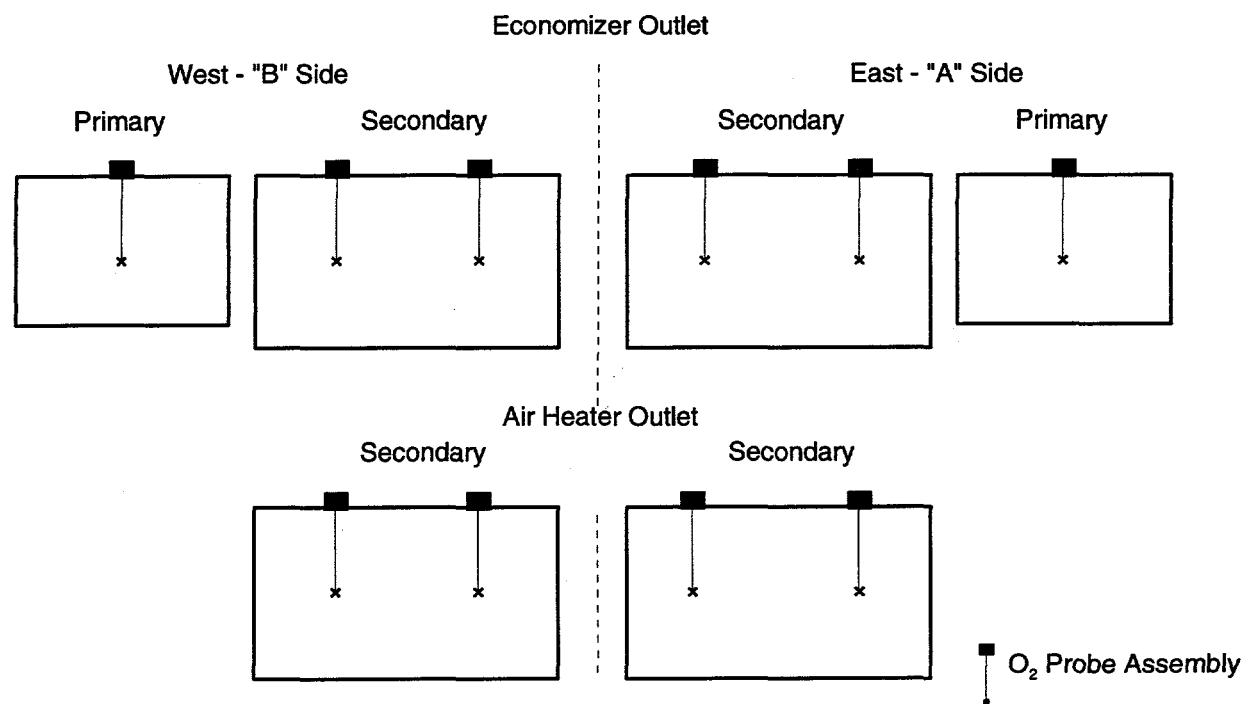
Figure 6-8: O 2 Probe Arrangement
