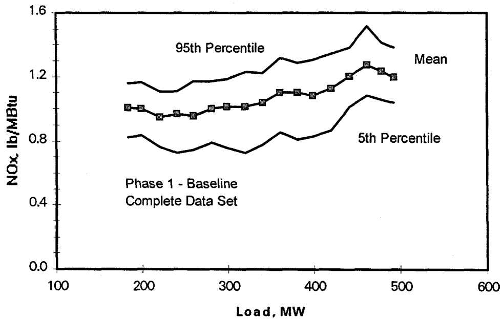
Figure 2-5: Pre-Retrofit NO x Emissions
