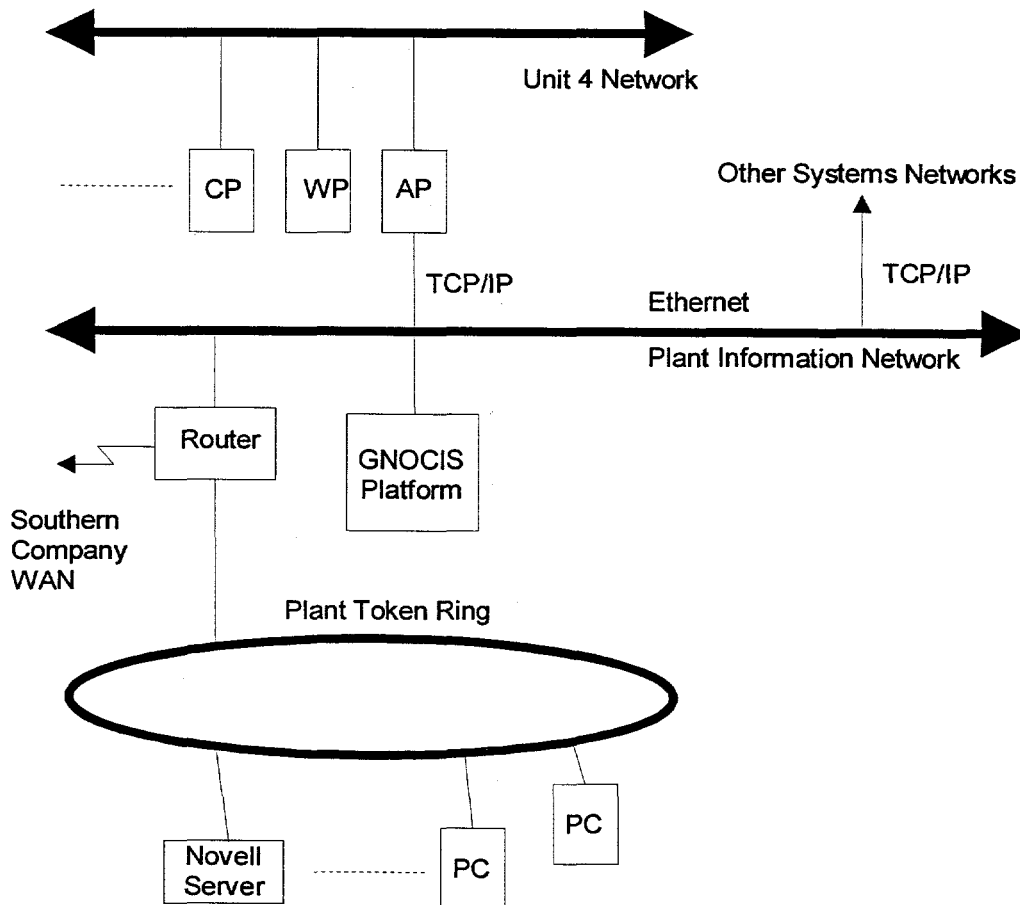
Figure 5-6: Hammond Plant Network
