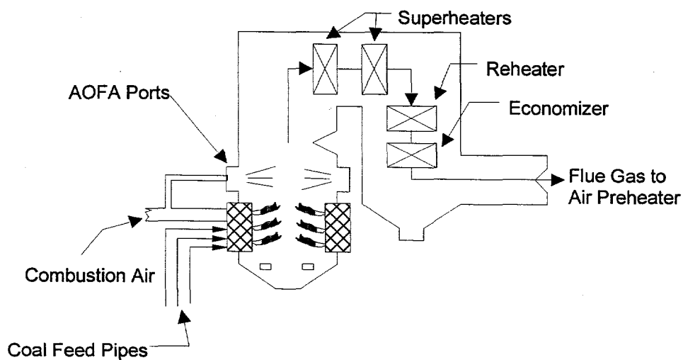
Figure 3-3: Advanced Overfire Air Concept
