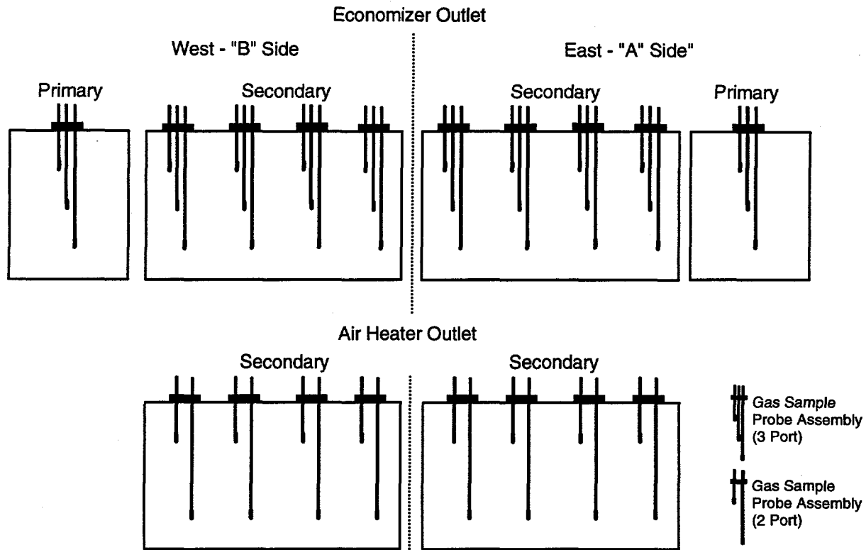
Figure 6-3: Extractive Gas Analysis System Probe Arrangement
