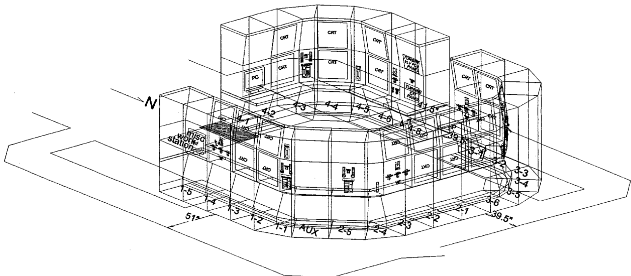
Figure 5-3: Unit 1-4 Control Room Layout (Planned)
