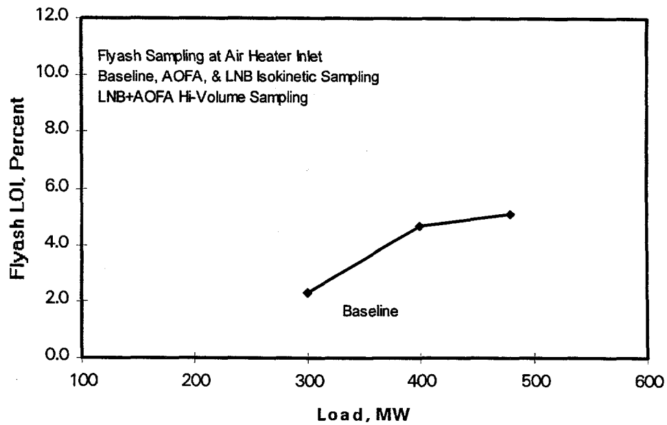
Figure 2-6: Pre-Retrofit Fly Ash Loss-on-Ignition
