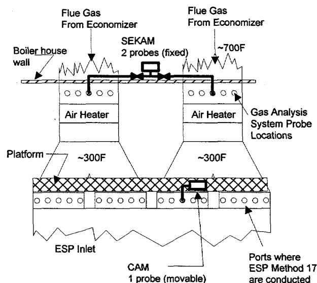
Figure 6-4: Extractive Gas Analysis System Probe Locations
