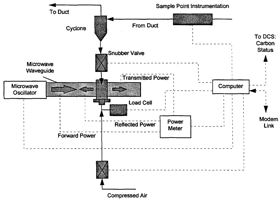
Figure 6-6: CAM Arrangement
