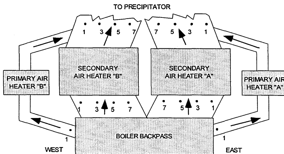
Figure 6-2: Extractive Gas Analysis System Probe Locations
