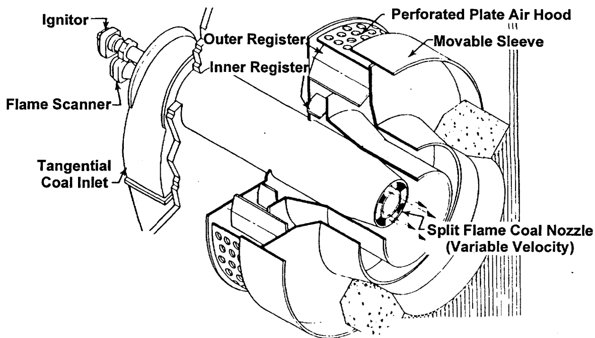
Figure 4-4: FWEC Controlled Flow/Split Flame Burner
