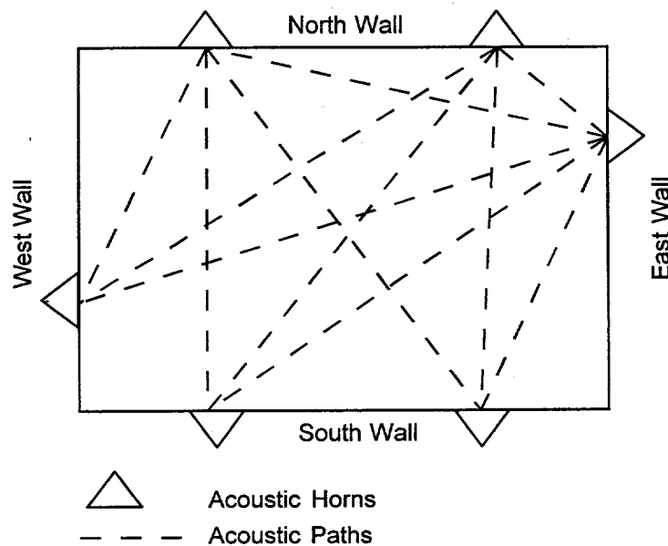
Figure 6-11: Acoustic Pyrometer
