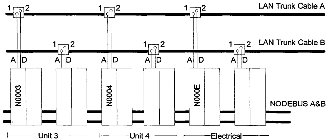
Figure 5-5: DCS Network
