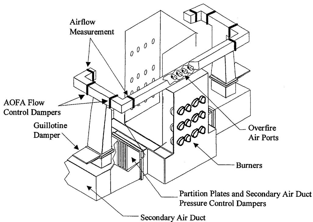
Figure 4-1: Advanced Overfire Air System
