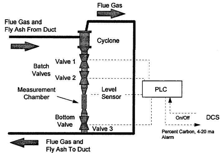
Figure 6-5: SEKAM Arrangement
