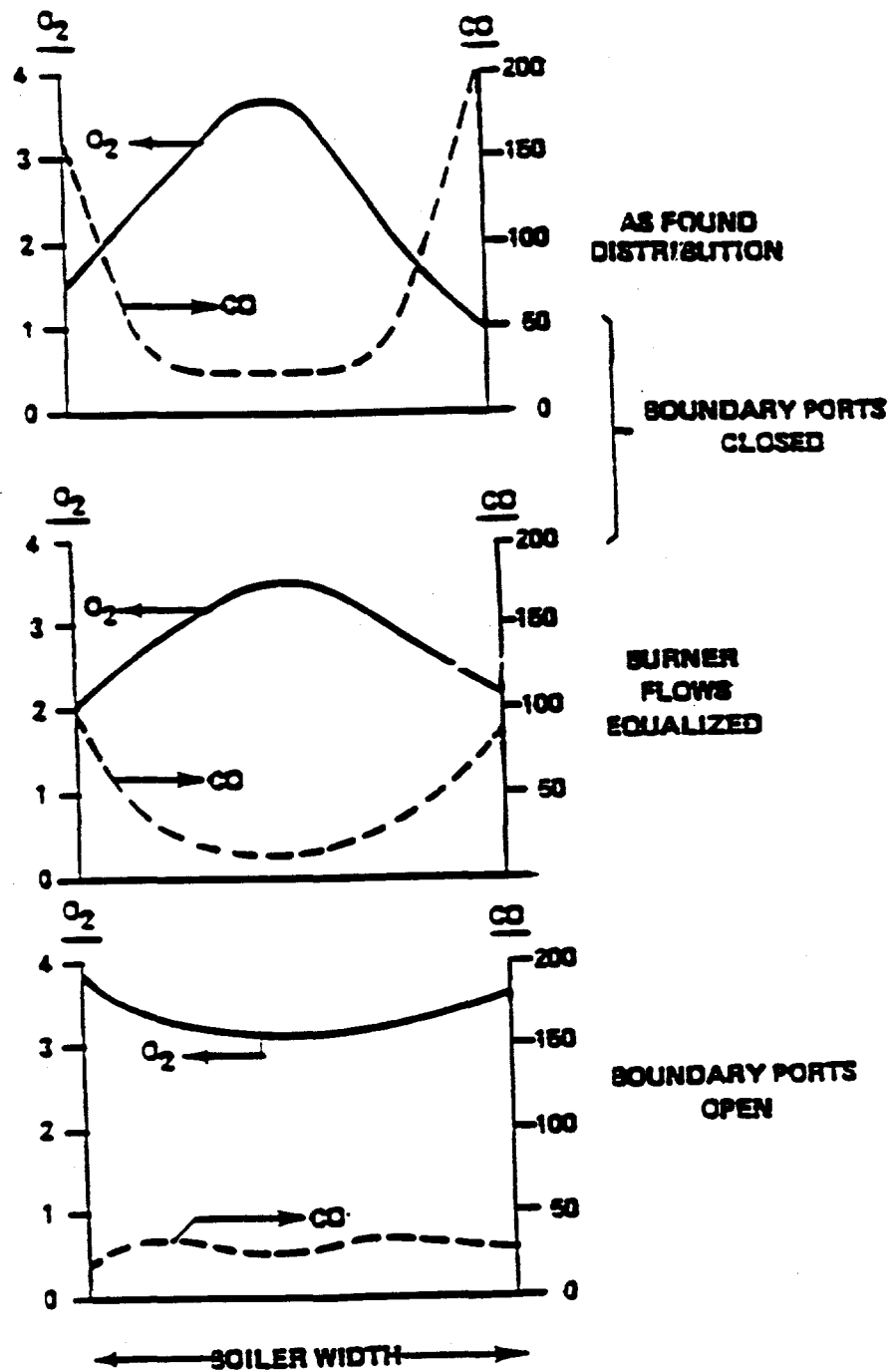
FIGURE 3-2 Effectiveness of Boundary Air and Secondary Air Balancing
