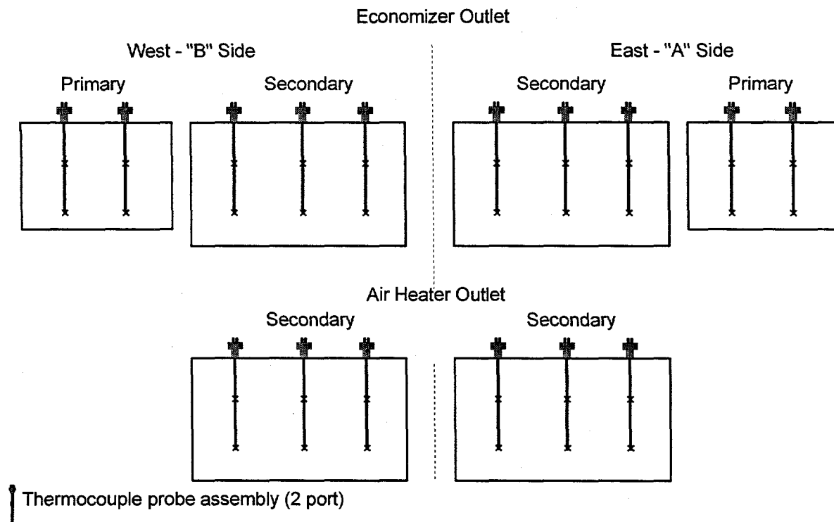
Figure 6-9: Thermocouple Probe Arrangement
