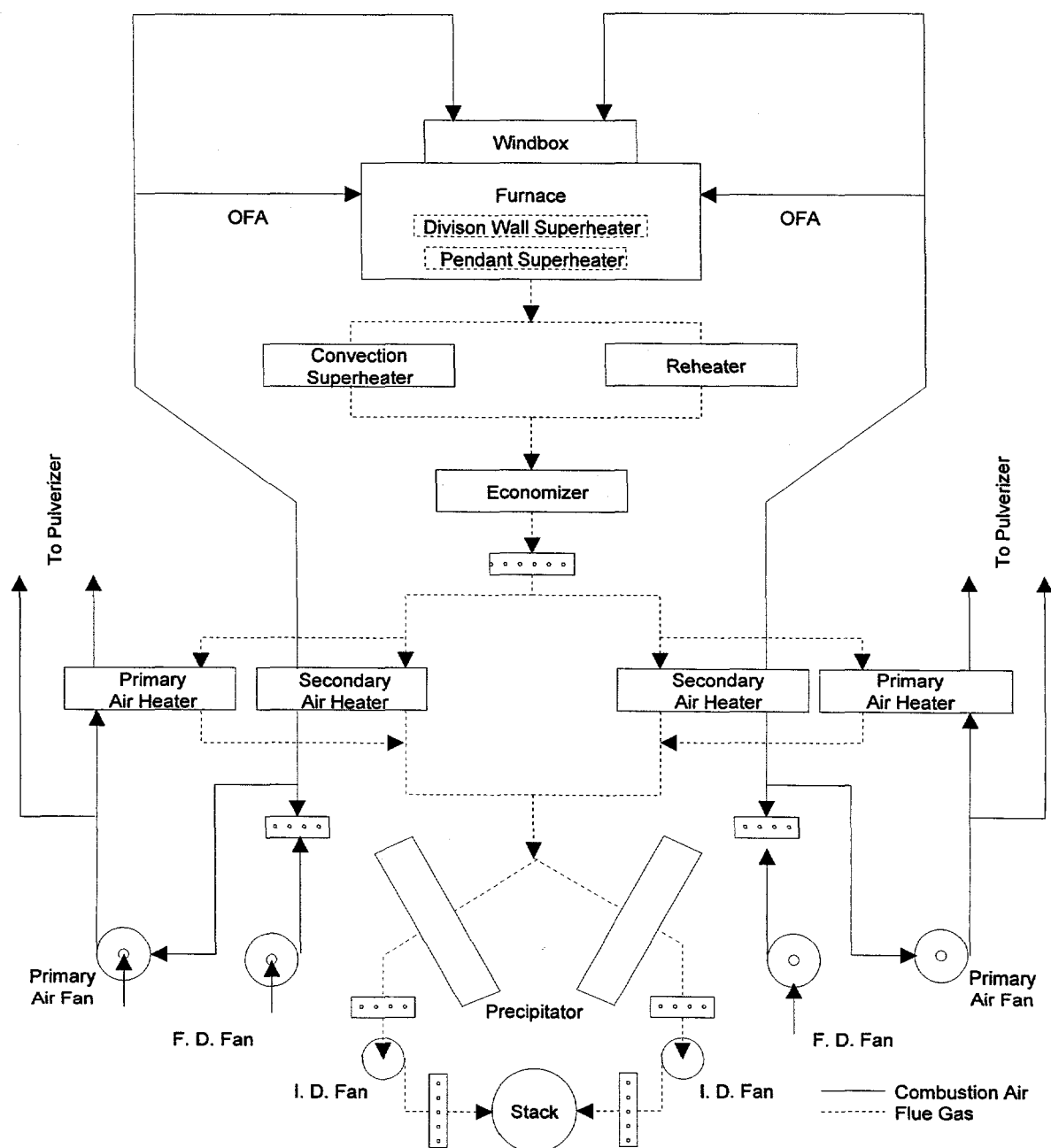
Figure 2-3: Layout of Combustion Air and Flue Gas Paths
