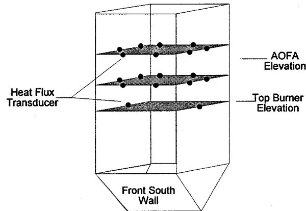
Figure 6-10: Arrangement of Heat Flux Sensors
