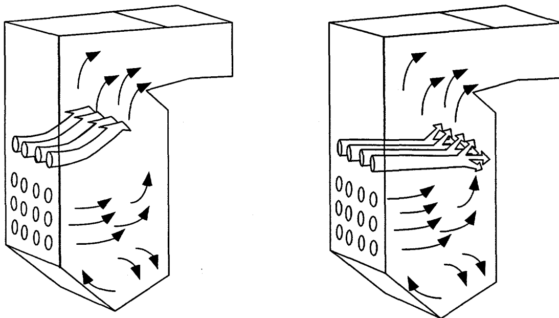
Furnace Flow Patterns with Low OFA Flow
