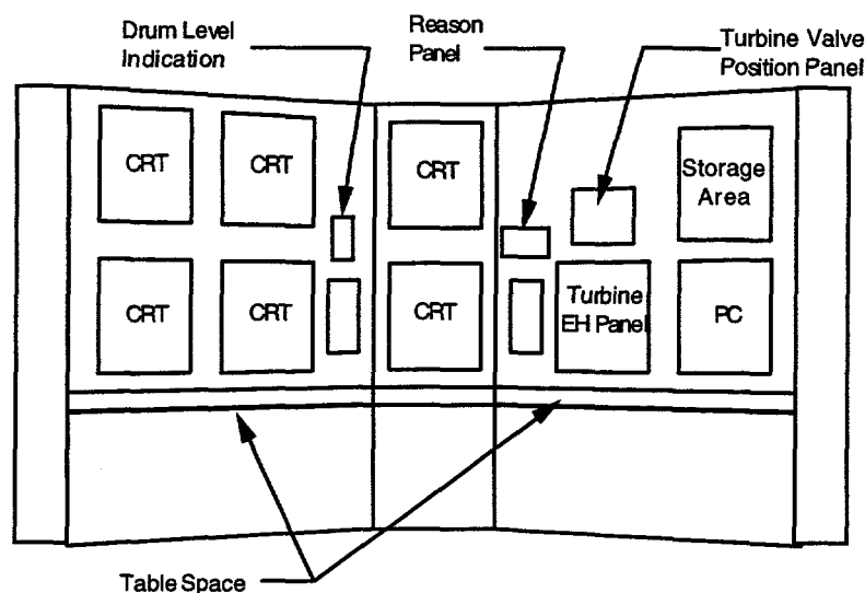
Figure 5-4: Unit 4 Benchboard
