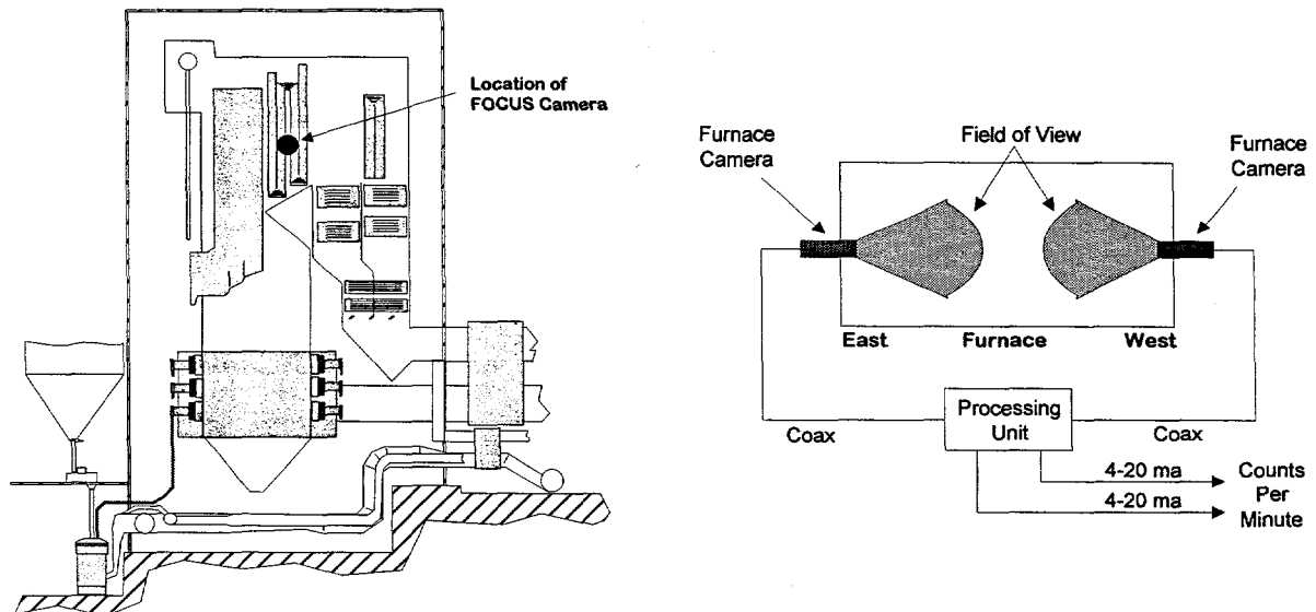
Figure 6-7: FOCUS Arrangement
