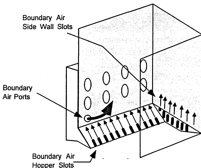
Figure 4-3: Boundary Air System
