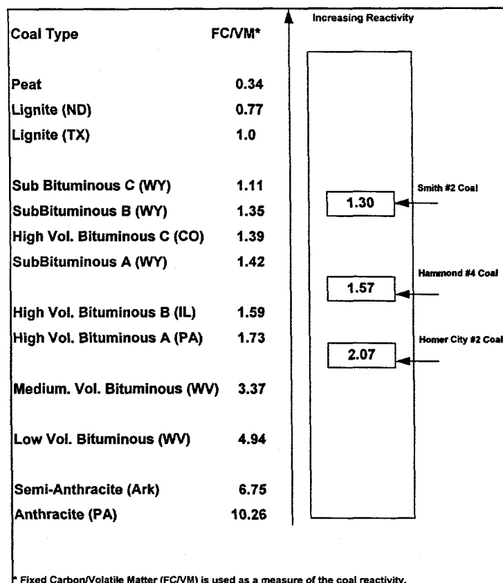
Figure 2-4: Comparison of Hammond Coal Reactivity to Other U.S. Coals
