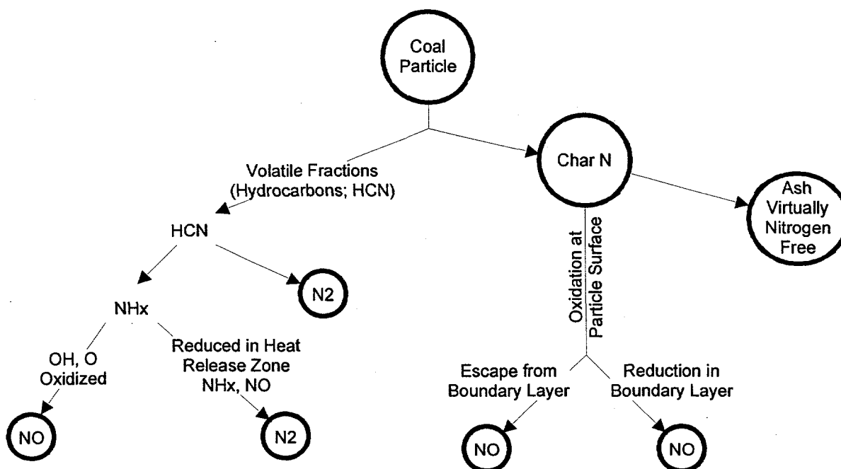
Figure 3-1: Possible History of Fuel Nitrogen
