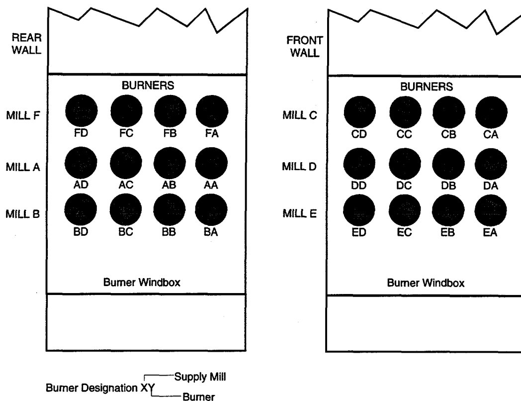
Figure 2-2: Burner Layout
