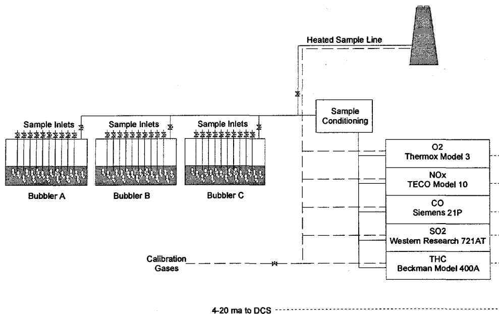
Figure 6-1: Extractive Gas Analysis System
