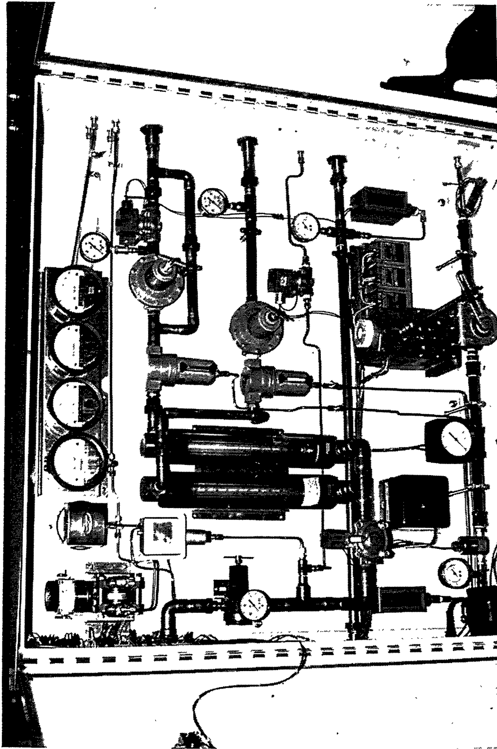
Figure 2.29 Internal Configuration of the Control Enclosure
