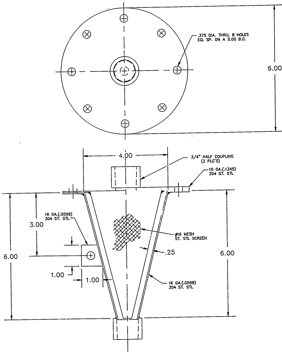
Figure 2.23 Slurry Strainer
