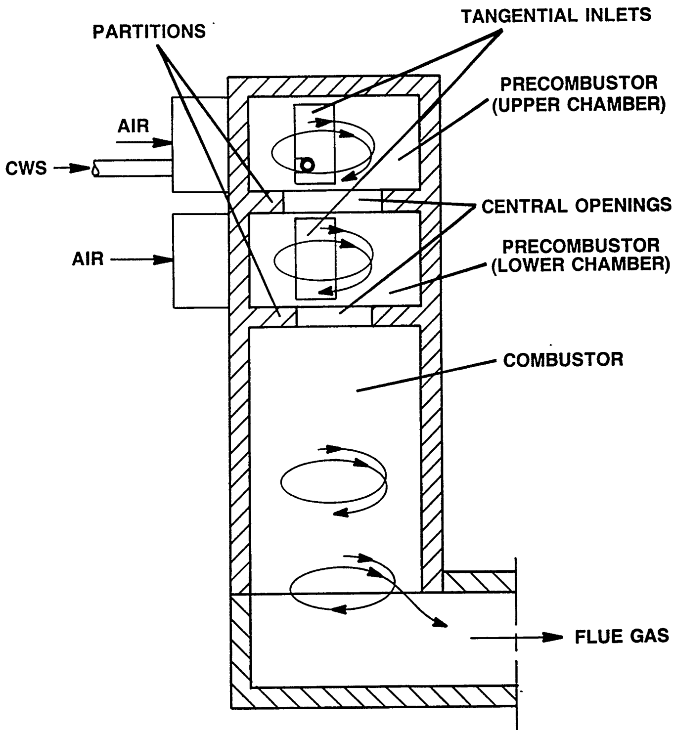
Figure 2.2 Combustor Principle of Operation
