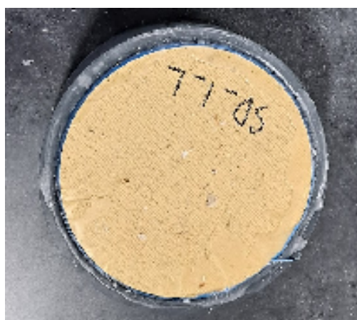
Figure 6. Test cup with the aqueous solution and waxed samples.
