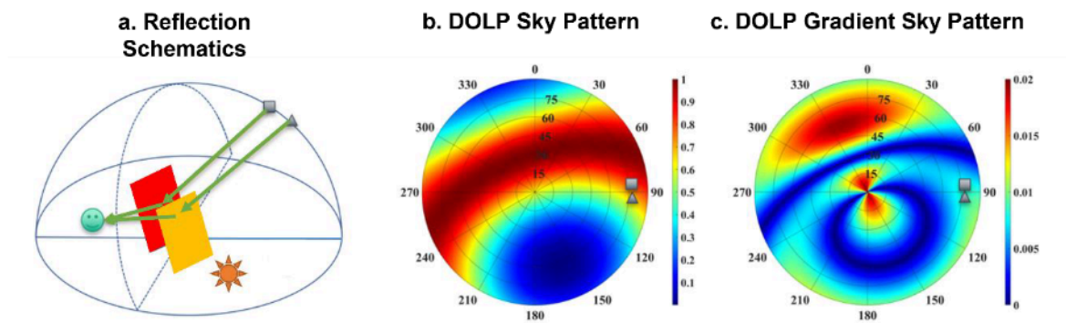
Figure 5. Polarization analysis of the sky-vs-sky scenario. The sky polarization patterns were calculated based on the Rayleigh scattering model [8].
