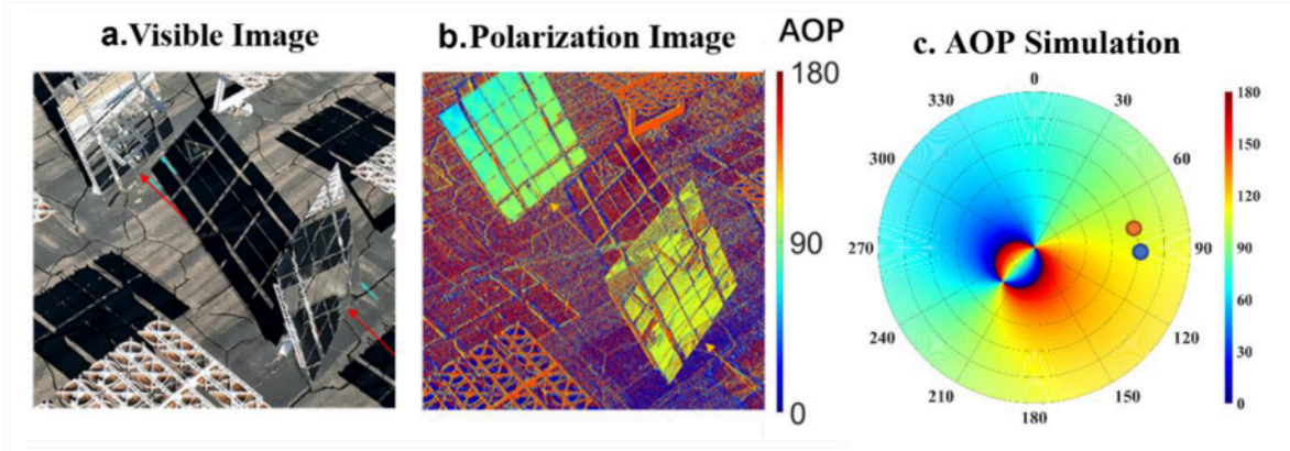
Figure 6. Example for ground-vs-ground scenario where the visible image (a) shows low contrast on the bottom edge to the ground, but the angle of polarization image (b) shows good contrast. The corresponding simulation of the sky [8] AOP pattern (c) is useful to predict AOP of the mirror reflection.
