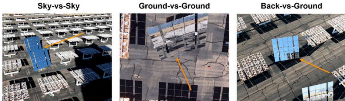
Figure 3. Examples of different scenarios that are challenging for conventional image processing techniques. In each case, some mirror edges appear very similar to adjacent background.
