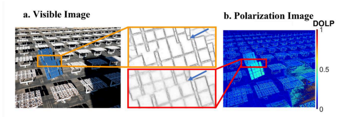
Figure 4. An example sky-vs-sky scenario where processing the conventional image did not have enough contrast to detect the edge between adjacent heliostats, but the increased contrast in the degree of linear polarization image enabled edge detection.
