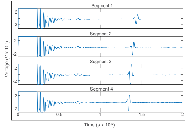
Fig. 3: Ultrasound propagation across the segments of the sample V+ (orthogonal to the build direction). Note the reduction in the echoes' time of flight with the segment's number.
