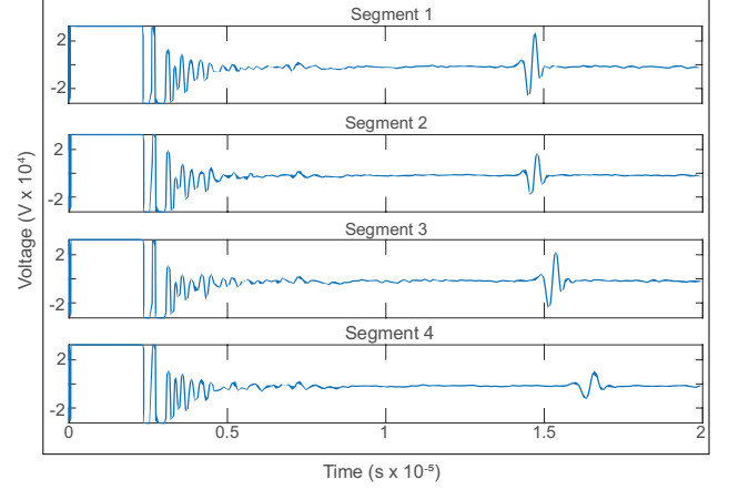
Fig. 4: Ultrasound propagation normal to the build directions across the segments of sample V-. The echoes' time of flight increases with the segment's number.
