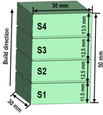
Fig. 1: Geometry and segmentation of SLM-fabricated stainless-steel samples.
