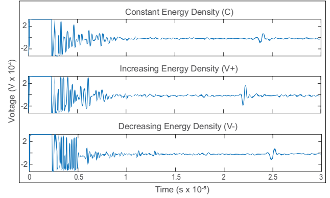
Fig. 2: Ultrasonic propagation in the build direction. The waveforms show faster arrival of the ultrasonic signal in the V+ sample and the increase in the TOF in the V- sample.
