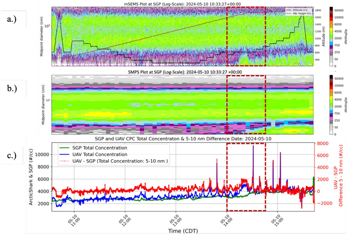
Figure 4. Comparison of aerosol measurements between the ArcticShark and surface instrumentation at the SGP field site. 4a shows the aerosol size distribution measured by the mSEMS aboard the ArcticShark, while 4b presents the aerosol size distribution from the SMPS at the SGP site. 4c displays a time series of aerosol concentration, comparing measurements from the ArcticShark (blue), the surface (green), and the difference between the two (red).
