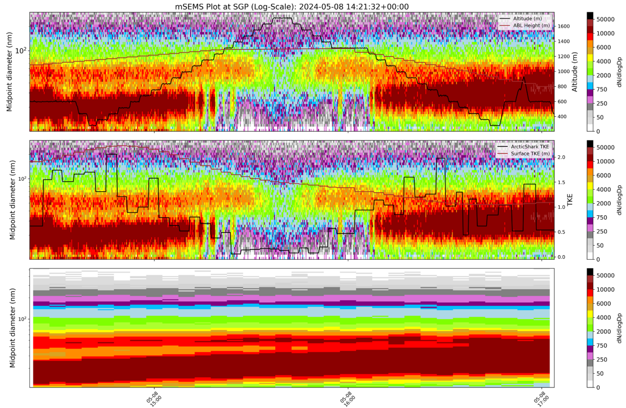
Figure 2. 2a presents the altitude of the ArcticShark (black line) and the estimated atmospheric boundary-layer (ABL) height (brown line) over the SGP field site overlaid onto an aerosol size distribution from the miniaturized scanning electrical mobility sizer (mSEMS) aboard the ArcticShark. 2b displays the same aerosol size distribution plot in Figure 1a, but overlaid by a time series of total kinetic energy (TKE) aboard the ArcticShark (black line) and at the surface of the SGP field site (brown line). 2c is an aerosol size distribution from the scanning mobility particle sizer (SMPS) at the surface of the SGP field site.
