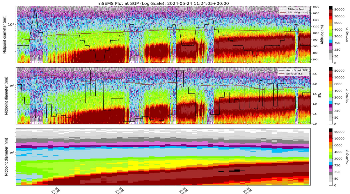
Figure 3. 3a presents the altitude of the ArcticShark (black-line) and the estimated ABL height (brown line) over the SGP field site overlaid onto an aerosol size distribution from the mSEMS aboard the ArcticShark. 3b displays the same aerosol size distribution plot in Figure 2a, but overlaid by a time series of TKE aboard the ArcticShark (black line) and at the surface of the SGP field site (brown line). 3c is an aerosol size distribution from the SMPS at the surface of the SGP field site.
