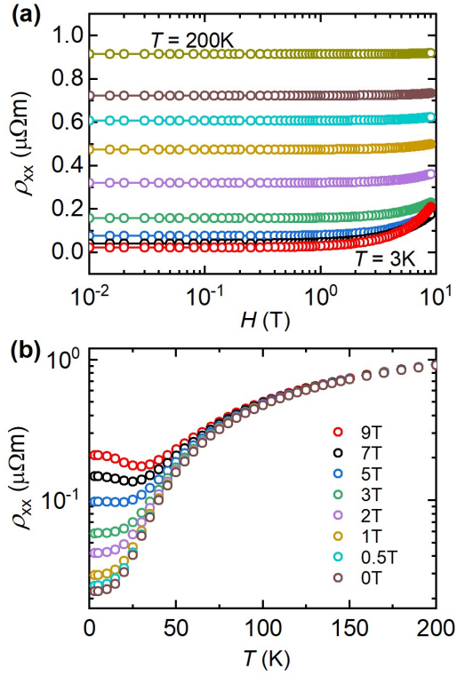
Fig. 2. (a) Magnetic field dependence of the longitudinal resistivity, \rho_{xx}(H) , at T = 3 K, 25 K, 35 K, 50 K, 75 K, 100 K, 125 K, 150 K, and 200 K (from bottom to top). (b) Temperature dependence of the longitudinal resistivity, \rho_{xx}(T) , at various magnetic fields as denoted by the legend.
