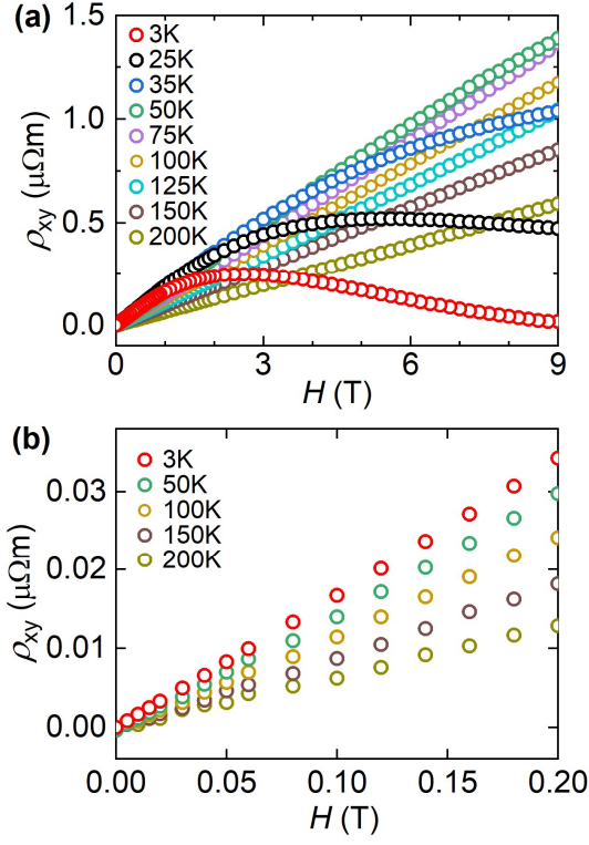
Fig. 6. (a) Magnetic field dependence of the Hall resistivity, \rho_{xy}(H) , at various temperatures. (b) Expanded view of \rho_{xy}(H) in (a) at magnetic fields up to H = 0.2 T. For clarity, only data at T = 3 K, 50 K, 100 K, 150 K and 200 K are presented. The linearity of \rho_{xy}(H) allow us to derive the Hall carrier density n_H = H/(e\rho_{xy}) .
