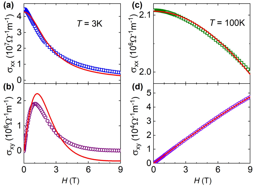
Fig. 5. (a) and (b) two-band model fittings of the longitudinal and Hall magnetoconductivities \sigma_{xx} and \sigma_{xy} for T = 3\text{ K} , respectively. (c) and (d) the same analysis as those in (a) and (b) but for T = 100\text{ K} . Symbols are experimental data and lines are fittings with Eq.(2) and Eq.(3). The derived densities are presented in Fig.4(b).
