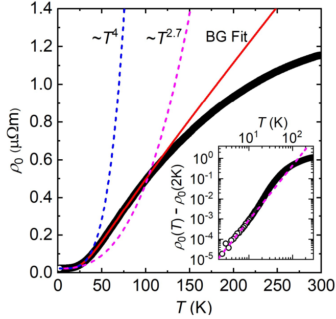
Fig.1. Zero-field cooling curve of the exfoliated sample. Symbols are experimental data. Dashed blue line, dashed magenta line and the red solid line present the fits of \rho_0 \sim T^4 , \rho_0 \sim T^{2.7} and Bloch-Gruneisen function Eq.1, respectively. The inset shows a logarithmic plot of the temperature dependence of the resistivity after subtracting the residual value \rho_0(2\text{K}) = 2.244 \mu\Omega\text{cm} at T = 2 \text{ K} . The dashed magenta line represents \rho_0 \sim T^{2.7} .
