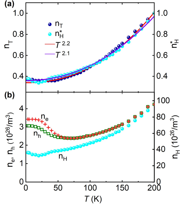
Fig. 4. (a) Temperature dependence of the thermal factor n_T and the normalized Hall carrier density n_H^* = n_H(T)/n_H(200\text{K}) . The red and violet lines represent power-law fittings of n_T \sim T^{2.2} and n_H^* \sim T^{2.1} , respectively. (b) Temperature dependence of the Hall carrier density n_H and the electron and hole densities n_e and n_h derived from two-band model analysis.
