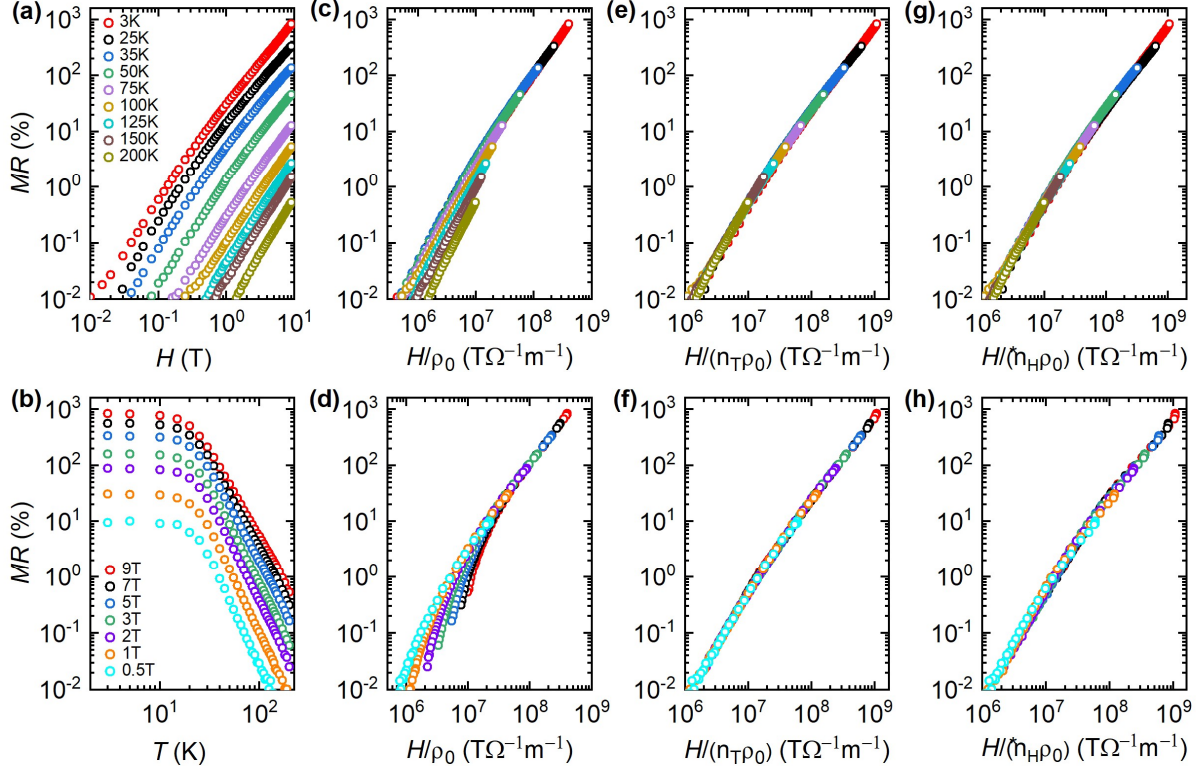
Fig. 3. (a) and (b) Magnetic field and temperature dependences of the MR derived from data in Figs. 2(a) and 2(b), respectively. (c) and (d) Kohler's rule plots of the data in (a) and (b), respectively. (e) and (f) Extended Kohler's rule plots of the MR curves in (a) and (b), respectively. The used n_T values are presented in Fig.4(a), where n_T = 1 at T = 200 K. (g) and (h) Extended Kohler's rule plots of the MR curves in (a) and (b) by replacing n_T with n_H^* , where n_H^* = n_H(T)/n_H(200K) is the normalized Hall carrier density, i.e., n_H^* = 1 at T = 200 K, for direct comparisons with the results in (e) and (f), where n_H(T) is the Hall carrier density obtained from the Hall resistivity at low magnetic fields, as elaborated in Fig.6 and its caption. n_H^* and n_H data are presented in Fig.4(a) and 4(b) respectively.
