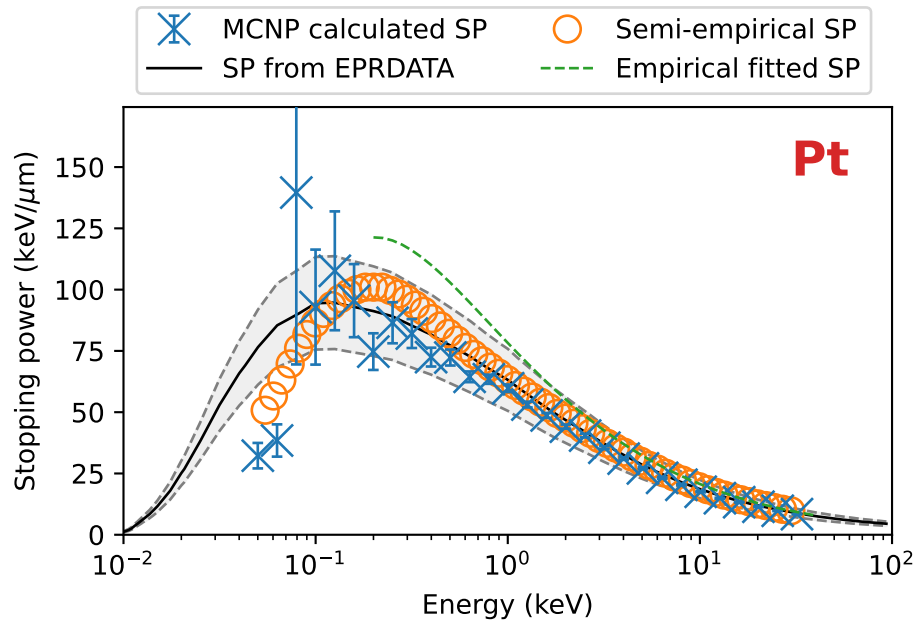
Figure 111: Stopping power results and benchmarks for platinum.
