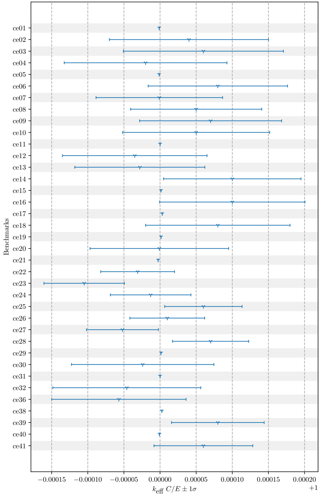
Figure 137: Analytical k_{\text{eff}} C/E Continuous Energy Benchmark Results
