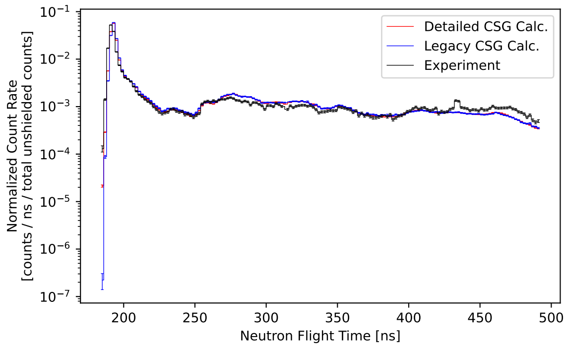
Figure 16: Comparison of the measured and calculated (ENDF/B-VI.6) normalized count rate of neutrons escaping from a 2.0 MFP (14-MeV neutron) thick sphere of concrete plotted against flight time.
