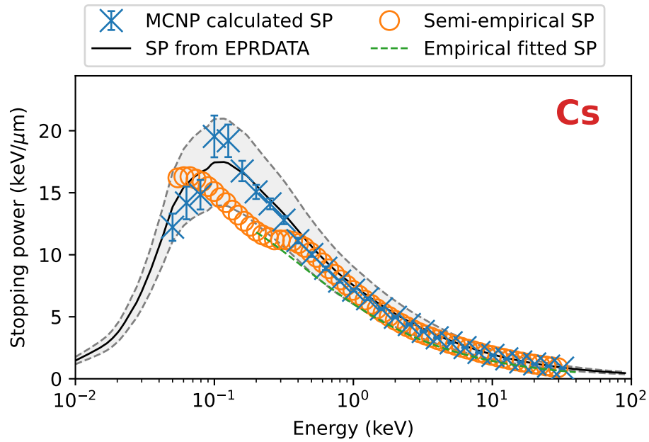
Figure 101: Stopping power results and benchmarks for cesium.
