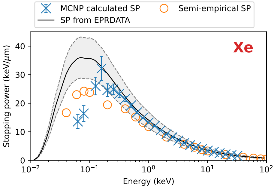
Figure 136: Stopping power results and benchmarks for solid xenon.
