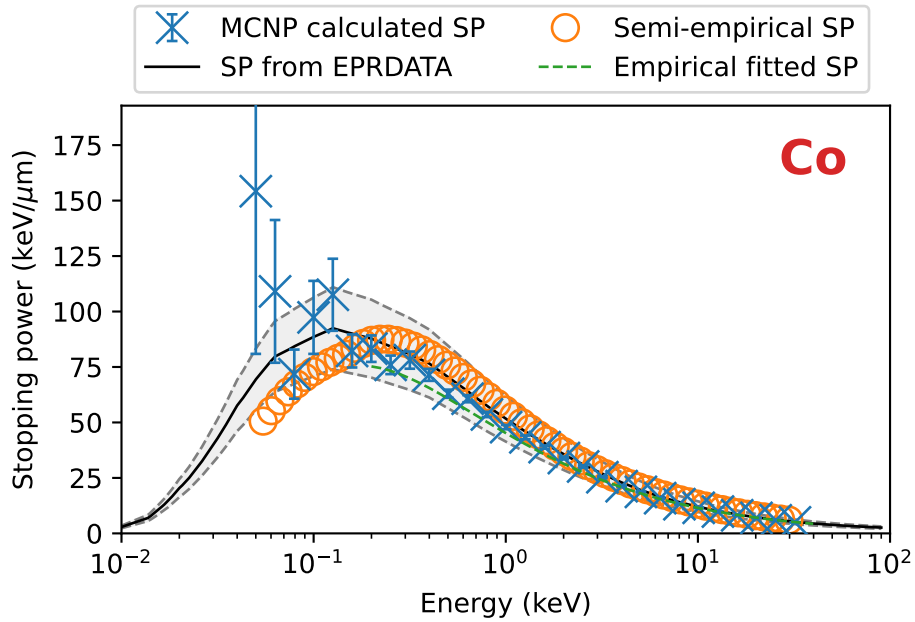
Figure 88: Stopping power results and benchmarks for cobalt.
