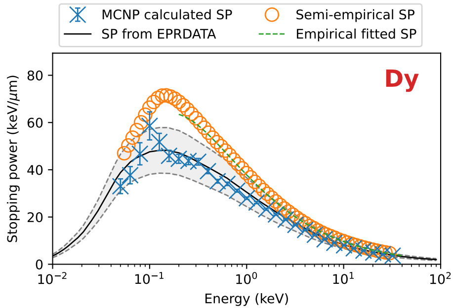
Figure 104: Stopping power results and benchmarks for dysprosium.
