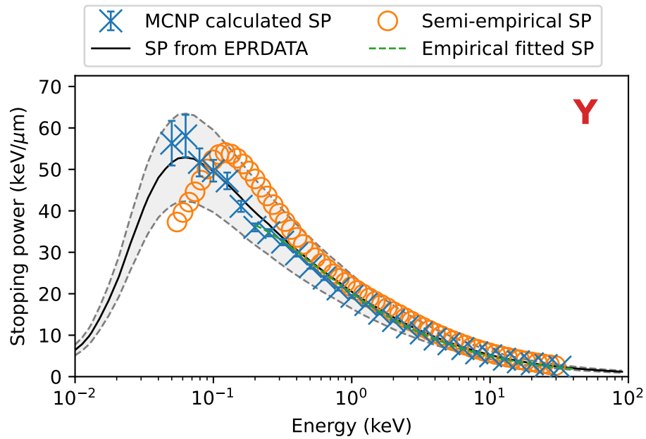
Figure 92: Stopping power results and benchmarks for yttrium.
