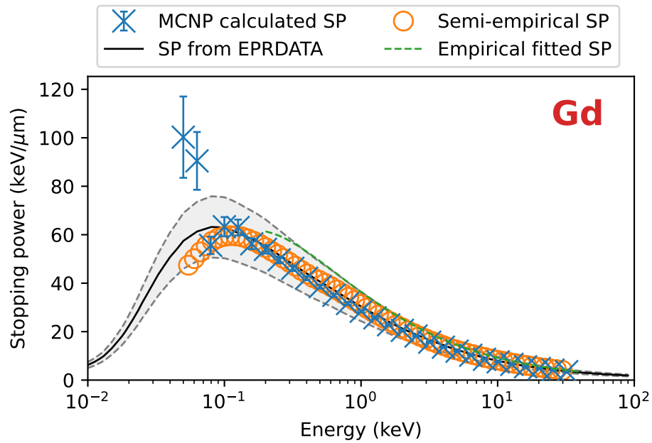
Figure 102: Stopping power results and benchmarks for gadolinium.
