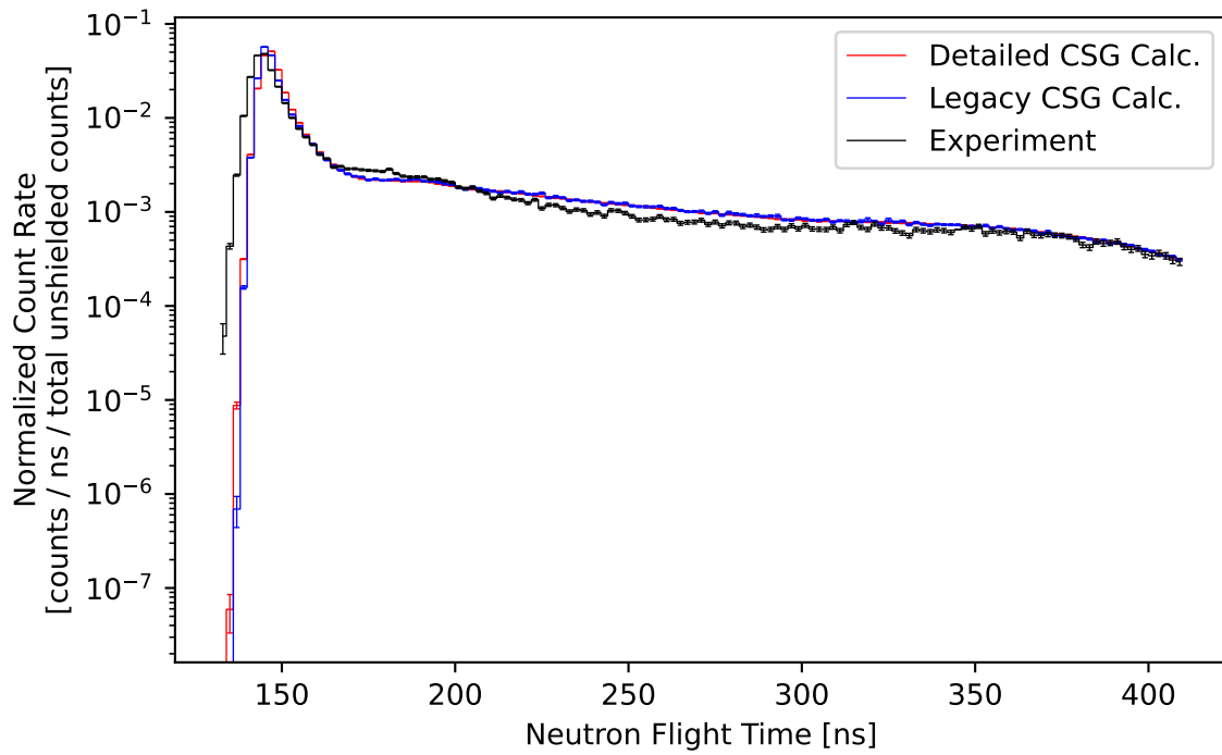
Figure 36: Comparison of the measured and calculated (ENDF/B-VIII.0) normalized count rate of neutrons escaping from a 1.6 MFP (14-MeV neutron) thick sphere of lithium-6 plotted against flight time.
