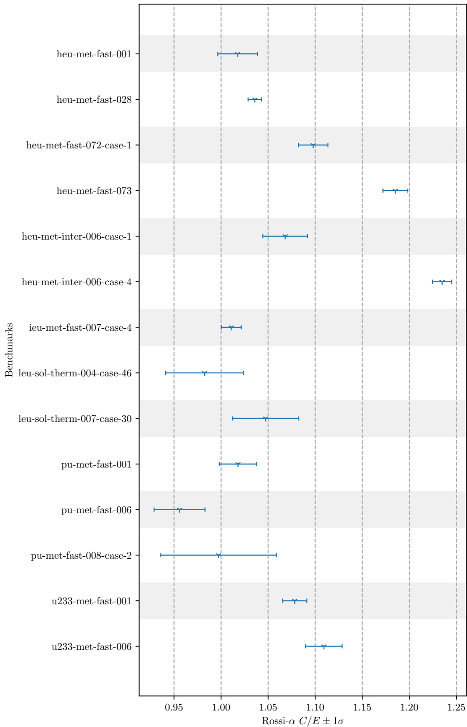
Figure 73: Rossi- \alpha C/E (ENDF/B-VII.0) Benchmark Results
