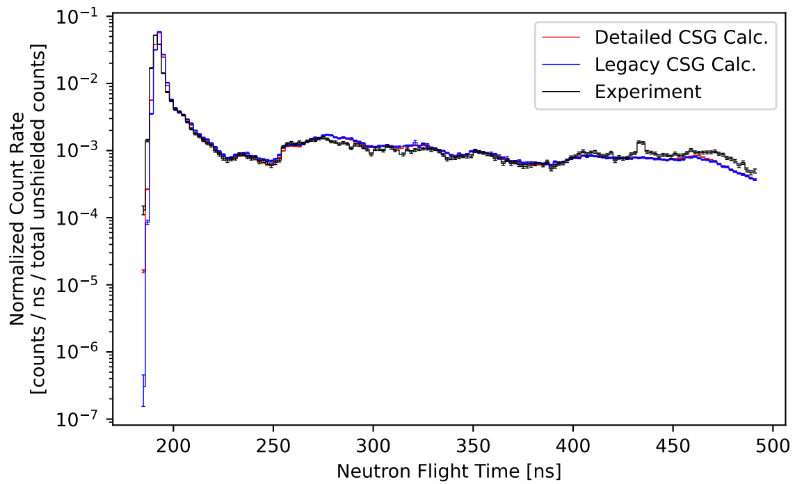
Figure 28: Comparison of the measured and calculated (ENDF/B-VII.1) normalized count rate of neutrons escaping from a 2.0 MFP (14-MeV neutron) thick sphere of concrete plotted against flight time.
