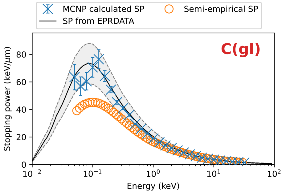
Figure 116: Stopping power results and benchmarks for glassy carbon.
