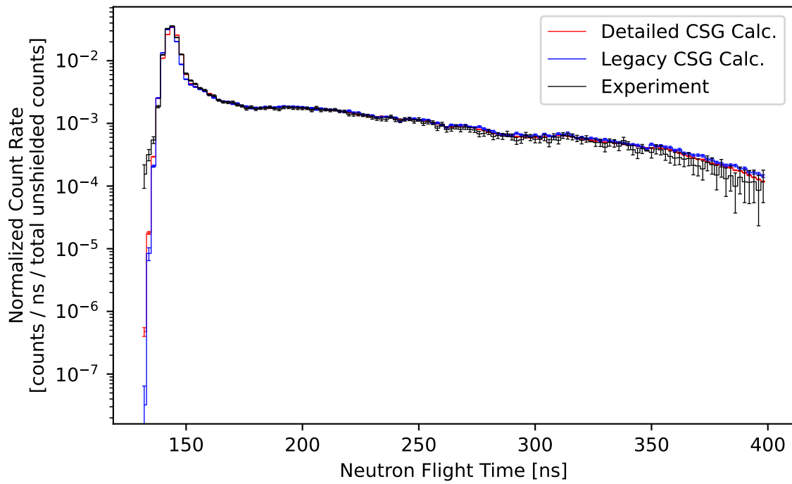
Figure 31: Comparison of the measured and calculated (ENDF/B-VII.1) normalized count rate of neutrons escaping from a 1.9 MFP (14-MeV neutron) thick sphere of water plotted against flight time.
