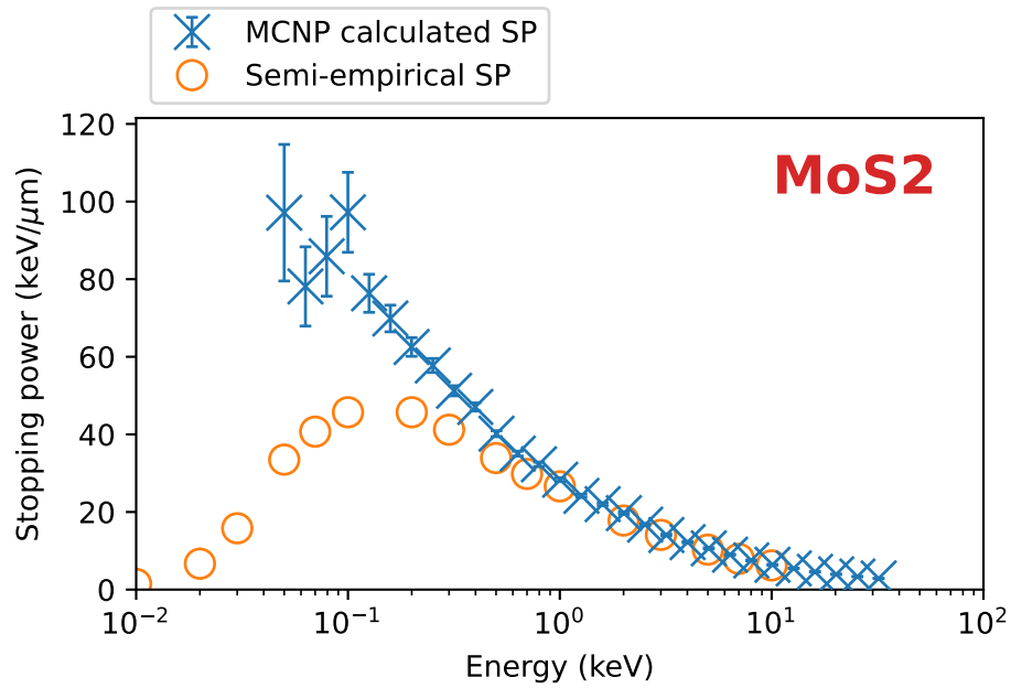
Figure 125: Stopping power results and benchmarks for molybdenum disulfide.
