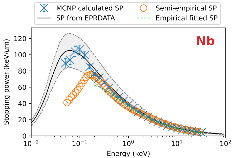
Figure 93: Stopping power results and benchmarks for niobium.
