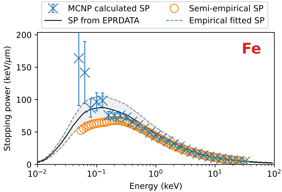
Figure 87: Stopping power results and benchmarks for iron.
