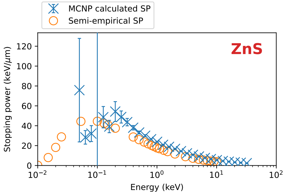
Figure 128: Stopping power results and benchmarks for zinc sulfide.
