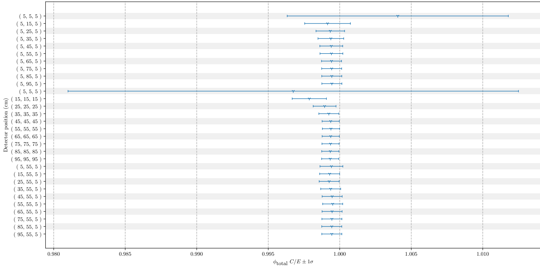
Figure 139: pli_ce C/E Calculation Benchmark Results
