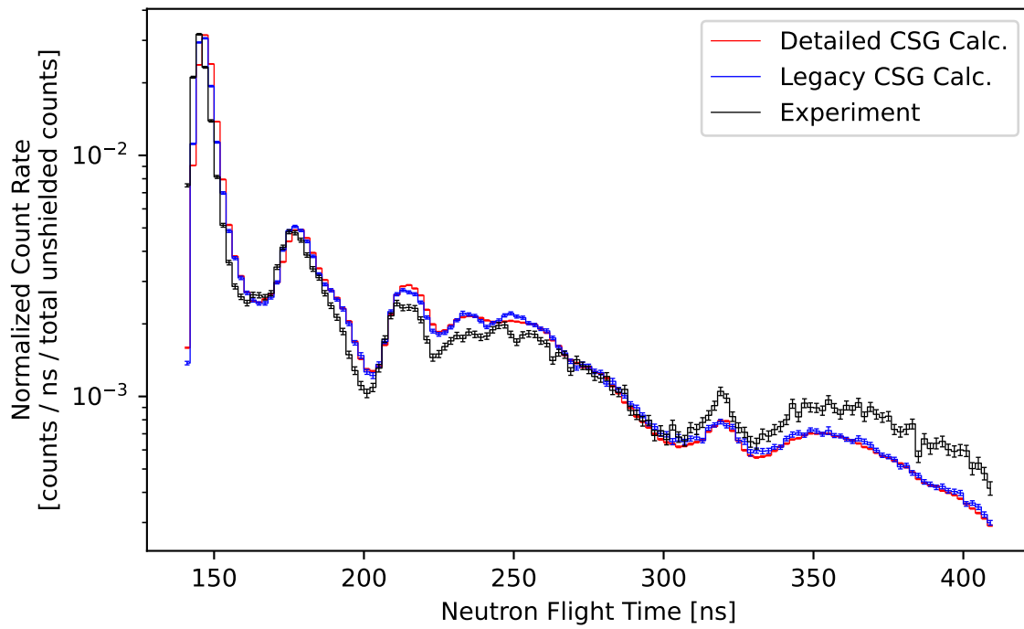
Figure 15: Comparison of the measured and calculated (ENDF/B-VI.6) normalized count rate of neutrons escaping from a 2.9 MFP (14-MeV neutron) thick sphere of carbon plotted against flight time.
