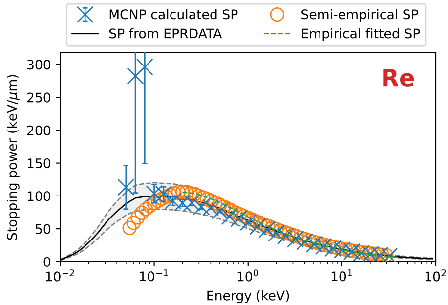
Figure 108: Stopping power results and benchmarks for rhenium.
