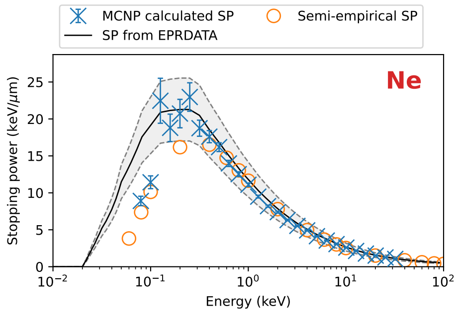
Figure 133: Stopping power results and benchmarks for solid neon.
