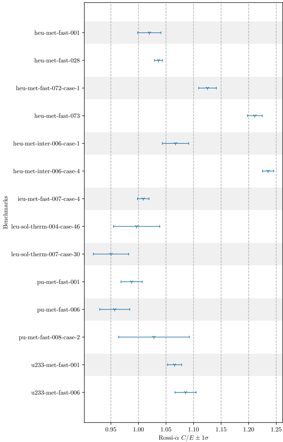
Figure 74: Rossi- \alpha C/E (ENDF/B-VII.1) Benchmark Results
