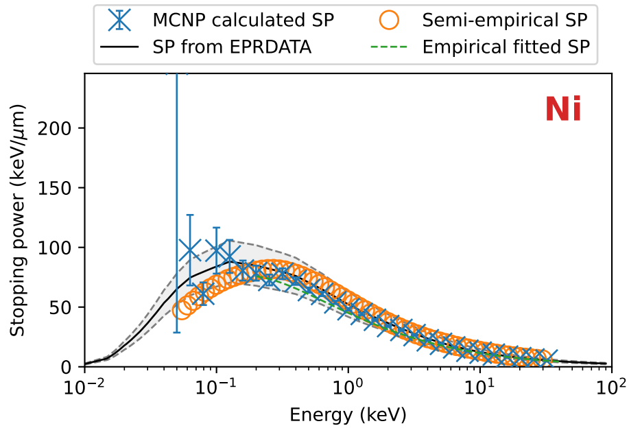
Figure 89: Stopping power results and benchmarks for nickel.
