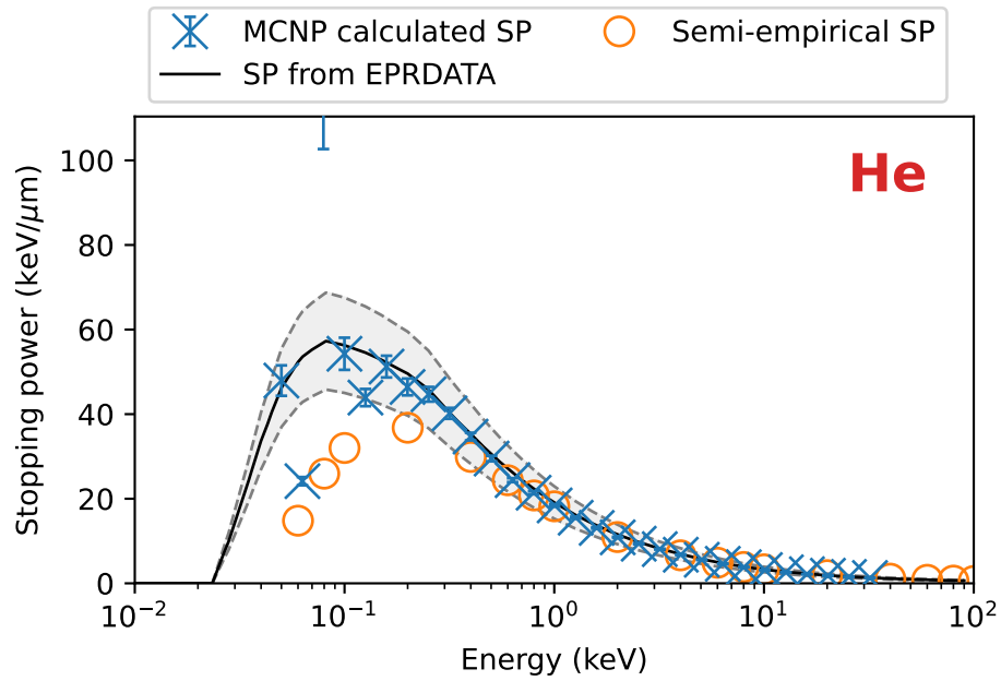
Figure 132: Stopping power results and benchmarks for solid helium.
