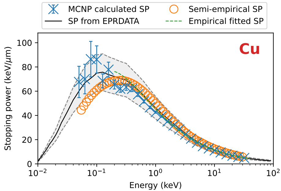
Figure 90: Stopping power results and benchmarks for copper.
