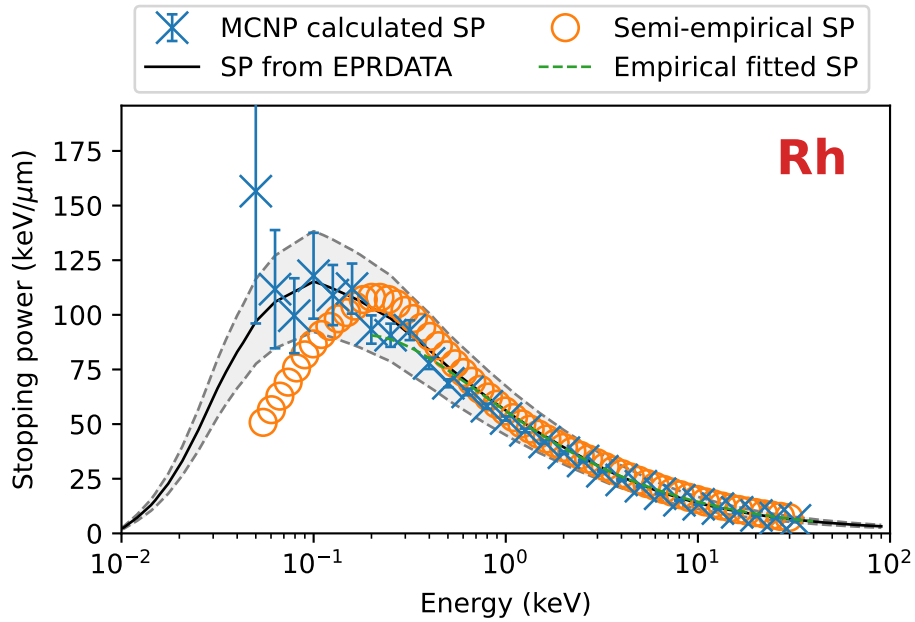
Figure 96: Stopping power results and benchmarks for rhodium.
