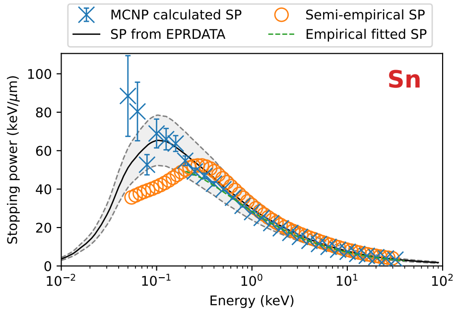
Figure 100: Stopping power results and benchmarks for tin.
