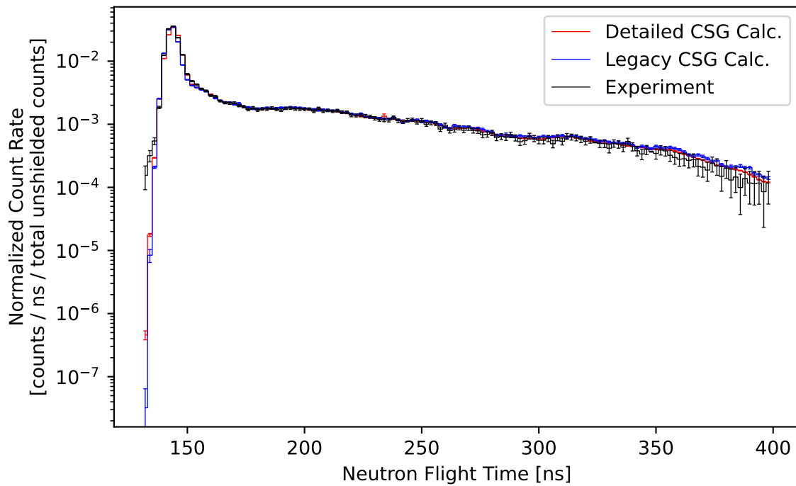
Figure 37: Comparison of the measured and calculated (ENDF/B-VIII.0) normalized count rate of neutrons escaping from a 1.9 MFP (14-MeV neutron) thick sphere of water plotted against flight time.
