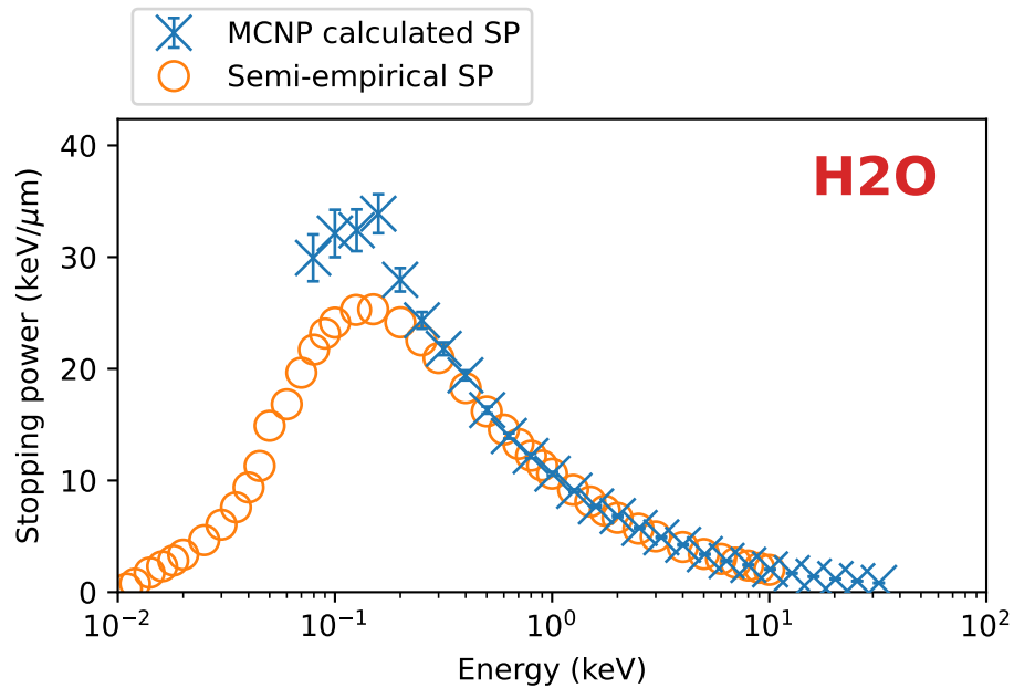
Figure 122: Stopping power results and benchmarks for vitreous ice.
