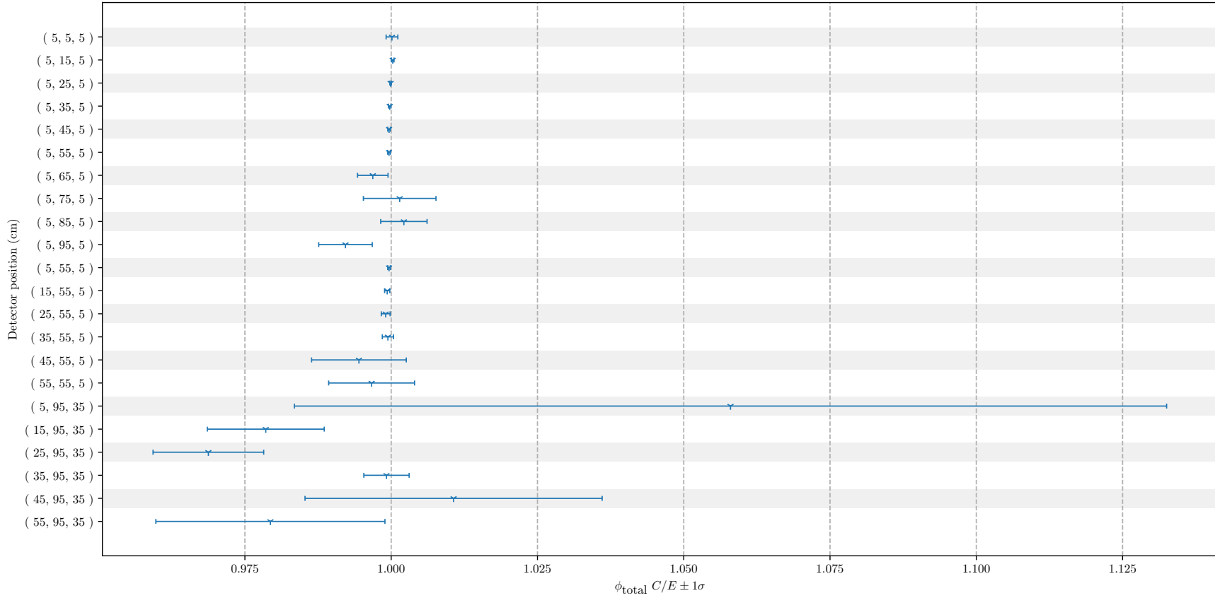
Figure 144: p3ii_ce C/E Calculation Benchmark Results
