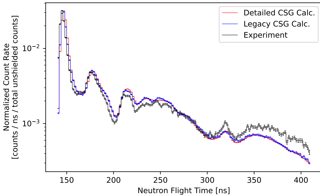
Figure 21: Comparison of the measured and calculated (ENDF/B-VII.0) normalized count rate of neutrons escaping from a 2.9 MFP (14-MeV neutron) thick sphere of carbon plotted against flight time.
