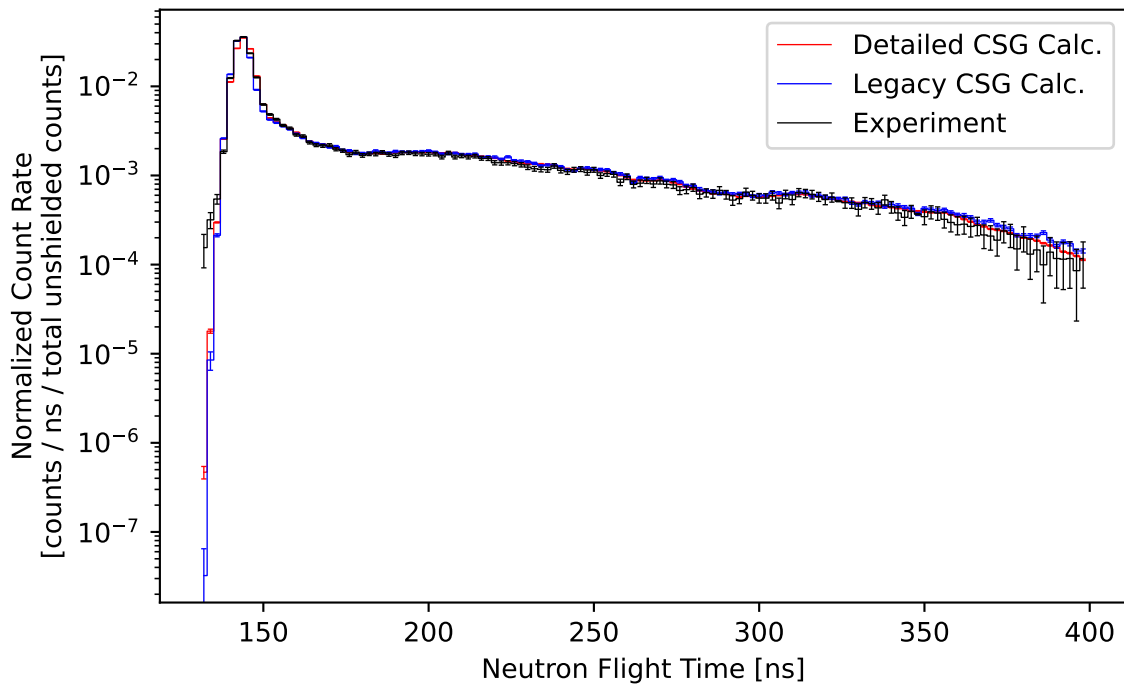
Figure 19: Comparison of the measured and calculated (ENDF/B-VI.6) normalized count rate of neutrons escaping from a 1.9 MFP (14-MeV neutron) thick sphere of water plotted against flight time.
