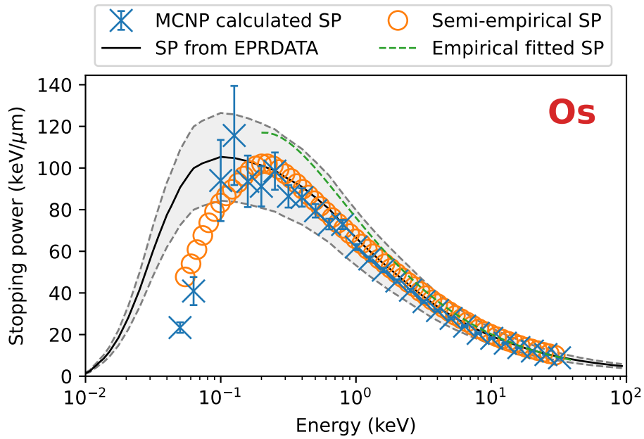
Figure 109: Stopping power results and benchmarks for osmium.
