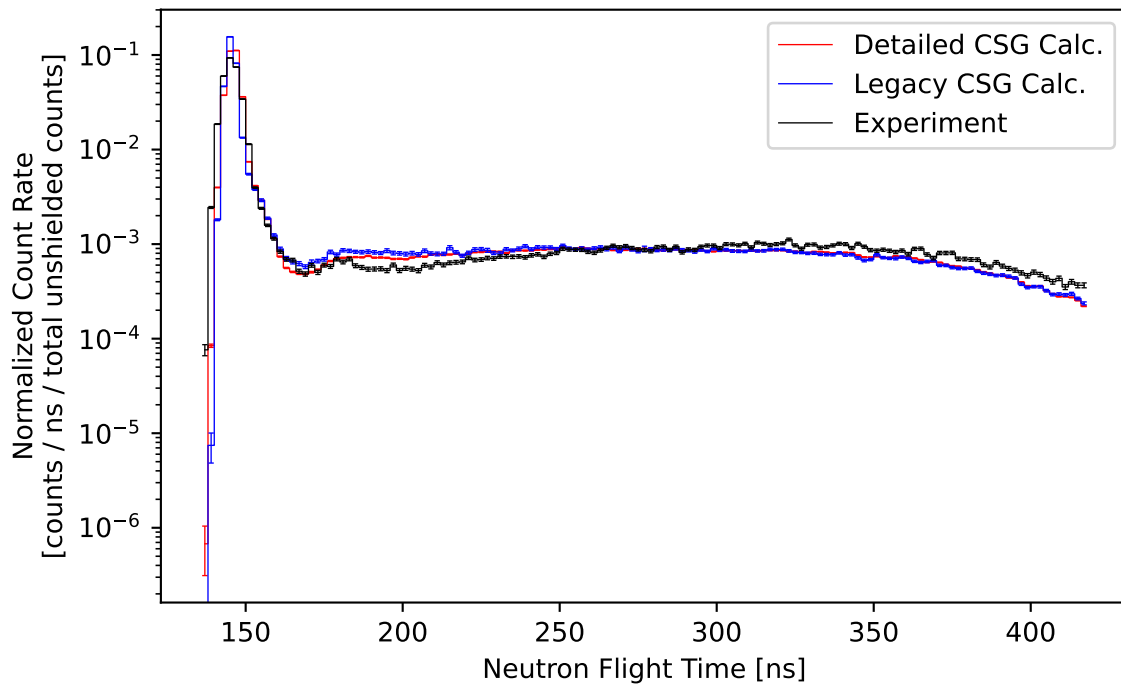
Figure 23: Comparison of the measured and calculated (ENDF/B-VII.0) normalized count rate of neutrons escaping from a 0.9 MFP (14-MeV neutron) thick sphere of iron plotted against flight time.
