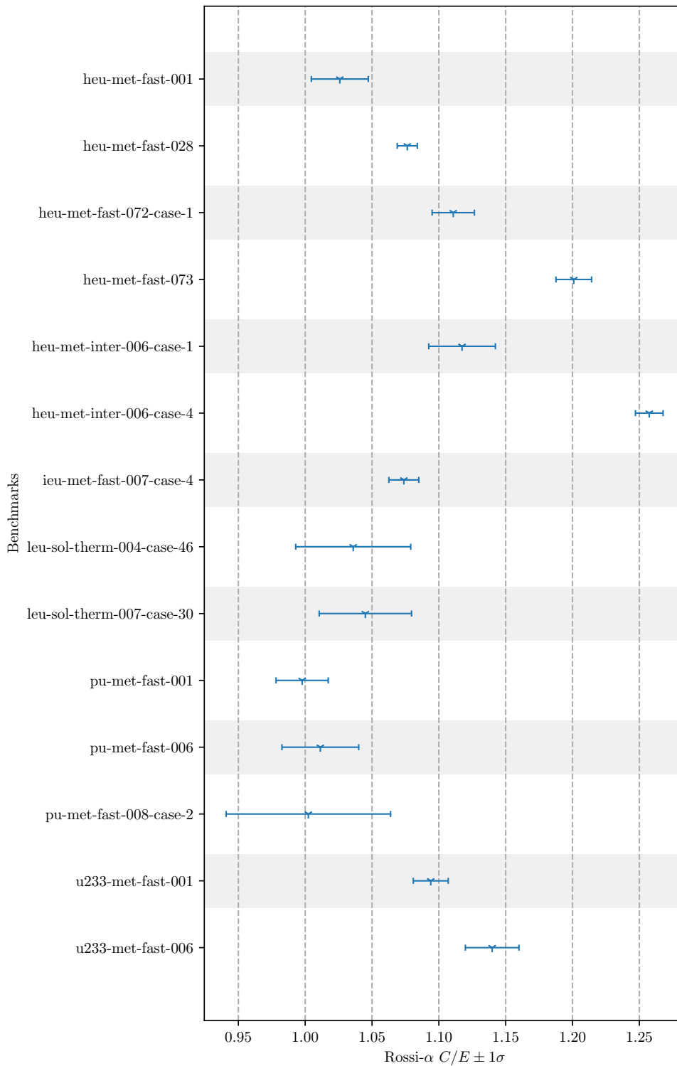
Figure 72: Rossi- \alpha C/E (ENDF/B-VI.6) Benchmark Results
