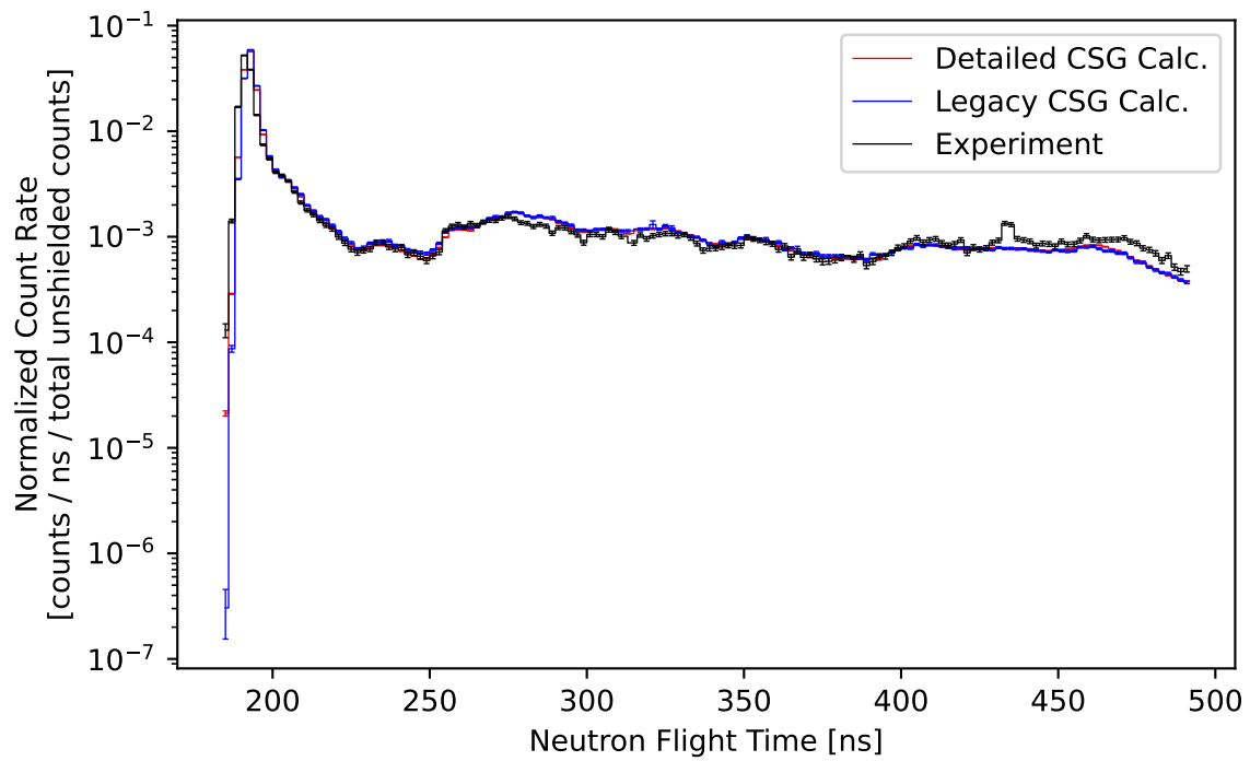
Figure 22: Comparison of the measured and calculated (ENDF/B-VII.0) normalized count rate of neutrons escaping from a 2.0 MFP (14-MeV neutron) thick sphere of concrete plotted against flight time.
