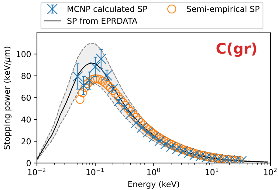
Figure 117: Stopping power results and benchmarks for graphite.
