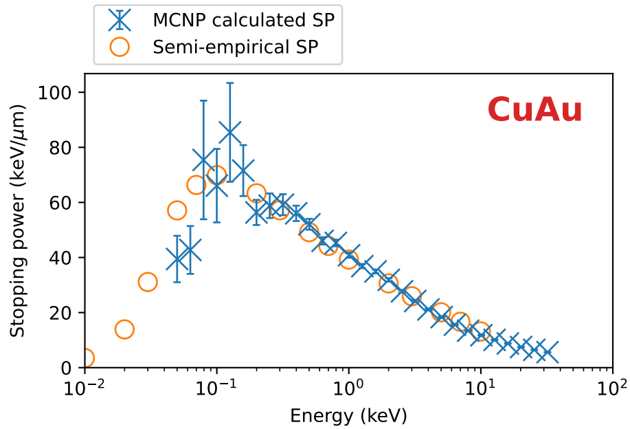
Figure 119: Stopping power results and benchmarks for rose gold.
