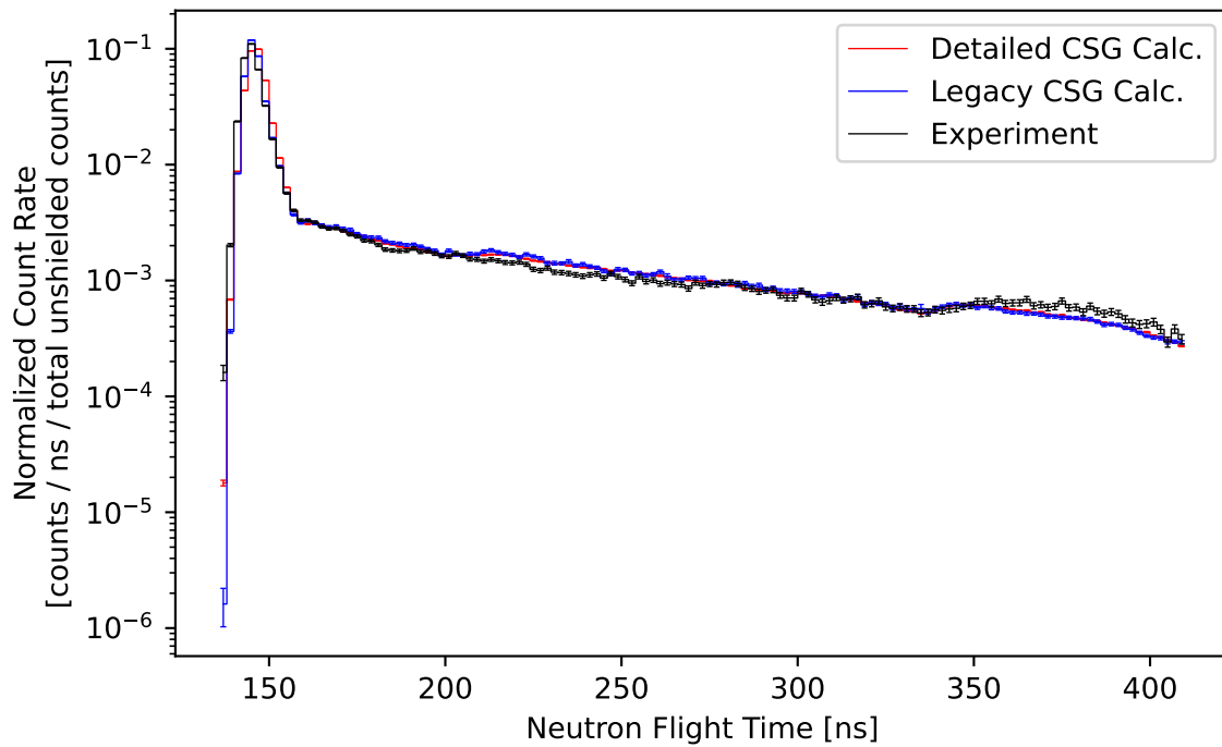
Figure 26: Comparison of the measured and calculated (ENDF/B-VII.1) normalized count rate of neutrons escaping from a 0.8 MFP (14-MeV neutron) thick sphere of beryllium plotted against flight time.
