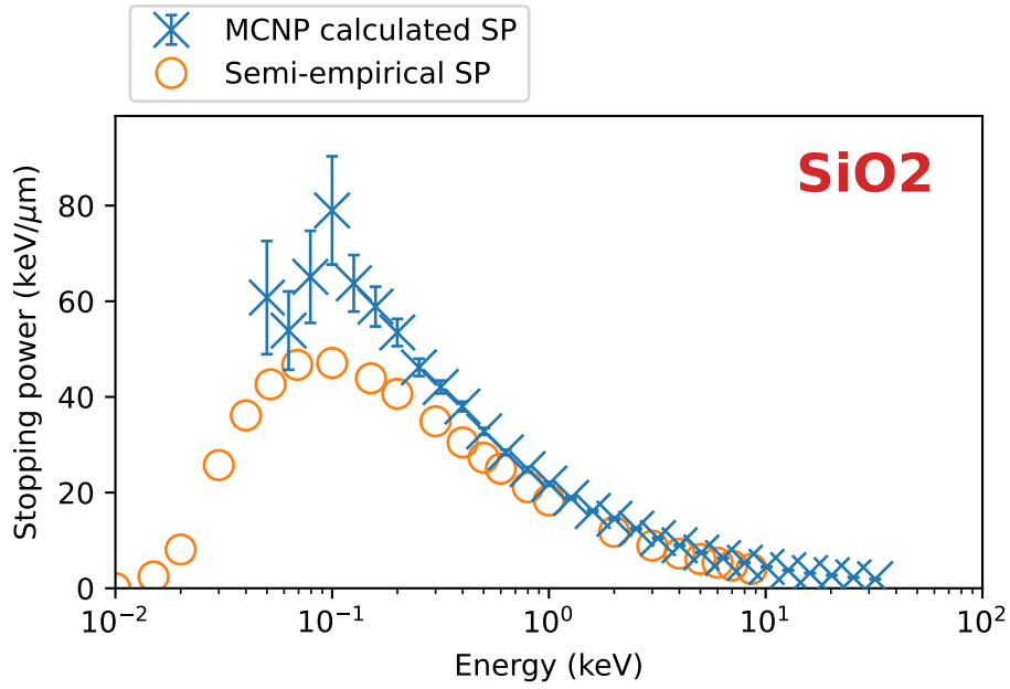
Figure 127: Stopping power results and benchmarks for quartz.
