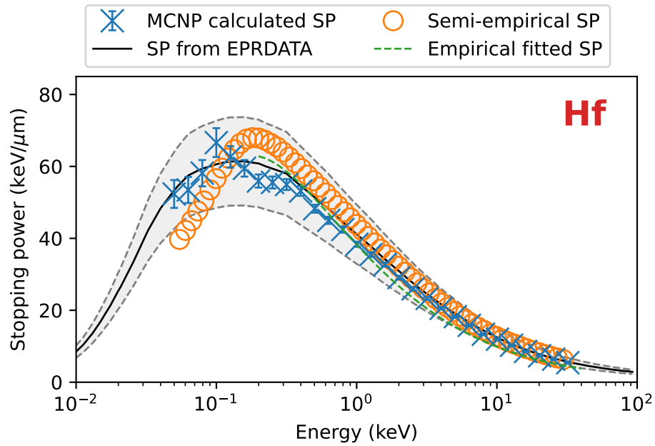
Figure 105: Stopping power results and benchmarks for hafnium.
