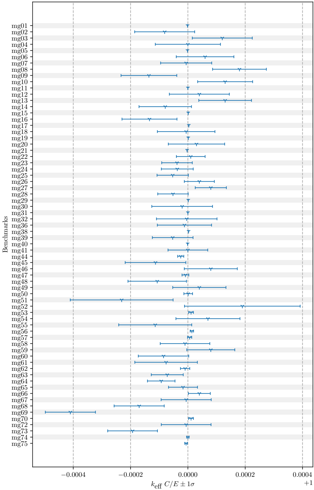
Figure 138: Analytical k_{\text{eff}} C/E Multigroup Benchmark Results
