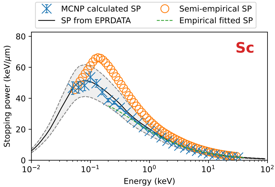
Figure 83: Stopping power results and benchmarks for scandium.
