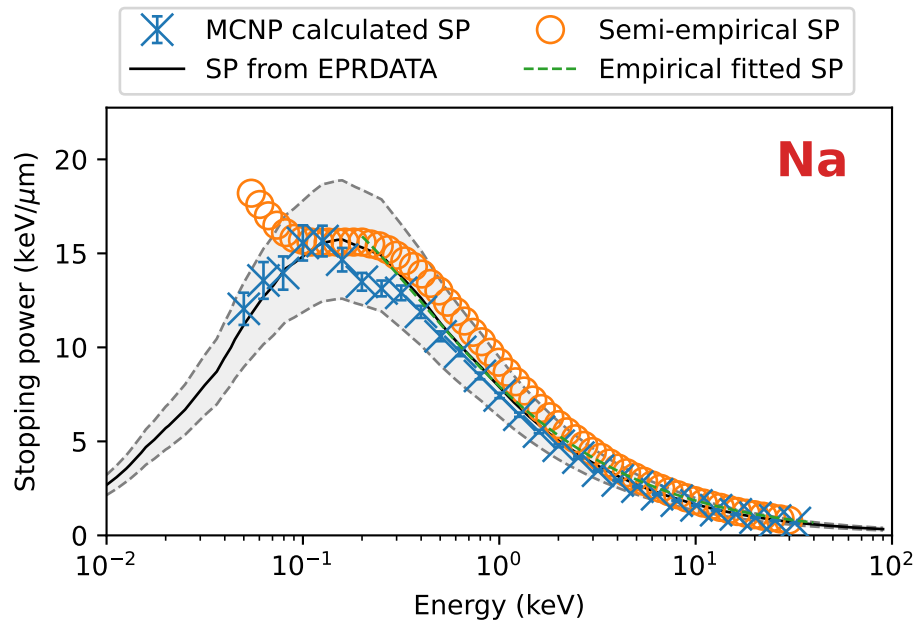
Figure 78: Stopping power results and benchmarks for sodium.
