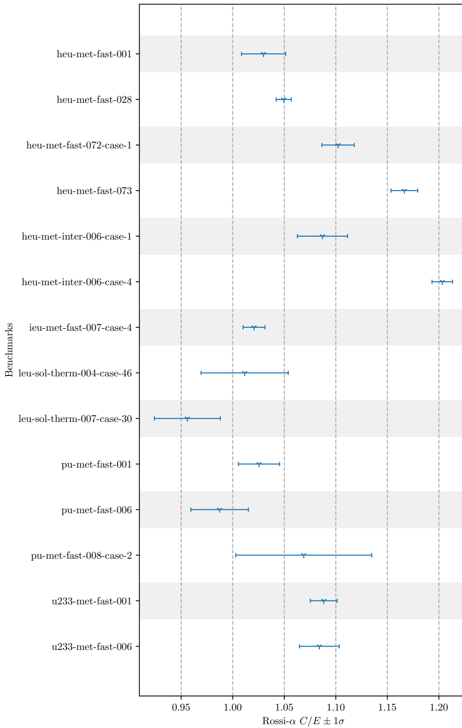
Figure 75: Rossi- \alpha C/E (ENDF/B-VIII.0) Benchmark Results
