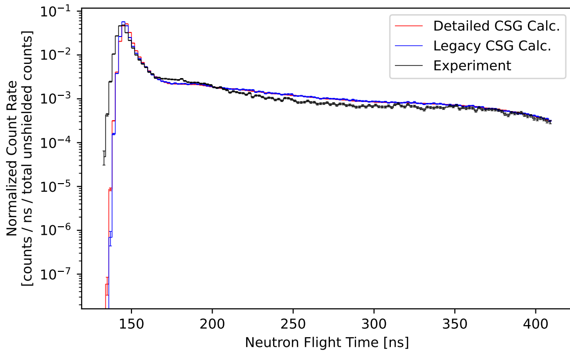
Figure 24: Comparison of the measured and calculated (ENDF/B-VII.0) normalized count rate of neutrons escaping from a 1.6 MFP (14-MeV neutron) thick sphere of lithium-6 plotted against flight time.
