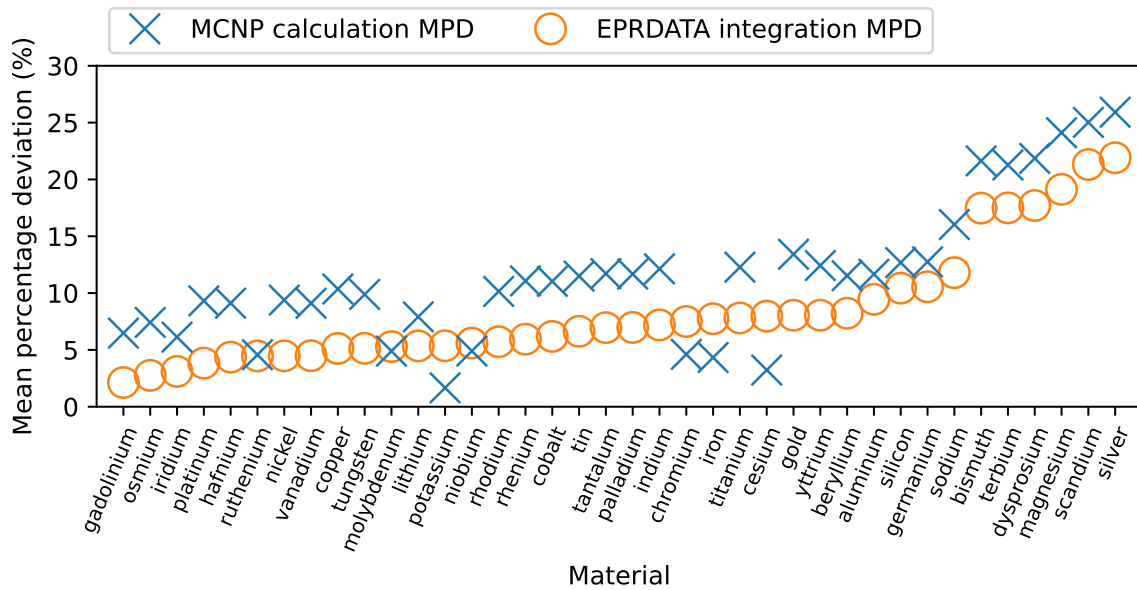
Figure 114: Mean percentage deviation (MPD) for simulated (with MCNP) and integrated (from EPRDATA) electron stopping powers in elemental solids.
