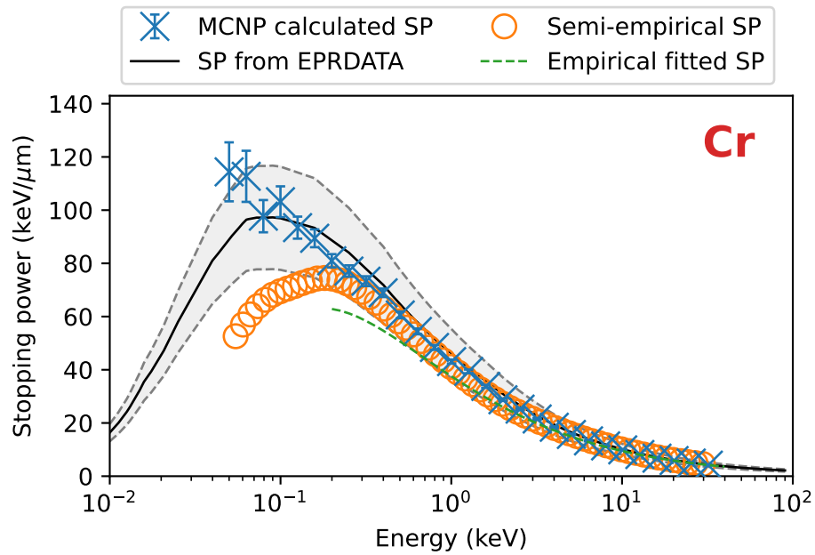
Figure 86: Stopping power results and benchmarks for chromium.
