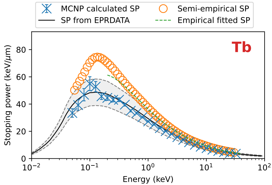
Figure 103: Stopping power results and benchmarks for terbium.
