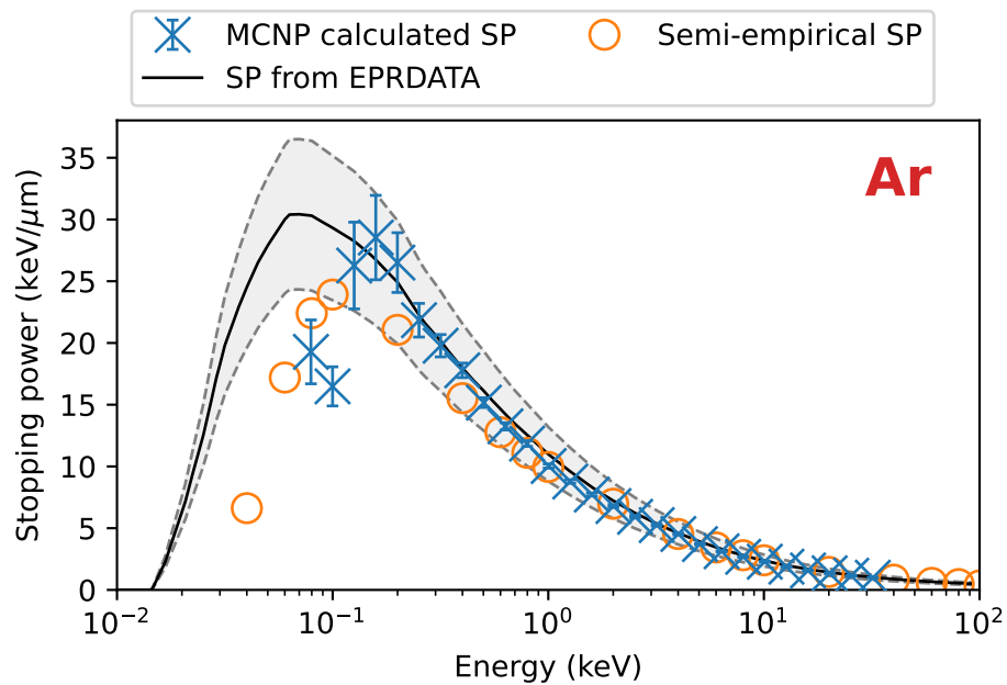
Figure 134: Stopping power results and benchmarks for solid argon.
