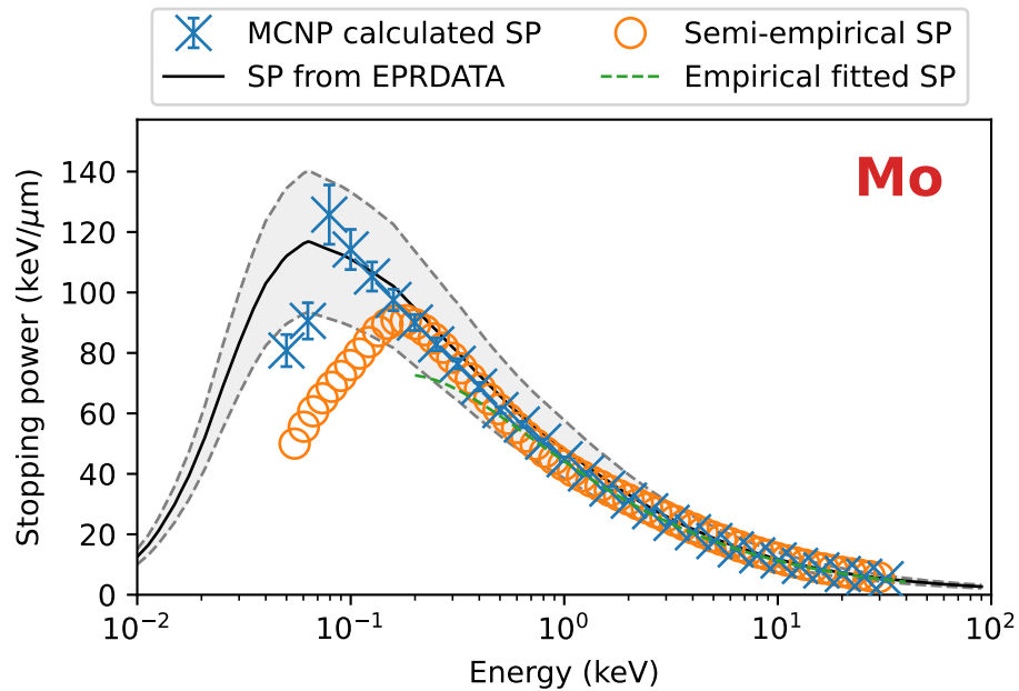
Figure 94: Stopping power results and benchmarks for molybdenum.
