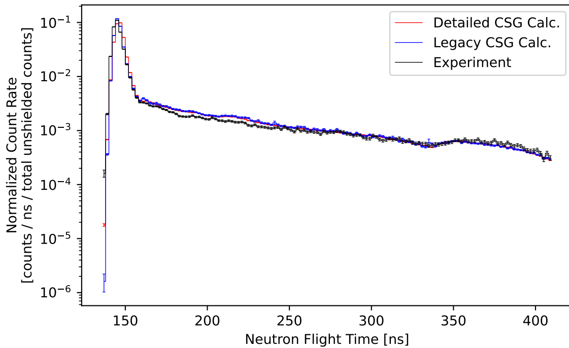
Figure 32: Comparison of the measured and calculated (ENDF/B-VIII.0) normalized count rate of neutrons escaping from a 0.8 MFP (14-MeV neutron) thick sphere of beryllium plotted against flight time.
