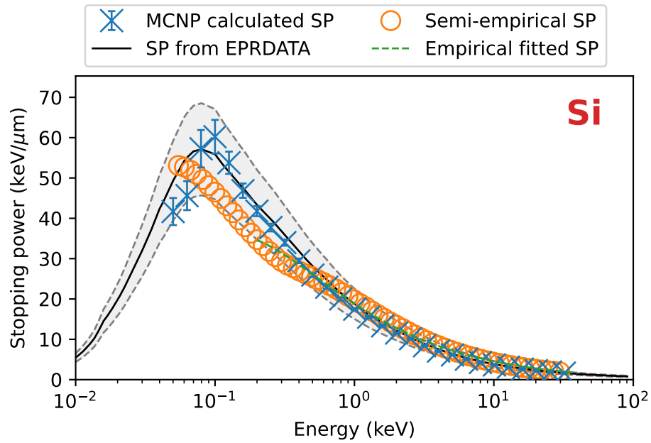
Figure 81: Stopping power results and benchmarks for silicon.
