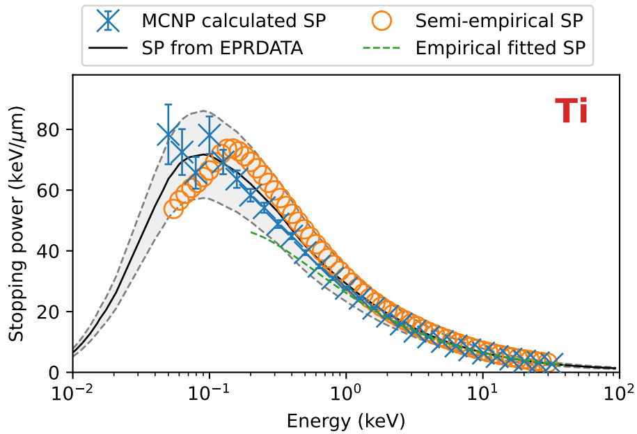
Figure 84: Stopping power results and benchmarks for titanium.
