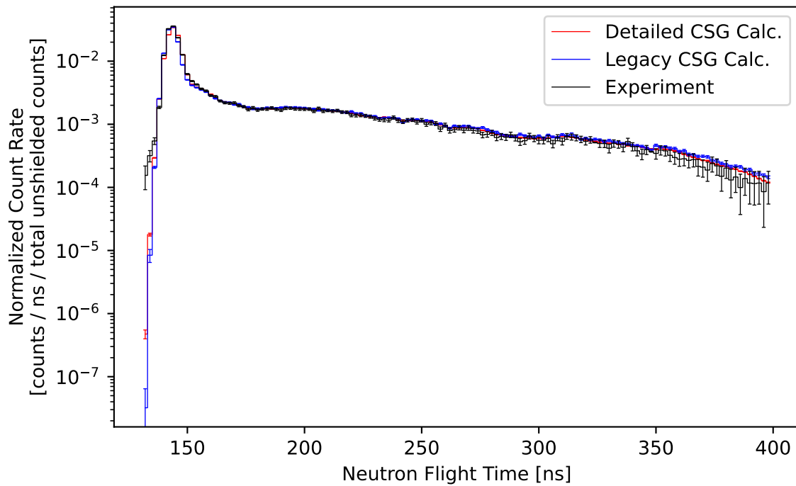
Figure 25: Comparison of the measured and calculated (ENDF/B-VII.0) normalized count rate of neutrons escaping from a 1.9 MFP (14-MeV neutron) thick sphere of water plotted against flight time.
