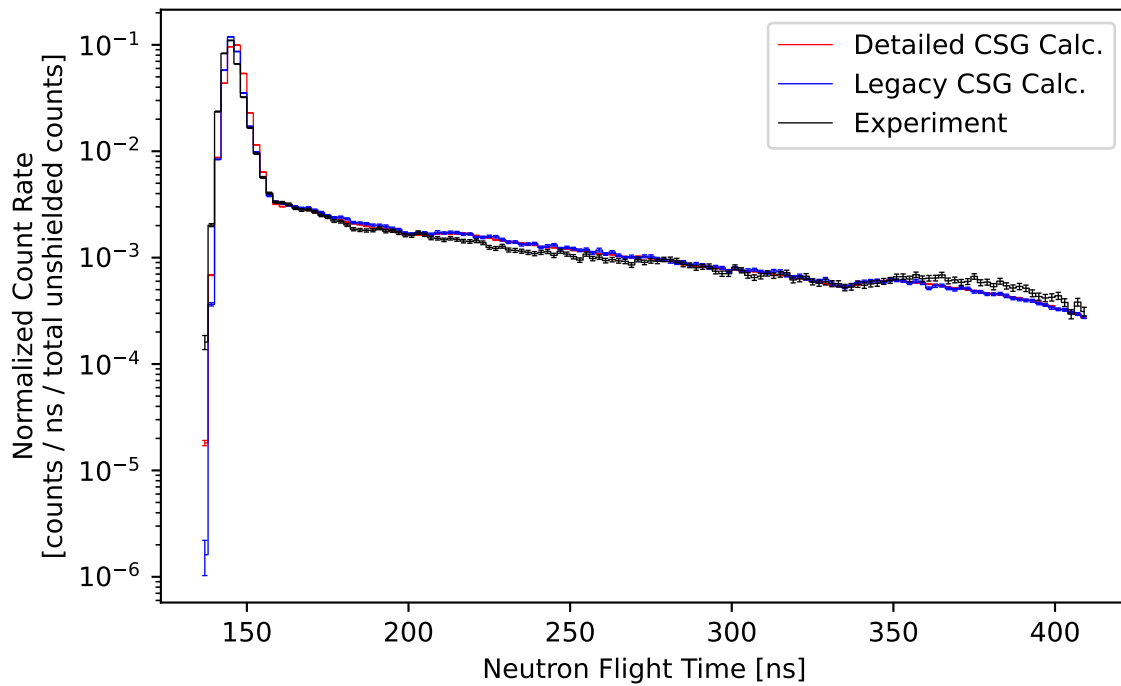
Figure 14: Comparison of the measured and calculated (ENDF/B-VI.6) normalized count rate of neutrons escaping from a 0.8 MFP (14-MeV neutron) thick sphere of beryllium plotted against flight time.
