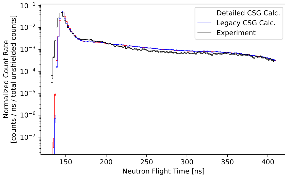
Figure 30: Comparison of the measured and calculated (ENDF/B-VII.1) normalized count rate of neutrons escaping from a 1.6 MFP (14-MeV neutron) thick sphere of lithium-6 plotted against flight time.
