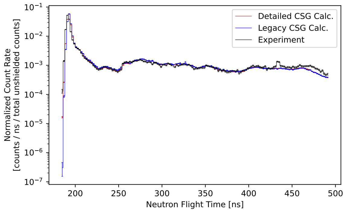
Figure 34: Comparison of the measured and calculated (ENDF/B-VIII.0) normalized count rate of neutrons escaping from a 2.0 MFP (14-MeV neutron) thick sphere of concrete plotted against flight time.
