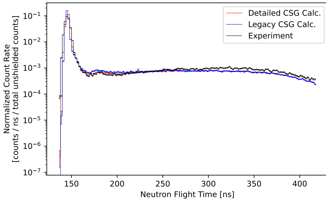
Figure 35: Comparison of the measured and calculated (ENDF/B-VIII.0) normalized count rate of neutrons escaping from a 0.9 MFP (14-MeV neutron) thick sphere of iron plotted against flight time.
