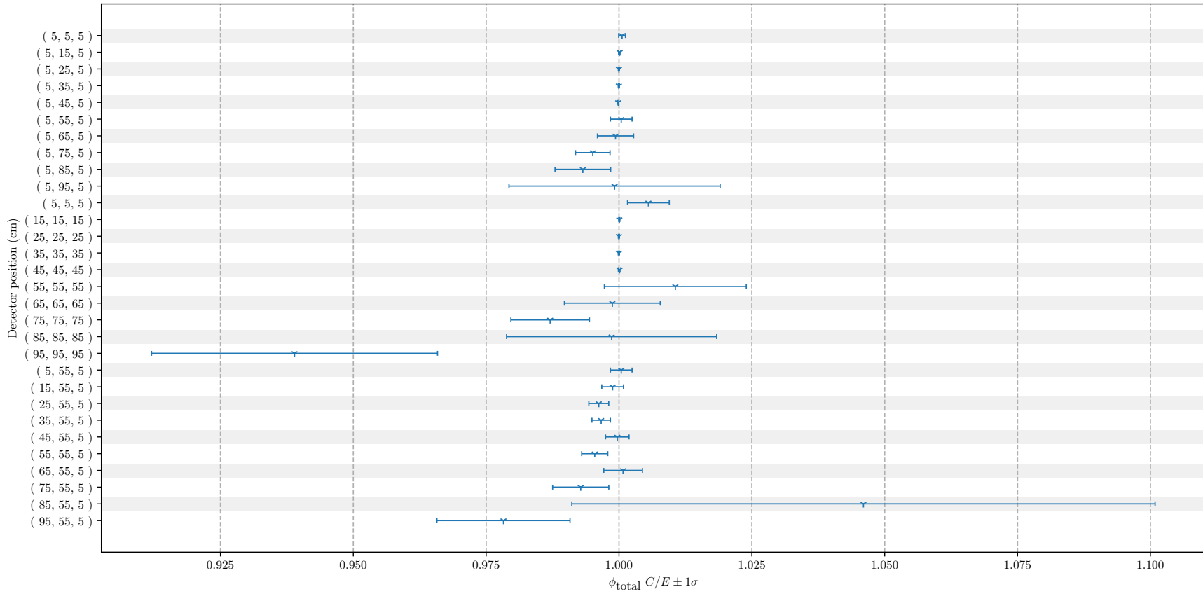
Figure 140: plii_ce C/E Calculation Benchmark Results
