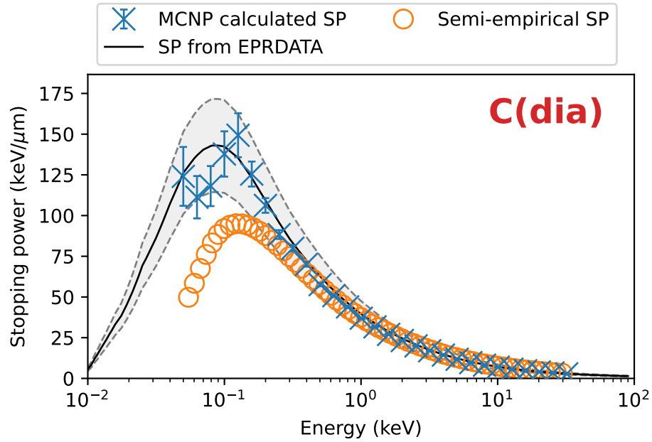
Figure 115: Stopping power results and benchmarks for diamond.
