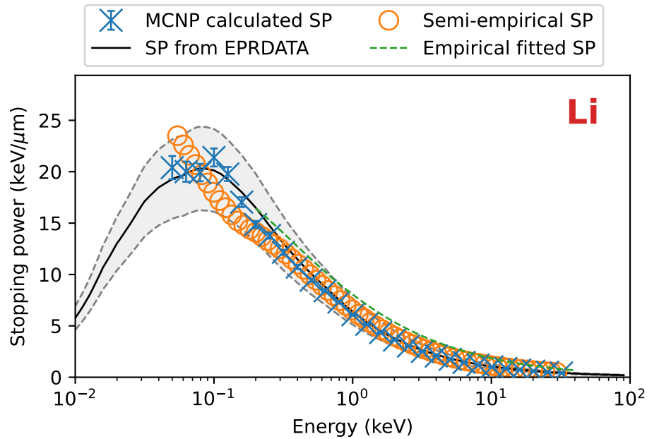
Figure 76: Stopping power results and benchmarks for lithium.
