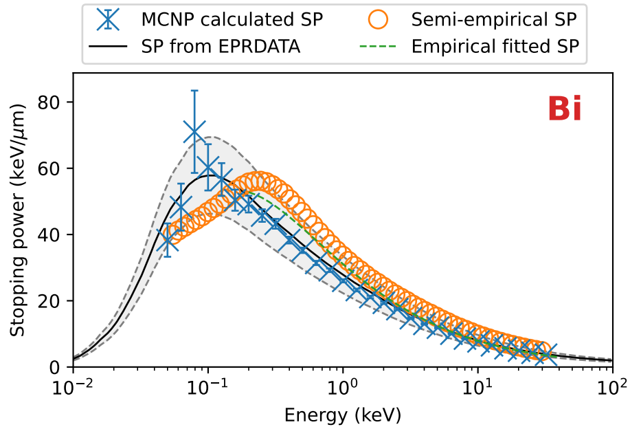
Figure 113: Stopping power results and benchmarks for bismuth.
