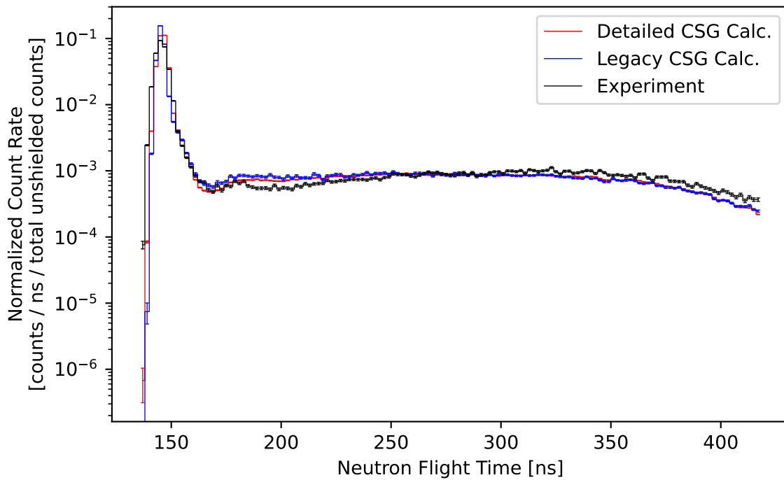
Figure 17: Comparison of the measured and calculated (ENDF/B-VI.6) normalized count rate of neutrons escaping from a 0.9 MFP (14-MeV neutron) thick sphere of iron plotted against flight time.
