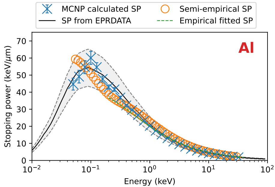
Figure 80: Stopping power results and benchmarks for aluminum.
