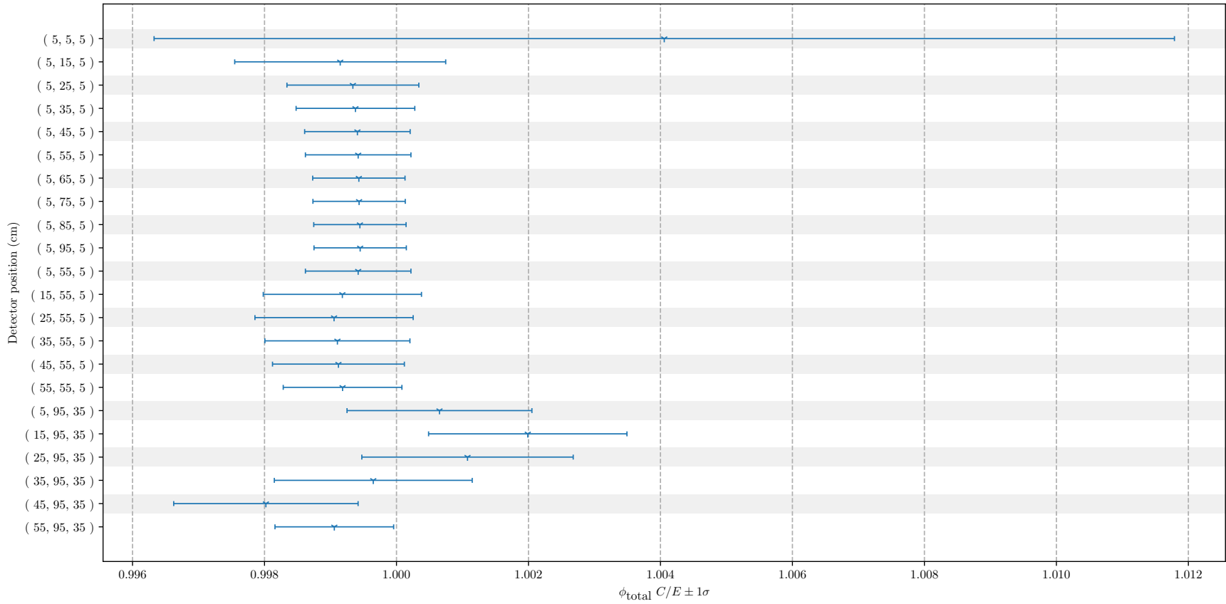
Figure 143: p3i_ce C/E Calculation Benchmark Results
