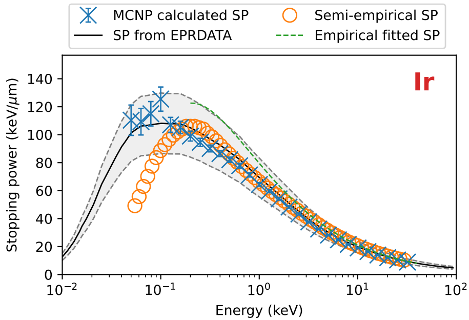
Figure 110: Stopping power results and benchmarks for iridium.
