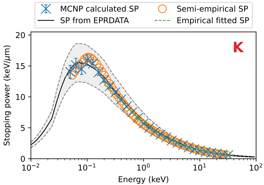
Figure 82: Stopping power results and benchmarks for potassium.
