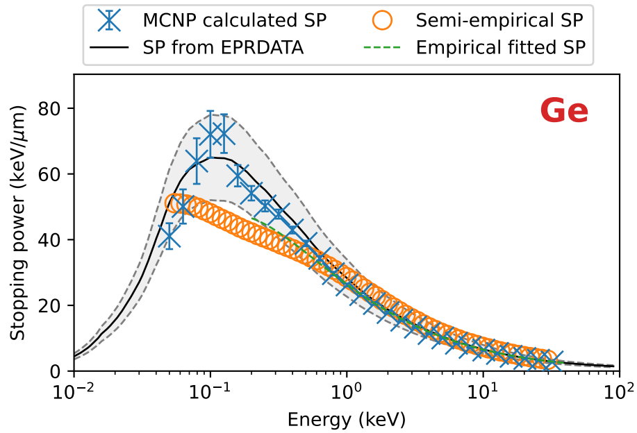
Figure 91: Stopping power results and benchmarks for germanium.
