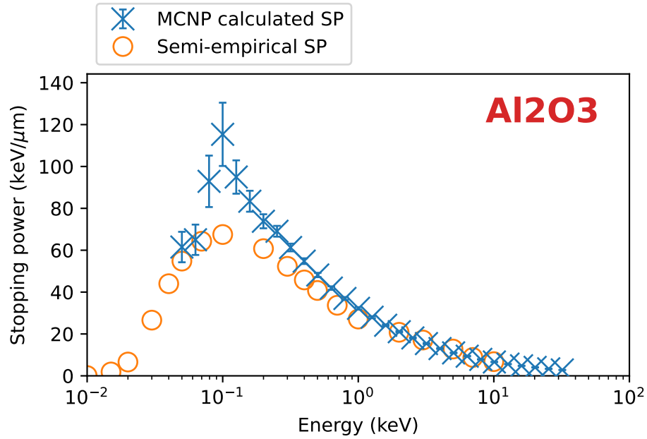
Figure 118: Stopping power results and benchmarks for sapphire.
