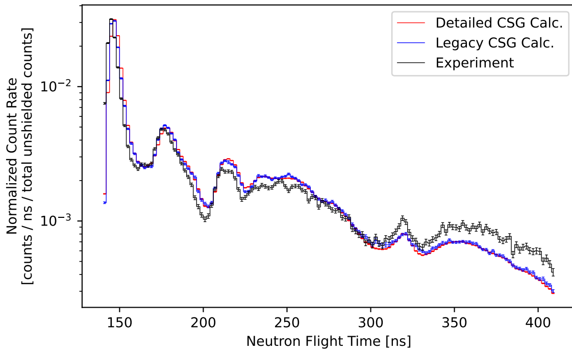
Figure 33: Comparison of the measured and calculated (ENDF/B-VIII.0) normalized count rate of neutrons escaping from a 2.9 MFP (14-MeV neutron) thick sphere of carbon plotted against flight time.
