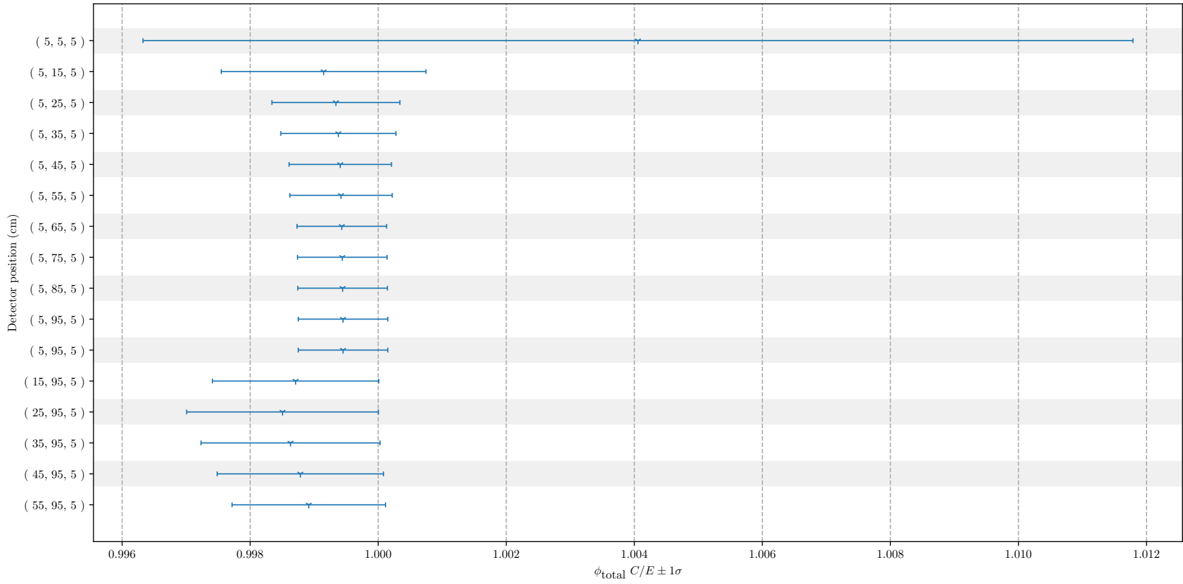
Figure 141: p2i_ce C/E Calculation Benchmark Results
