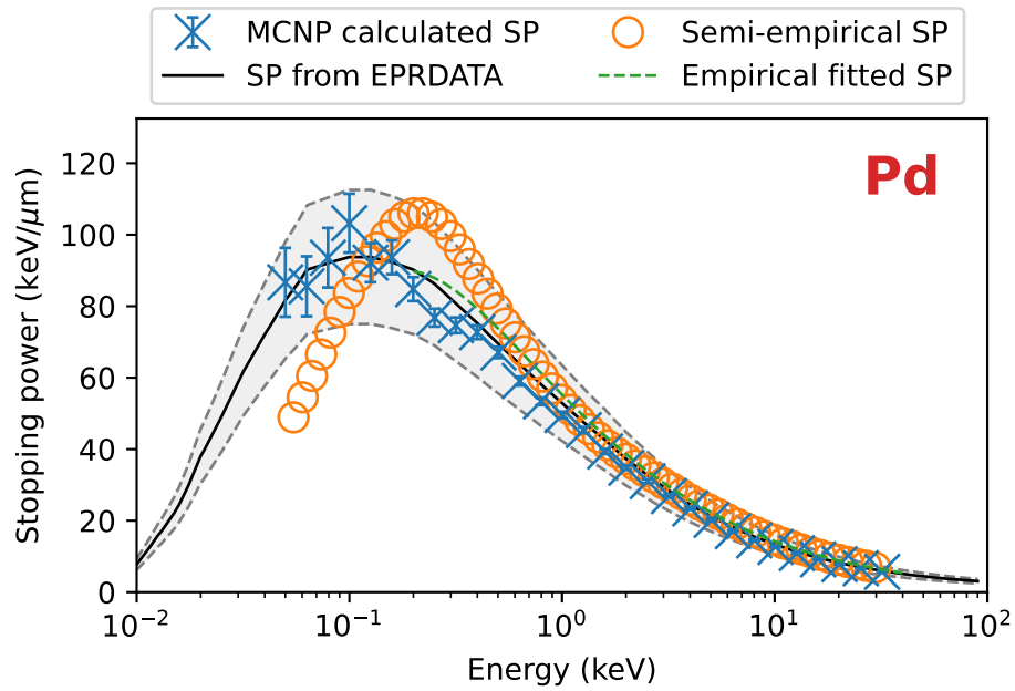
Figure 97: Stopping power results and benchmarks for palladium.
