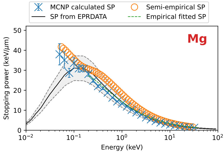
Figure 79: Stopping power results and benchmarks for magnesium.
