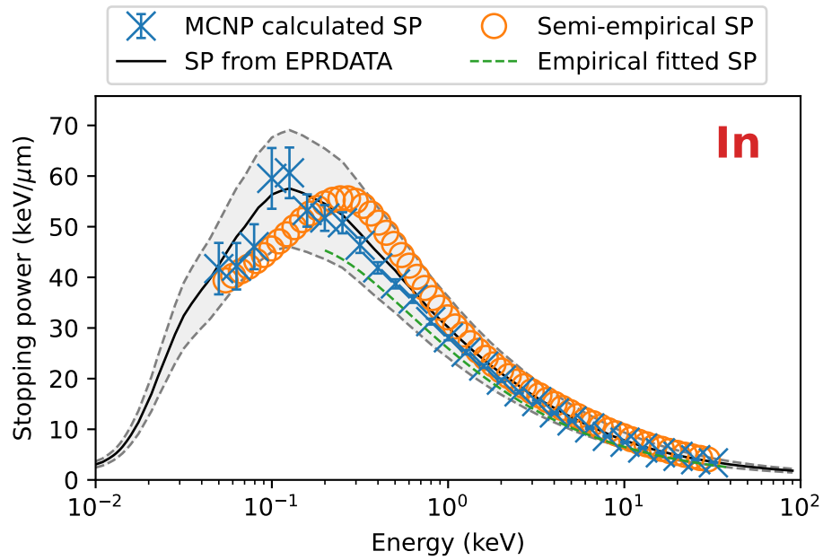
Figure 99: Stopping power results and benchmarks for indium.
