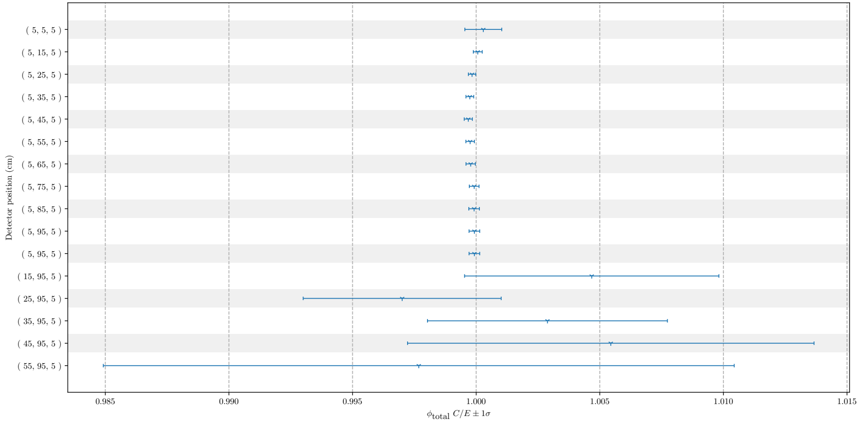
Figure 142: p2ii_ce C/E Calculation Benchmark Results
