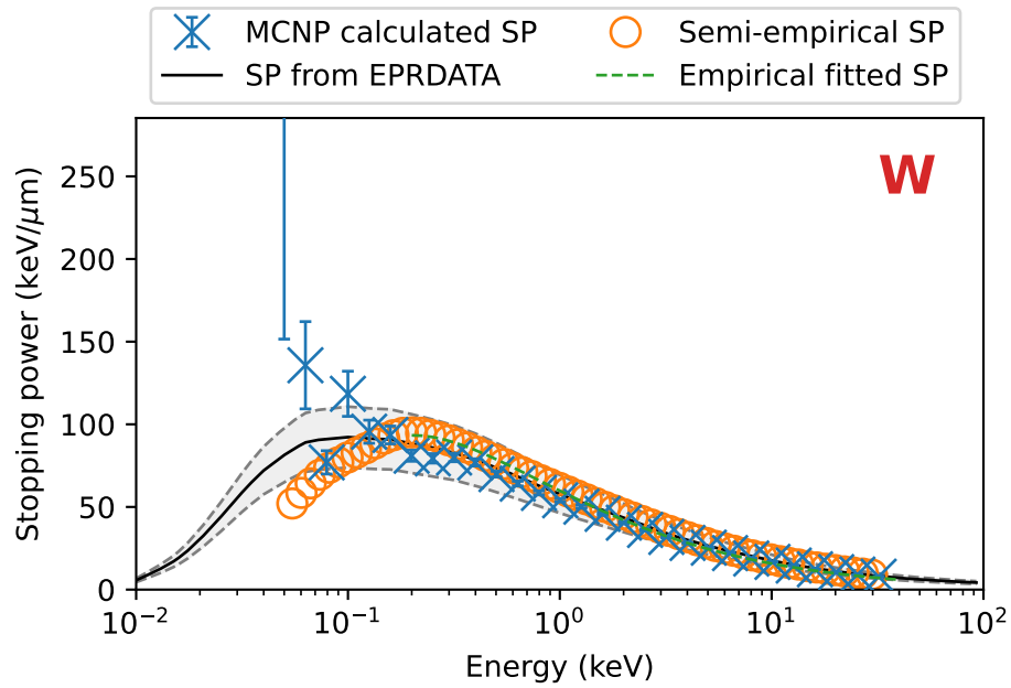
Figure 107: Stopping power results and benchmarks for tungsten.
