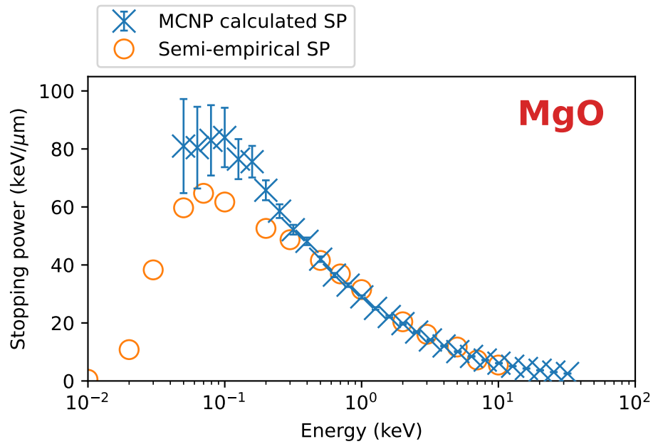
Figure 124: Stopping power results and benchmarks for magnesia.
