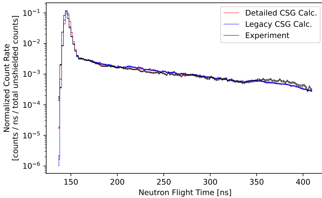
Figure 20: Comparison of the measured and calculated (ENDF/B-VII.0) normalized count rate of neutrons escaping from a 0.8 MFP (14-MeV neutron) thick sphere of beryllium plotted against flight time.
