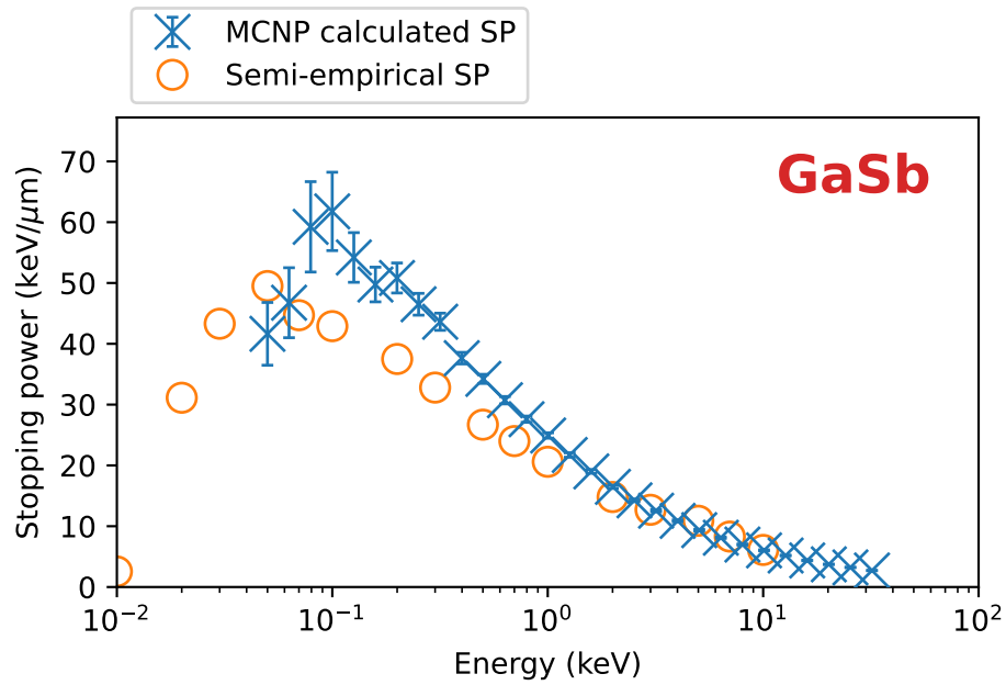
Figure 121: Stopping power results and benchmarks for gallium antimonide.
