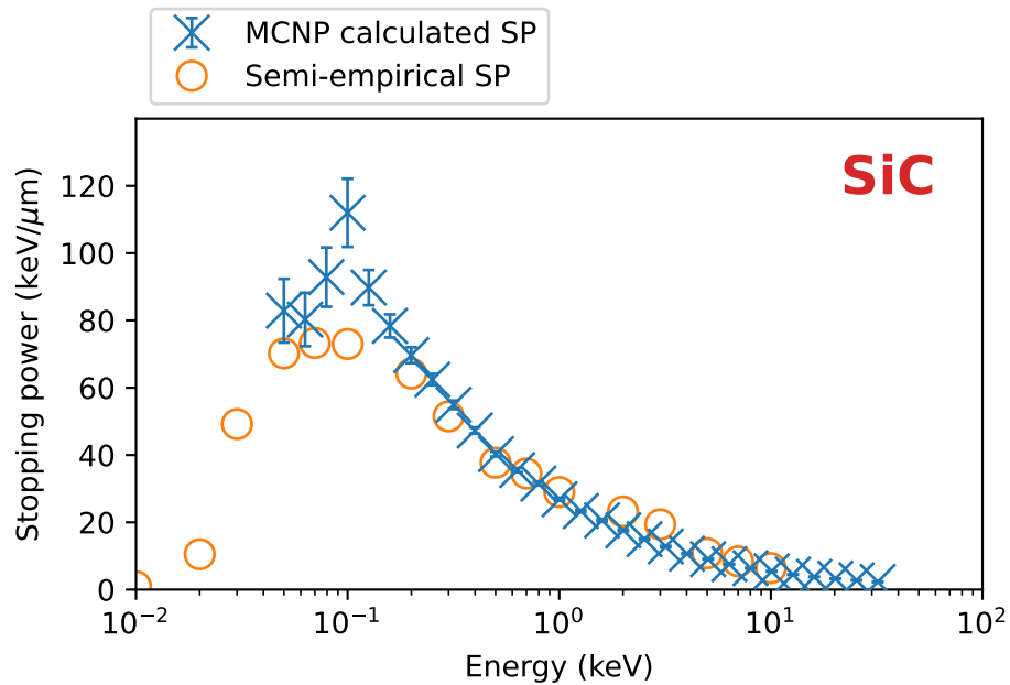
Figure 126: Stopping power results and benchmarks for silicon carbide.
