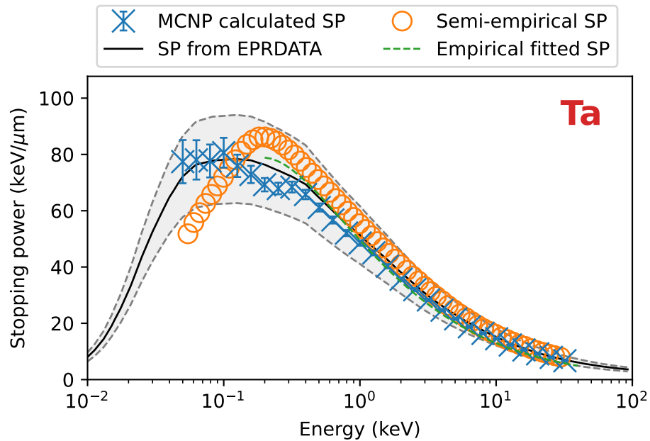
Figure 106: Stopping power results and benchmarks for tantalum.
