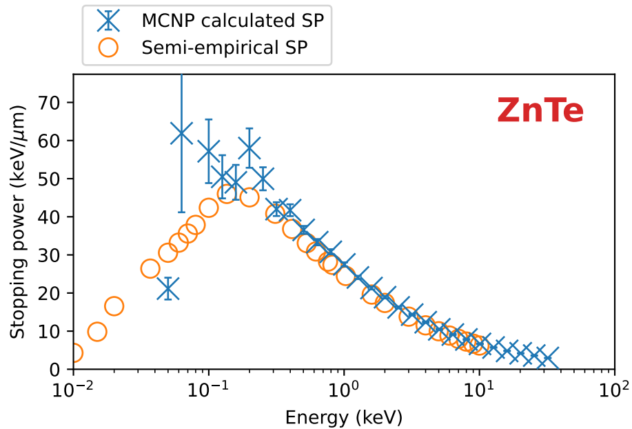
Figure 130: Stopping power results and benchmarks for zinc telluride.
