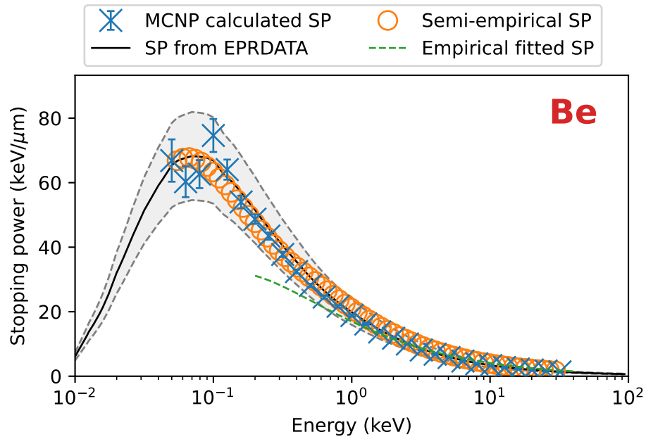
Figure 77: Stopping power results and benchmarks for beryllium.
