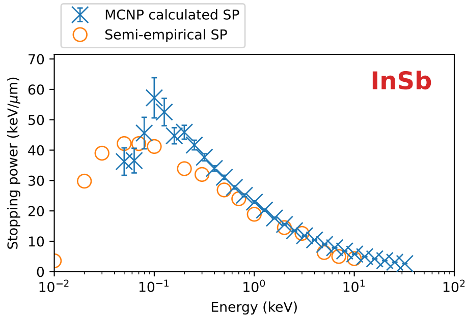
Figure 123: Stopping power results and benchmarks for indium antimonide.
