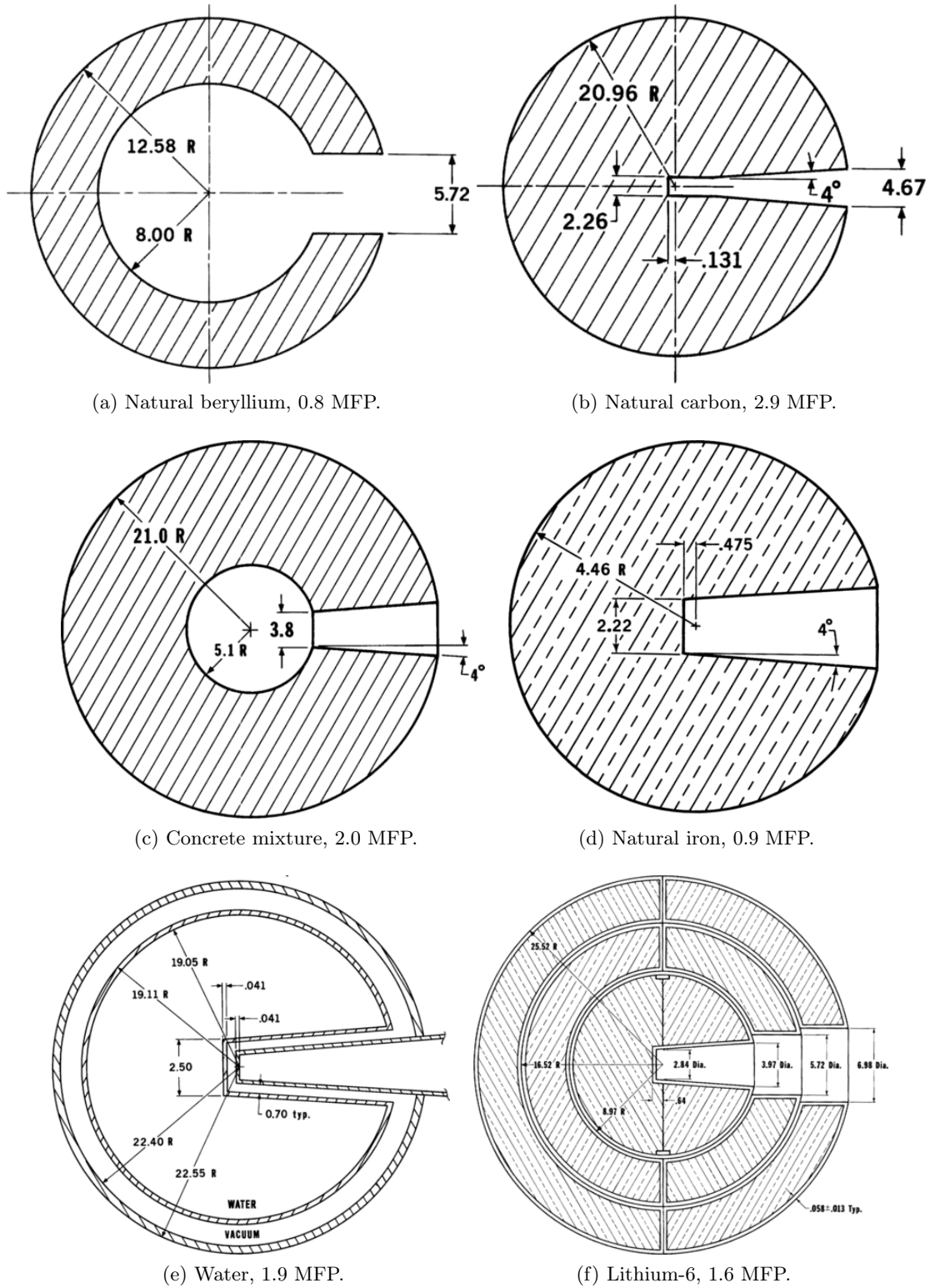
Figure 1: Pulsed sphere geometries reformatted from [15] (dimensions are centimeters).
