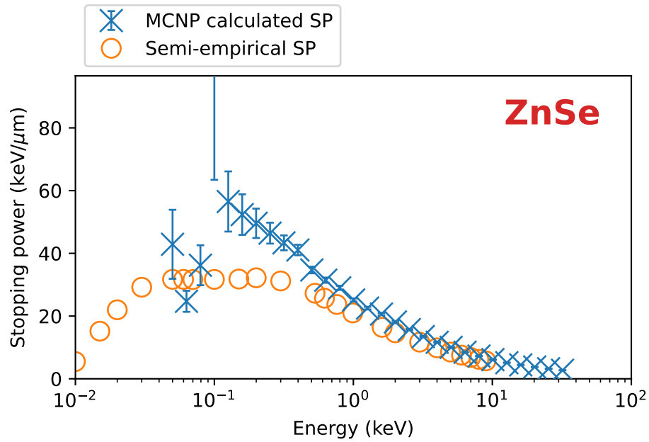
Figure 129: Stopping power results and benchmarks for zinc selenide.
