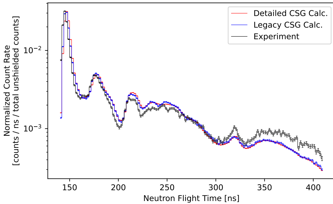
Figure 27: Comparison of the measured and calculated (ENDF/B-VII.1) normalized count rate of neutrons escaping from a 2.9 MFP (14-MeV neutron) thick sphere of carbon plotted against flight time.
