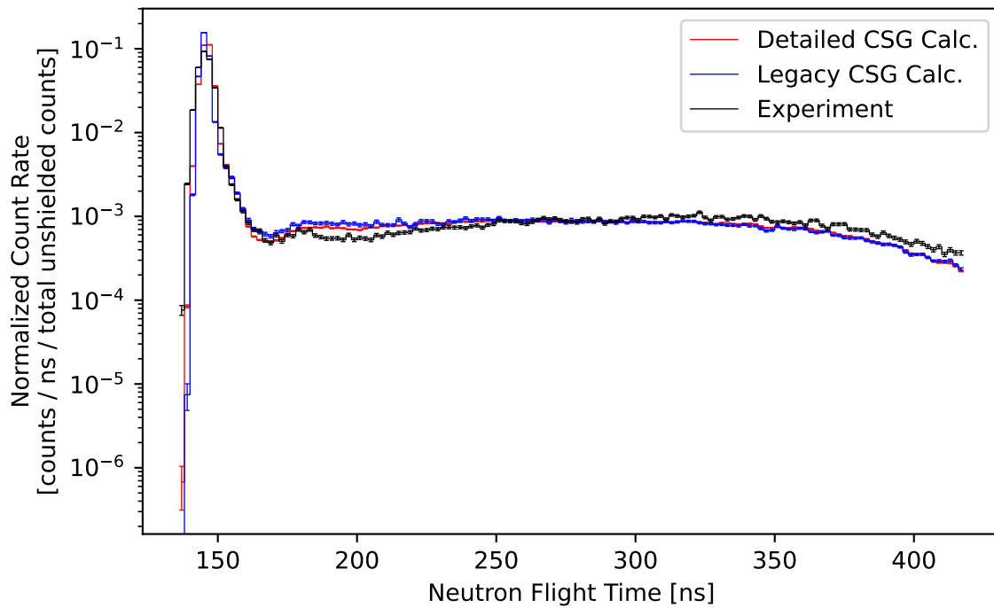
Figure 29: Comparison of the measured and calculated (ENDF/B-VII.1) normalized count rate of neutrons escaping from a 0.9 MFP (14-MeV neutron) thick sphere of iron plotted against flight time.
