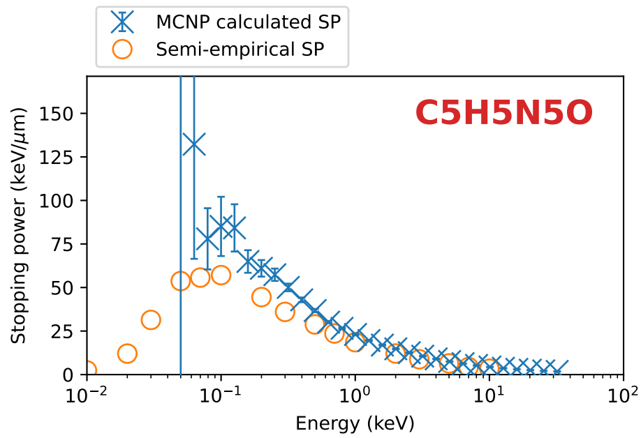
Figure 131: Stopping power results and benchmarks for guanine.
