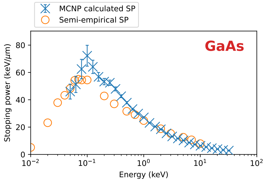
Figure 120: Stopping power results and benchmarks for gallium arsenide.
