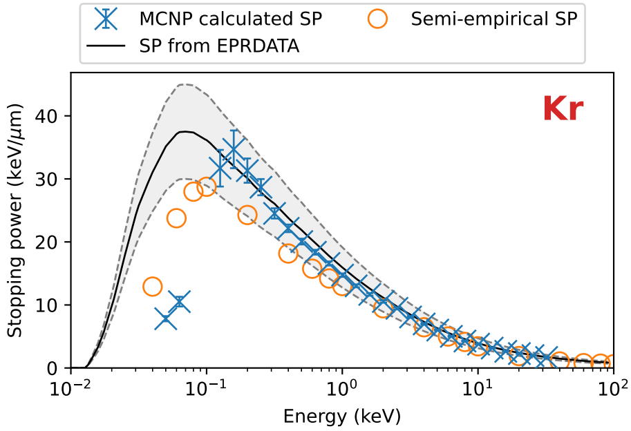
Figure 135: Stopping power results and benchmarks for solid krypton.
