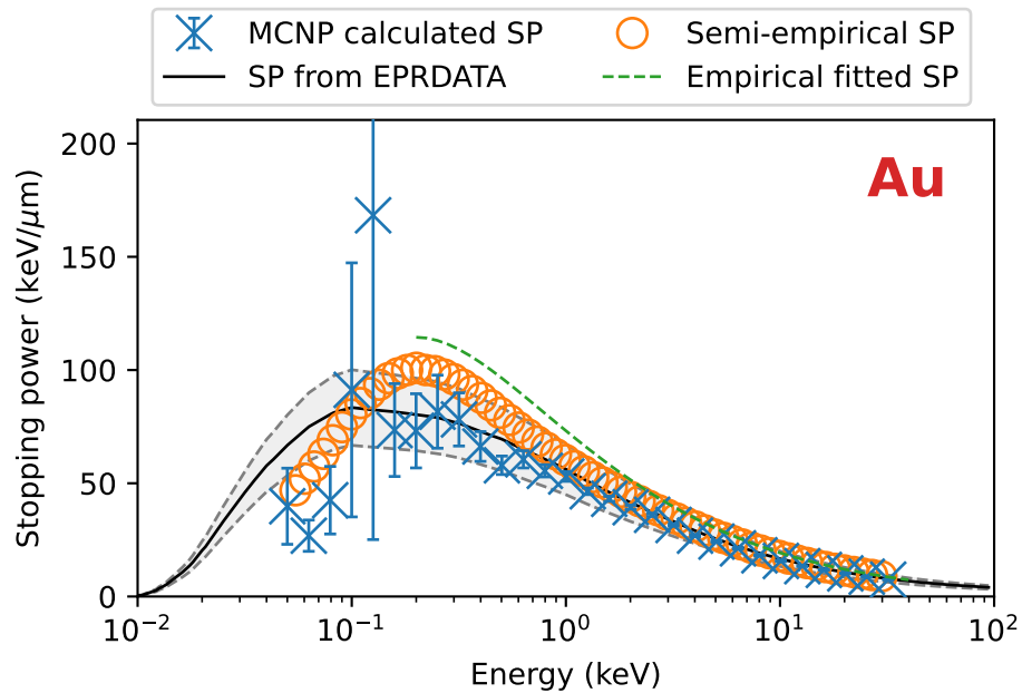
Figure 112: Stopping power results and benchmarks for gold.
