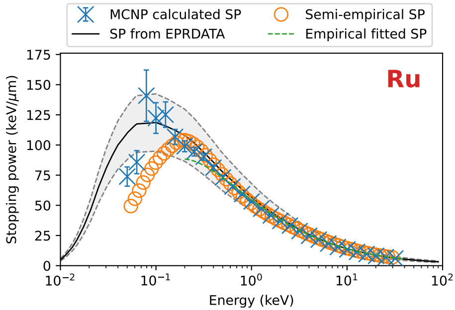
Figure 95: Stopping power results and benchmarks for ruthenium.
