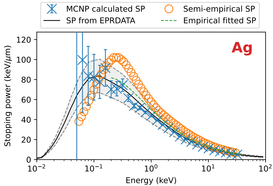
Figure 98: Stopping power results and benchmarks for silver.
