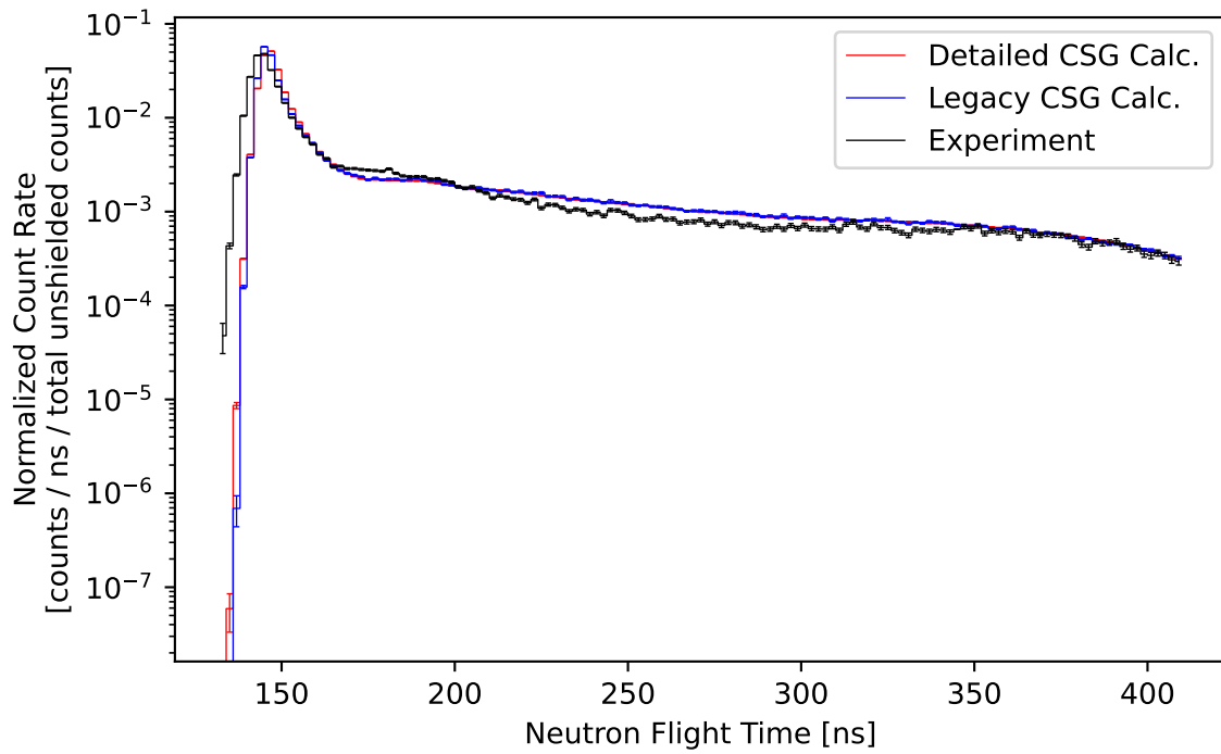
Figure 18: Comparison of the measured and calculated (ENDF/B-VI.6) normalized count rate of neutrons escaping from a 1.6 MFP (14-MeV neutron) thick sphere of lithium-6 plotted against flight time.
