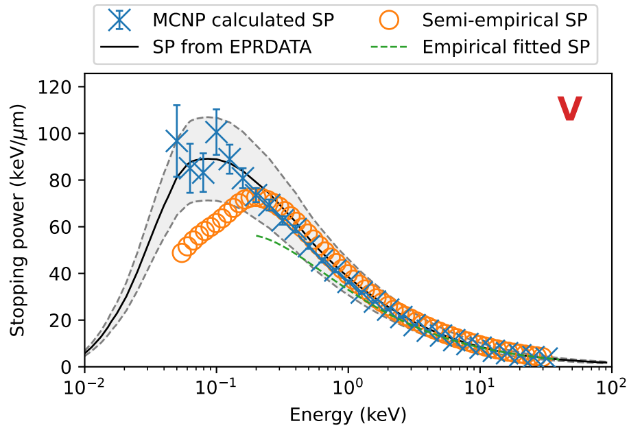
Figure 85: Stopping power results and benchmarks for vanadium.
