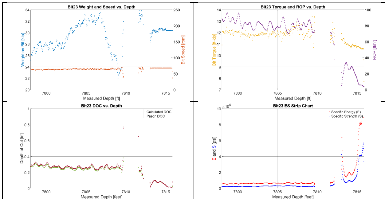
Figure 32. Bit 23 drilling record.
