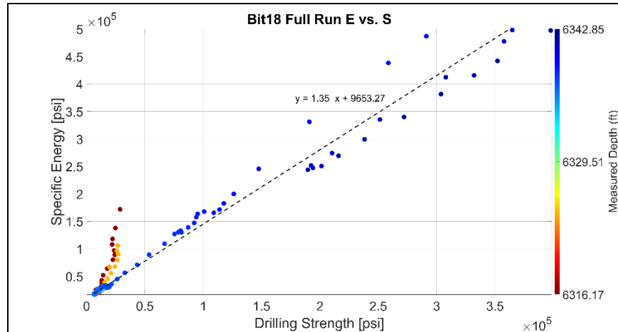
Figure 31. E-S diagram for Bit 18.
