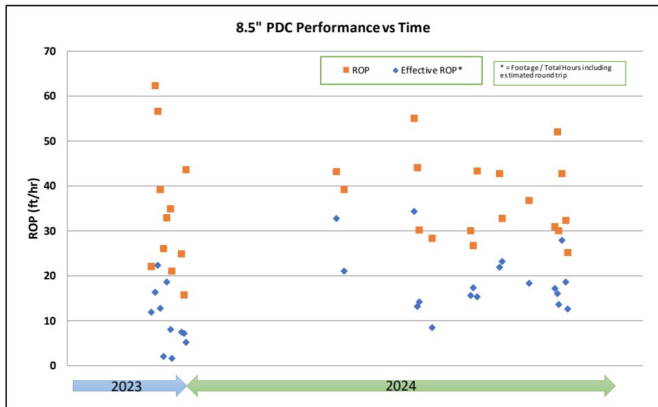
Figure 38. PDC ROP vs. time for wells following GDC-36
