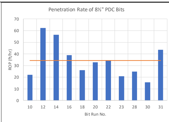
Figure 15. PDC bit ROP performance in the 8 1/2" interval.
