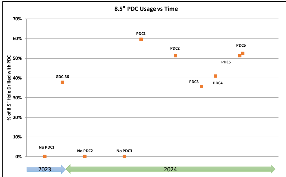
Figure 37. 8.5\" PDC usage vs. time at The Geysers
