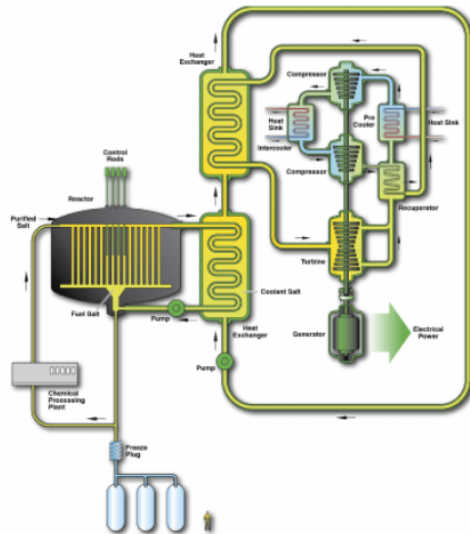
Figure 2-3. Molten Salt Reactor Example 13
