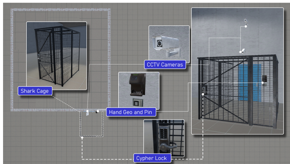
Figure 4-8. Vital Area PPS Equipment
