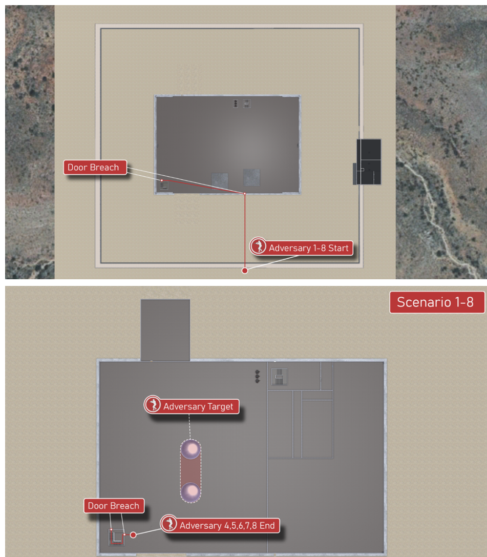
Figure 5-1. Adversary Attack Scenario One
