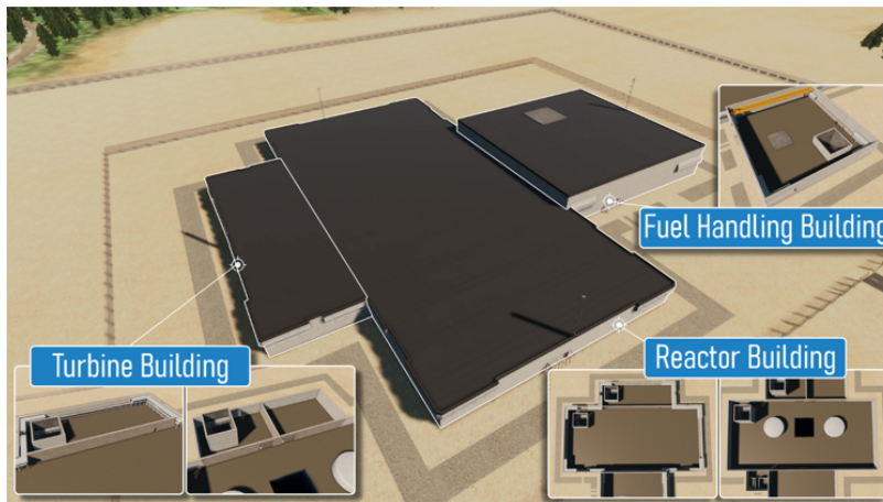
Figure 3-2. Hypothetical Sodium Fast Reactor (Single Building) 17
