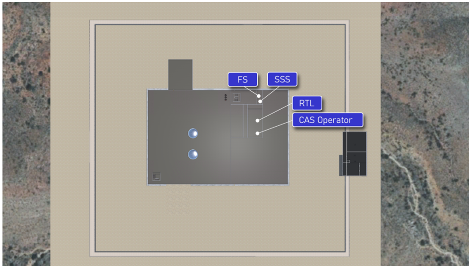
Figure 4-12. Below-Grade Physical Security Positions
