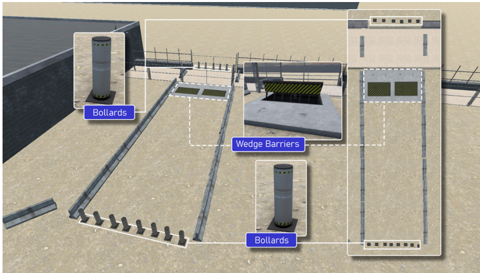
Figure 4-5. Vehicle Entry Control Point
