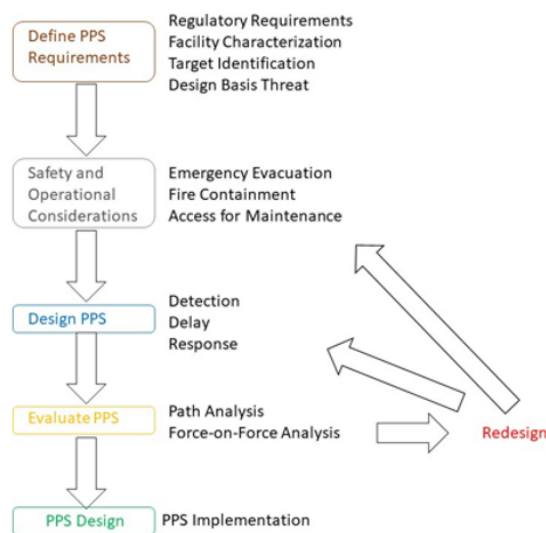
Figure 3-1. Security-by-Design Design and Evaluation Process Outline (DEPO) Approach
