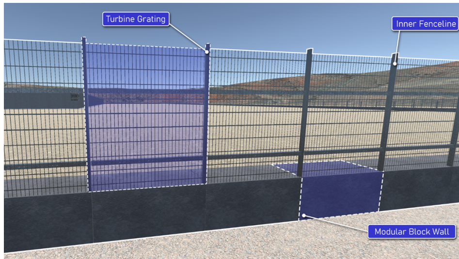
Figure 4-3. Inner Fence and Vehicle Barrier System
