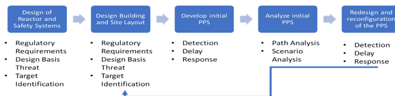
Figure 3-3. Hypothetical SMR and PPS Design Process
