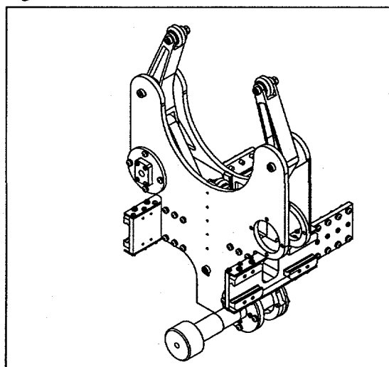
Figure 6: Overview of clamber system
