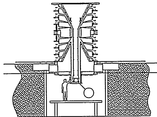
Fig. 1. PBFA-X configuration
