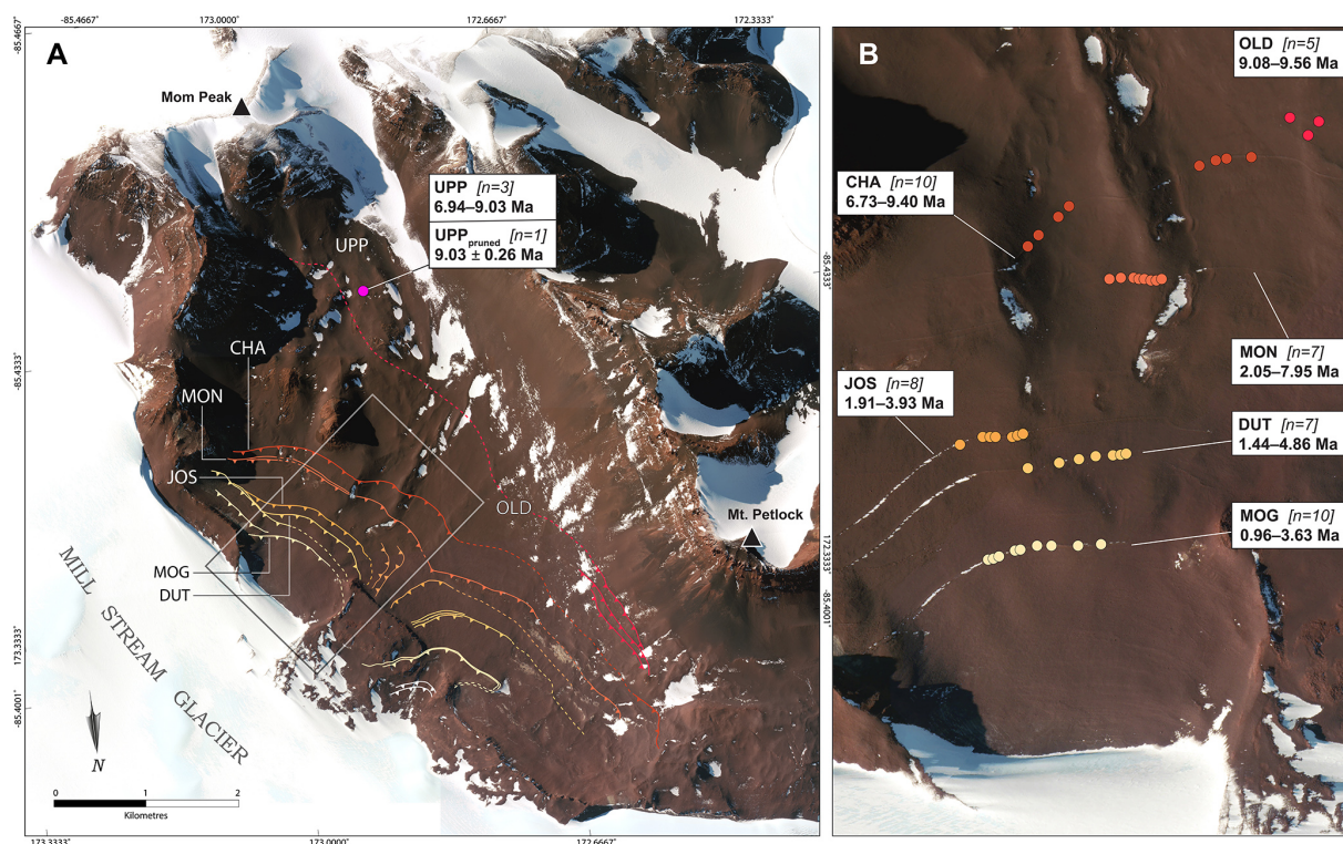
Figure 2. Glacial geomorphic map and cosmogenic nuclide surface-exposure chronology of the Otway Massif study area. (a) Relative positions of moraines and drift edges marking the former extent of the Mill Stream Glacier (EAIS) margin. Dashed lines denote inferred drift edges. The white box indicates the area covered in panel (b). Also shown are the cosmogenic ^3\text{He} surface-exposure ages for the Upper (UPP) drift unit for both single ( n = 3 ) and pruned ( n = 1 ) populations. Bold type denotes age ranges, while italics indicate mean ages. (b) Inset map of the Mogul (MOG), Dutch (DUT), Joshua (JOS), Montana (MON), Charlie (CHA), and Old (OLD) deposits and their corresponding ^3\text{He} surface-exposure ages. Note that ^{10}\text{Be} and ^{21}\text{Ne} ages for the Mogul moraine are not shown. The base map is derived from WorldView-2 satellite imagery (© 2013, DigitalGlobe, Inc.).
