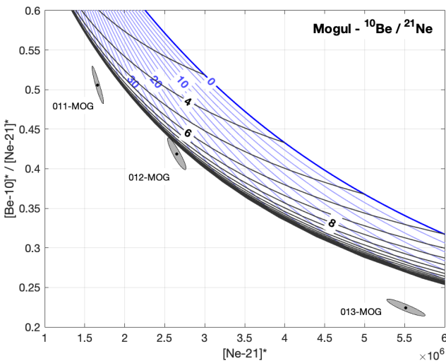
Figure 5. The 10 Be– 21 Ne normalised two-nuclide diagram for three sandstone erratics sampled on the Mogul moraine (15-OTW-011, 012, and 013). Numbered black and blue lines are isolines of constant exposure age (Ma) and steady erosion (cm Myr -1 ), respectively.
