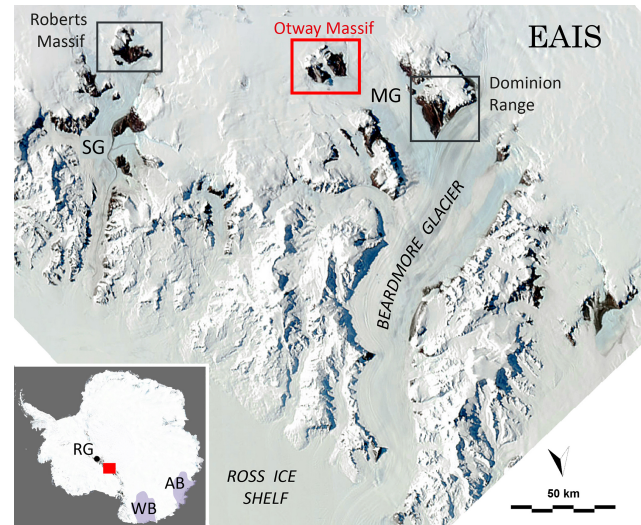
Figure 1. Location map showing position of Otway Massif and other Transantarctic Mountain sites mentioned in the text. SG stands for Shackleton Glacier, MG stands for Mill Glacier, RG (inset map) stands for Reedy Glacier. Also shown are the respective positions of the Aurora (AB) and Wilkes (WB) subglacial basins (inset map).
