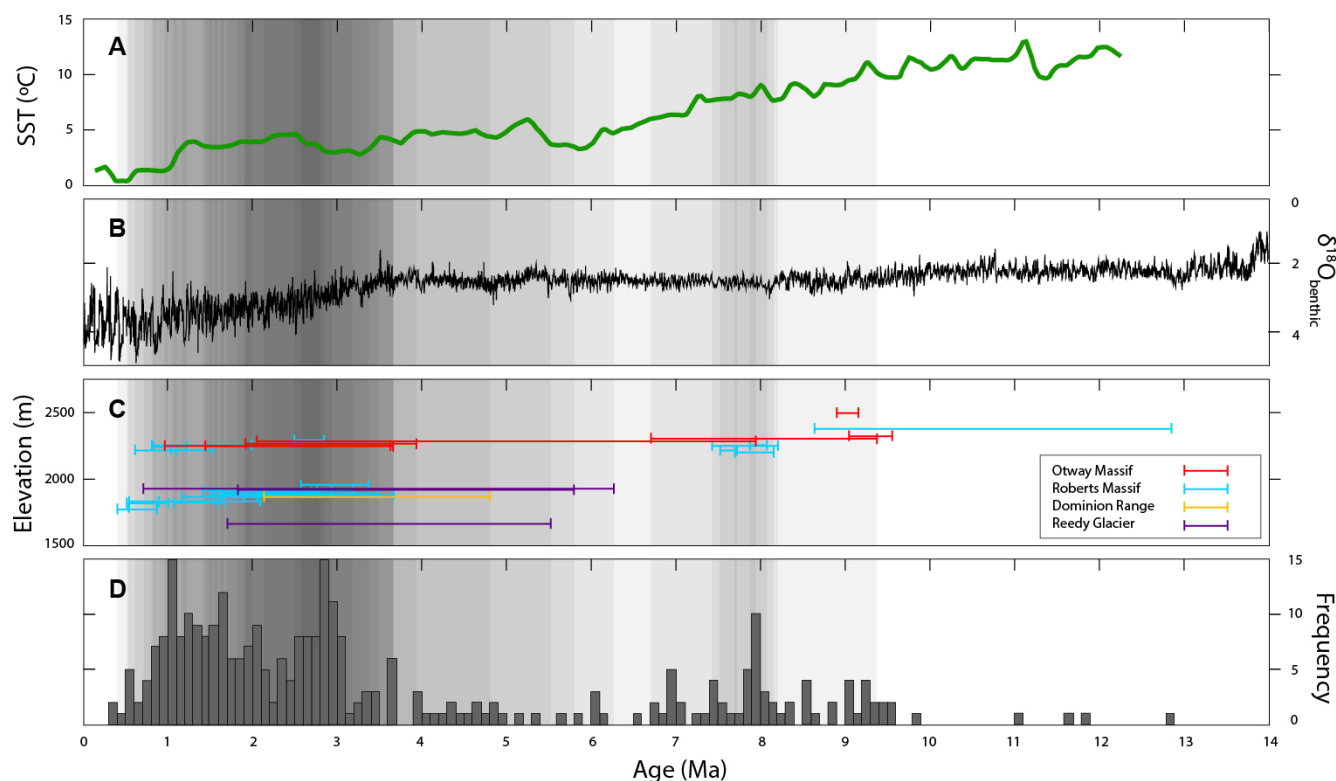
Figure 6. Temporal comparison of long-term global climate conditions and frequency of moraine deposition in the central and southern TAM, adapted from Balter-Kennedy et al. (2020) and including additional data from the present study and other published work (Ackert and Kurz, 2004; Bromley et al., 2010). (a) Southern Hemisphere average sea surface temperature reconstructed from alkenones (Herbert et al., 2016); (b) benthic oxygen isotope curve (De Vleeschouwer et al., 2017); (c) moraine age plotted against elevation for landforms at Otway Massif (red circles), Roberts Massif (turquoise circles), Dominion Range (yellow circle), and Reedy Glacier (purple circles); and (d) a histogram depicting all apparent exposure ages (all samples from each of the four TAM locations discussed) shown in panel (c). Grey shading scales with the extent of agreement in moraine ages across different landforms featured in panel (c).
