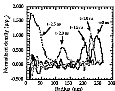
Figure 3: Radial density profiles calculated by Abel inverting radial lineouts of the x-ray transmission through the capsule.
