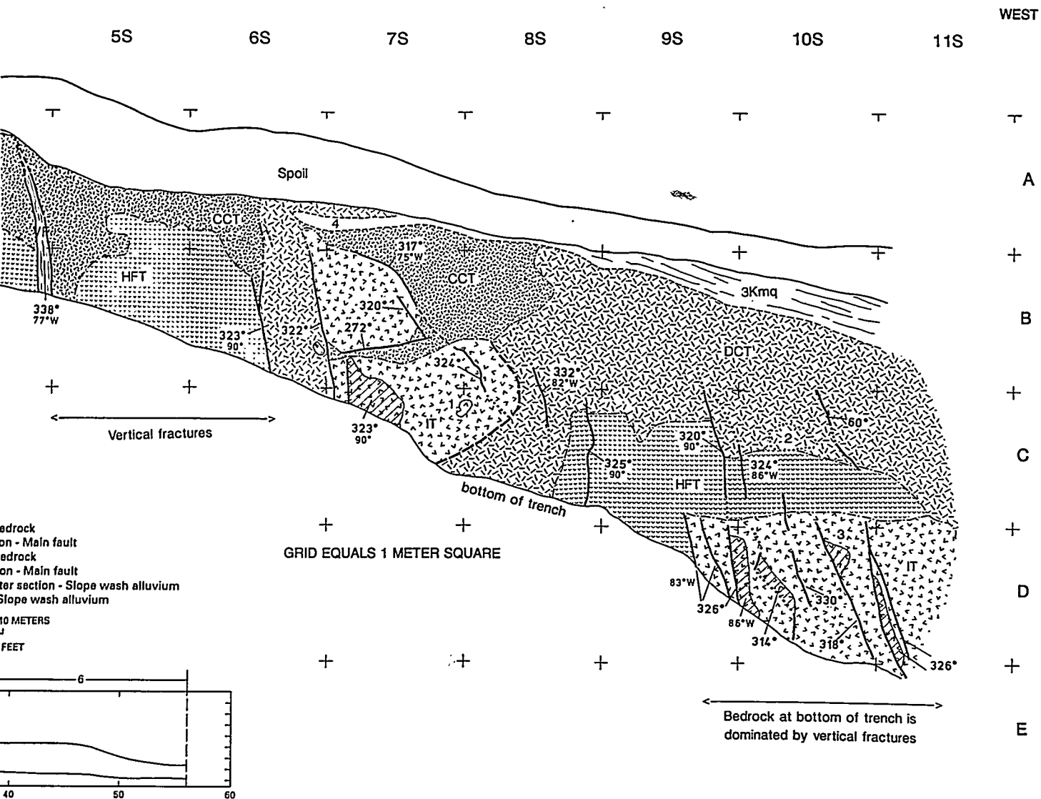
VIEWING THE BEDROCK EXPOSED ON THE SOUTH WALL, EAST END OF TRENCH 14 BOW RIDGE FAULT AT EXILE HILL, NYE COUNTY, NEVADA
