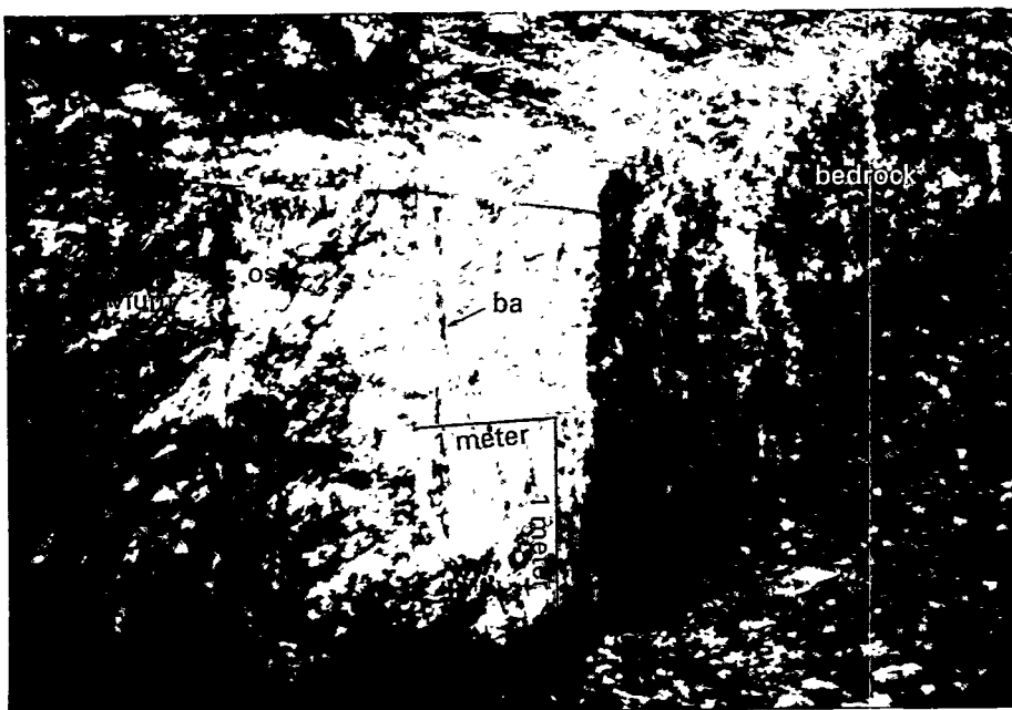
Figure 6. The main fault exposed on the north wall, center section, of trench 14. Symbols: ba, black ash and fractures filled with fine-grained sediment; os, dense opaline silica stringers. The very light-colored nonwelded tuff (NWT) is virtually indistinguishable from the adjacent slope-wash alluvium. See the center section of plate 1B for comparison.
