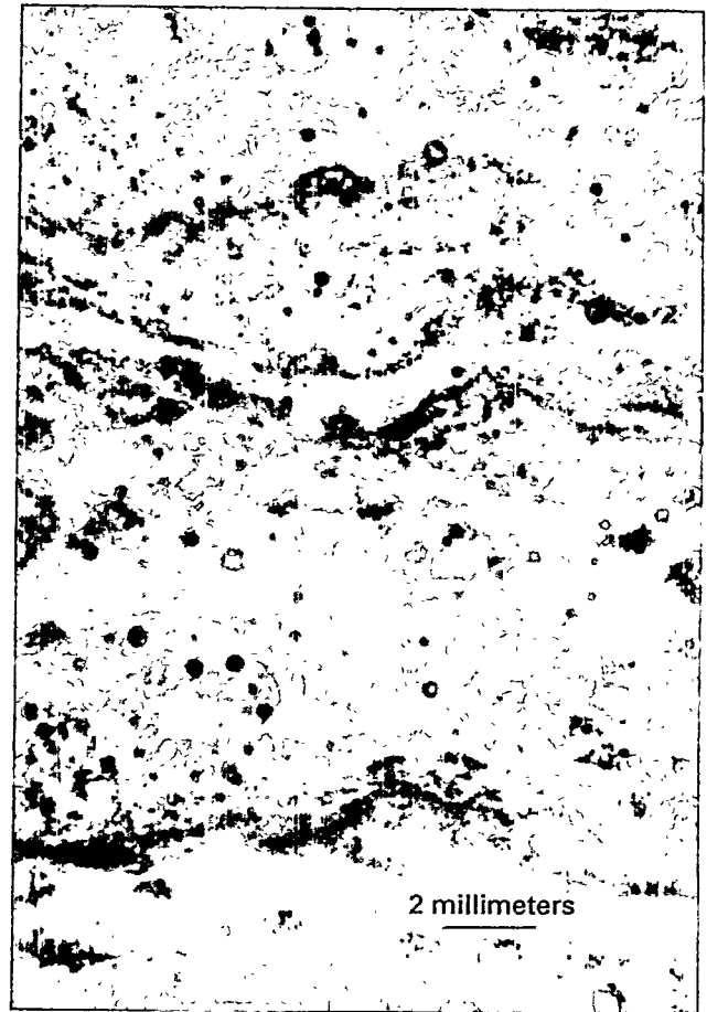
Figure 10. Photomicrograph of microcrystalline-banded carbonate with a crystallitic b-fabric. Material consists of fine particles of calcite mixed with clay particles.
