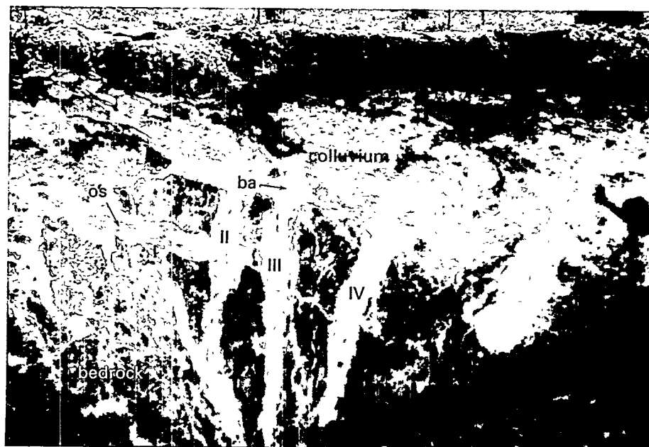
Figure 7. The main fault exposed on the south wall, center section, of trench 14. Symbols: ba, black ash and fractures filled with fine-grained sediment; os, dense opaline silica stringers. See the center section of plate 1D for comparison. Person in photograph is 160 centimeters tall.
