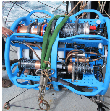
(b) Near surface instrument frame (NSIF)
