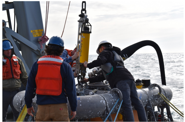
(d) With all mooring components except the MFN trail-cable and stretch hoses are fed aft, and buoyancy elements are transferred over the transom with the A-frame and released. The MFN is lifted clear of the deck, shifted outboard with the A-frame, and lowered into the water. The MFN is released when it is about 30 m above the sea floor.
