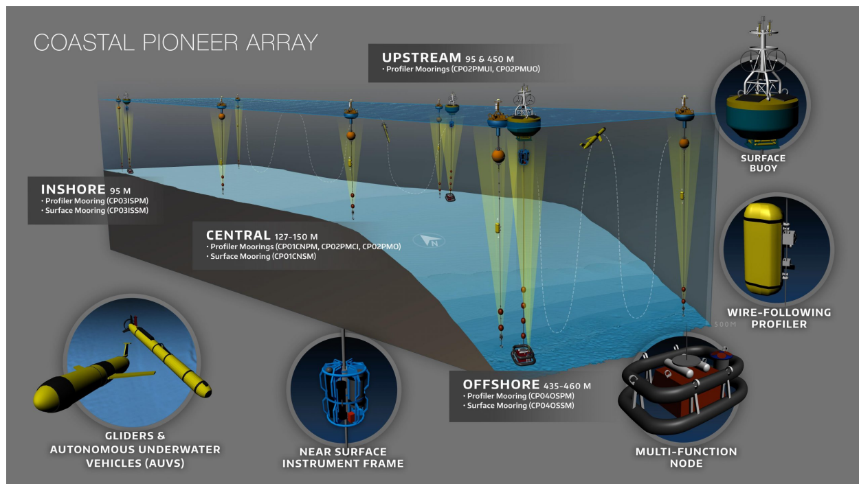
Figure 1-1 Coastal Pioneer Array sensor platforms (reproduced from https://oceanobservatories.org/array/coastal-pioneer-array/ ).
