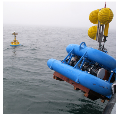
(c) Multi-function node (MFN)
