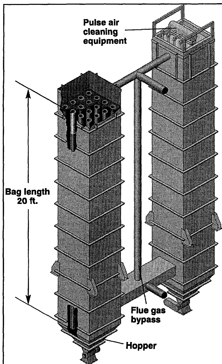
Figure 3.3 Baghouse
