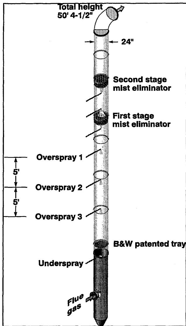
Figure 3.4 Wet Scrubber
