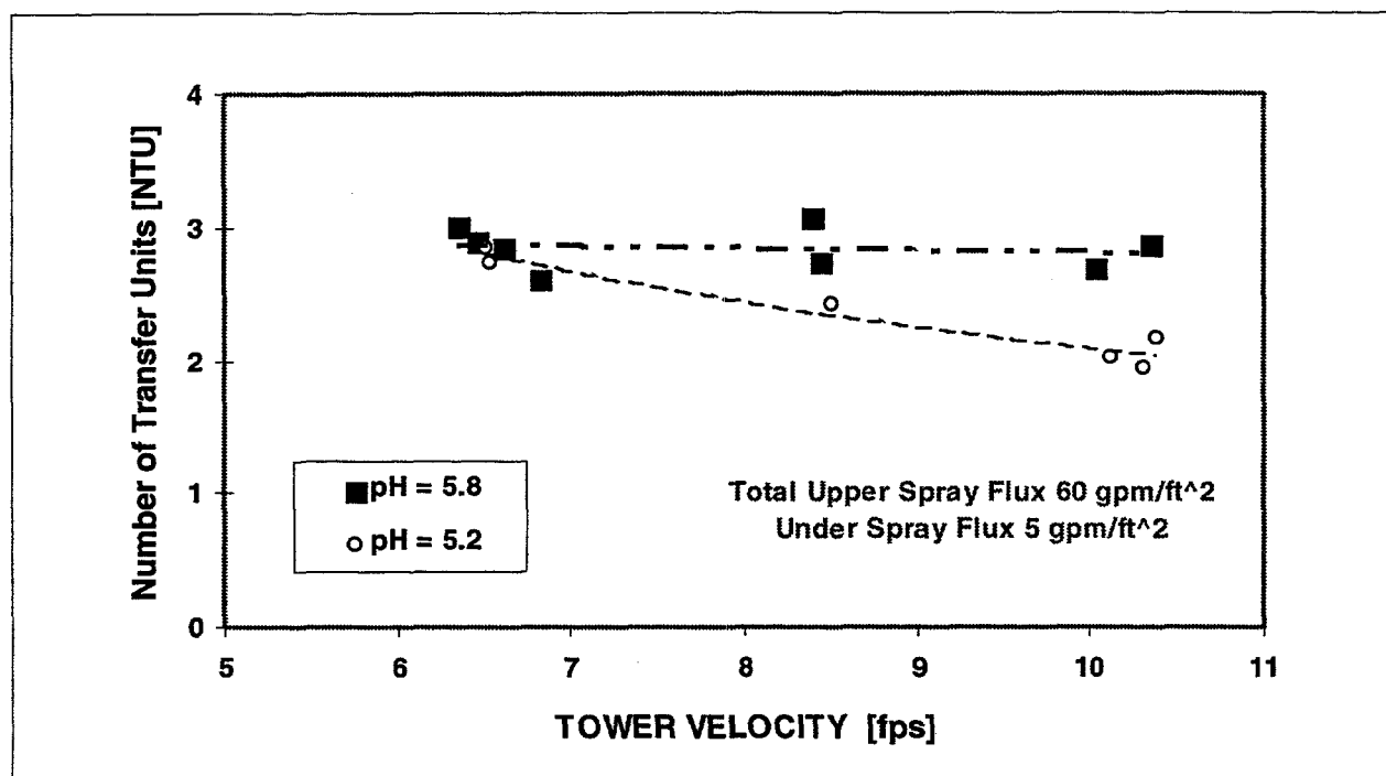
Figure 4.6 Effect of pH and Tower Velocity on \text{SO}_2 Performance, LSFO
