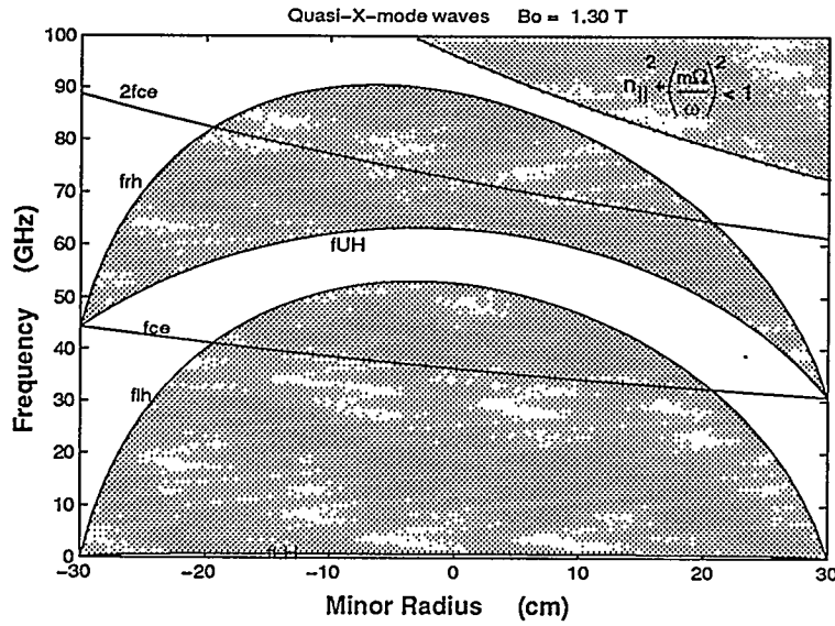
Figure 1: Accessibility diagram in the midplane for PBX-M parameters under the plasma conditions n_{eo} = 3.3 \times 10^{13} \text{ cm}^{-3} , B_{To} = 1.3T , and viewing angle = 57^\circ with respect to the toroidal direction. Emission cannot originate in the shaded regions. Upshifted second harmonic emission in the range 65 - 90 GHz is spatially localized between the right-hand cutoff and the condition imposed by Eqn. 2.
