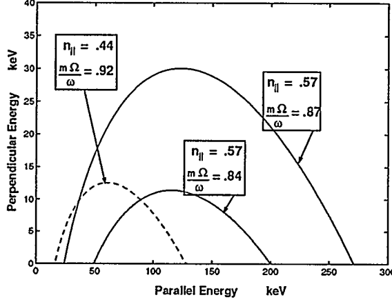
Figure 3: Solid lines illustrate the change in the resonance curve due to a change in the ratio \frac{m\Omega}{\omega} at a constant n_{||} . The dotted line illustrates the change in the resonance curve due to a change in the viewing angle ( n_{||} ).
