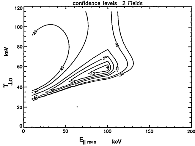
Figure 7: Confidence levels given by P(\Theta|D) found from Eqn. 9 (where \Theta = [E_{||max}, T_{\perp 0}] ) for middle radial region while the Lower Hybrid power is on, time = 417 in Table 1. The most probable solution is the maximum of the distribution, marked by +.
