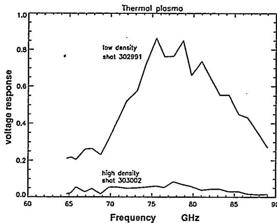
Figure 5: Lower line shows measured emission from a high density ohmic plasma for which the thermal emission is cut off, n_{eo} = 3. \times 10^{13} cm^{-3} , T_{eo} = 700eV , B_{To} = 1.3T . The upper line shows the thermal emission from a low density plasma where the thermal layer can be observed, n_{eo} = 1. \times 10^{13} cm^{-3} , T_{eo} = 900eV , B_{To} = 1.3T . The low level of emission in the high density case demonstrates that the viewing dumps are effective.
