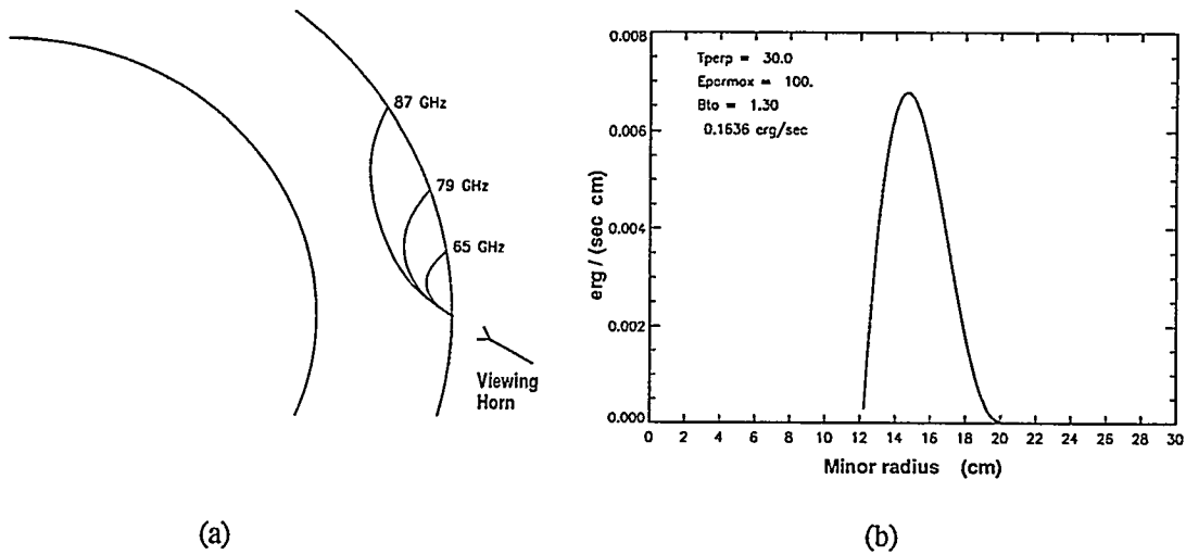
Figure 2: (a) Toroidal view of observation ray path, n_{eo} = 3.4 \times 10^{13} \text{ cm}^{-3} , B_{To} = 1.3T , viewing angle = 57^\circ with respect to the toroidal direction. (b) Second harmonic emission along ray path at 80 GHz given a fast electron energy distribution which is constant with radius with a density of 2 \times 10^{10} \text{ cm}^{-3} , a plateau to a high parallel energy cutoff of 100 keV and a perpendicular temperature of 30 keV.
