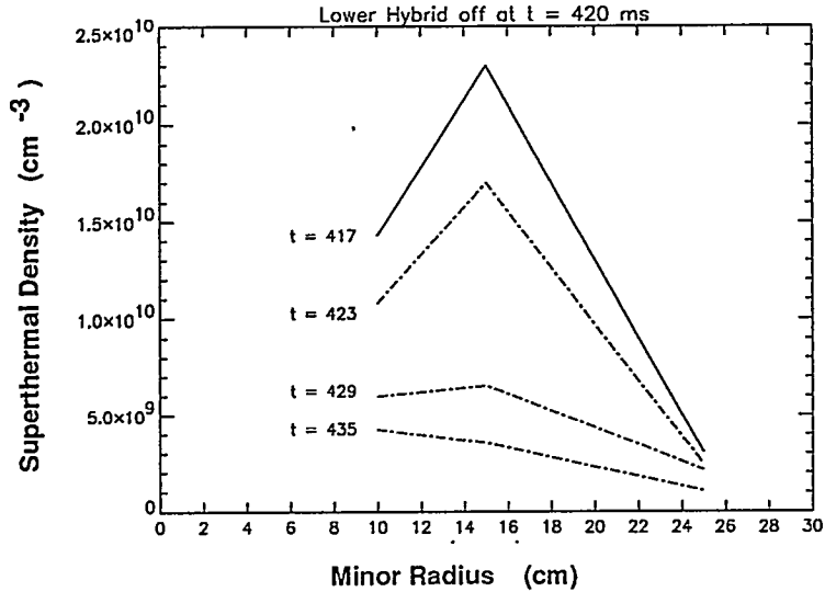
Figure 8: Radial profile of the superthermal density measured by the Oblique ECE system. The dotted lines show the time evolution of the density profile after the Lower Hybrid power is turned off at 420 ms.
