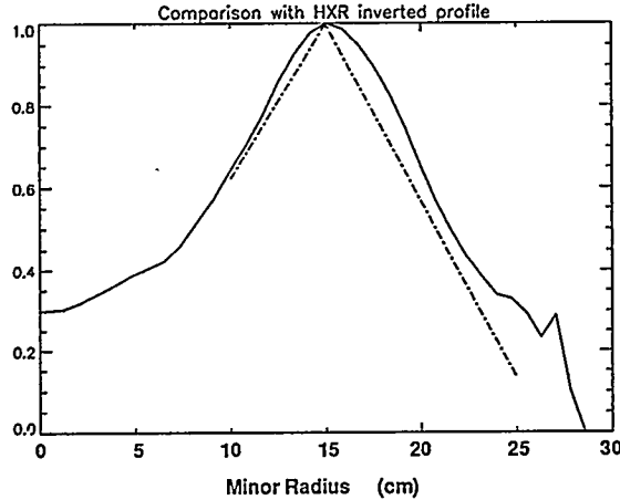
Figure 9: Solid line shows the normalized inverted Hard X-ray emissivity profile on the outer midplane while the Lower Hybrid power is on. Dotted line shows the normalized density profile measured by Oblique ECE at the same time.
