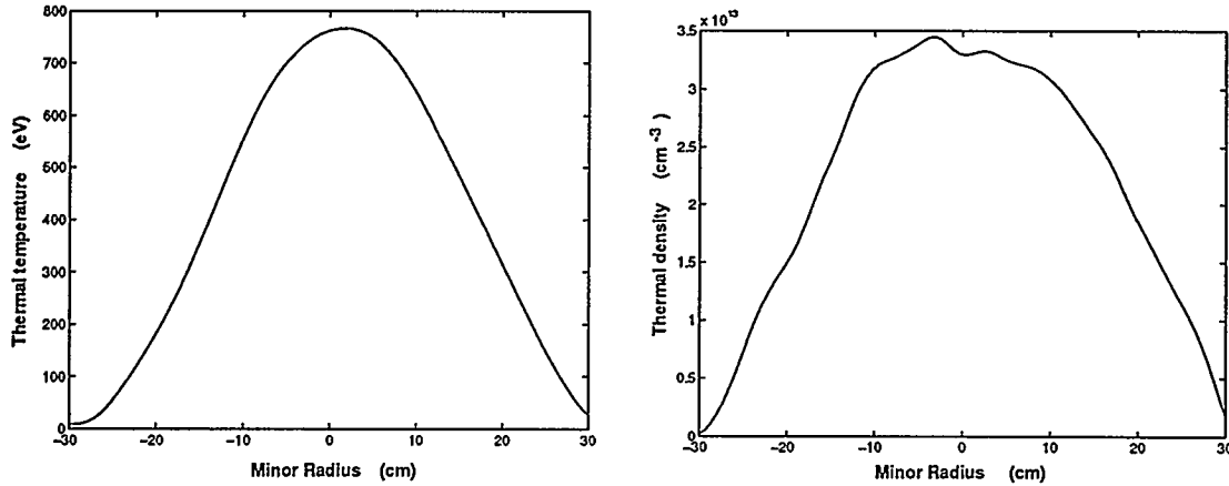
Figure 6: Typical temperature and density profiles for the shots used in this analysis. PBX-M shots 312021 - 312060.
