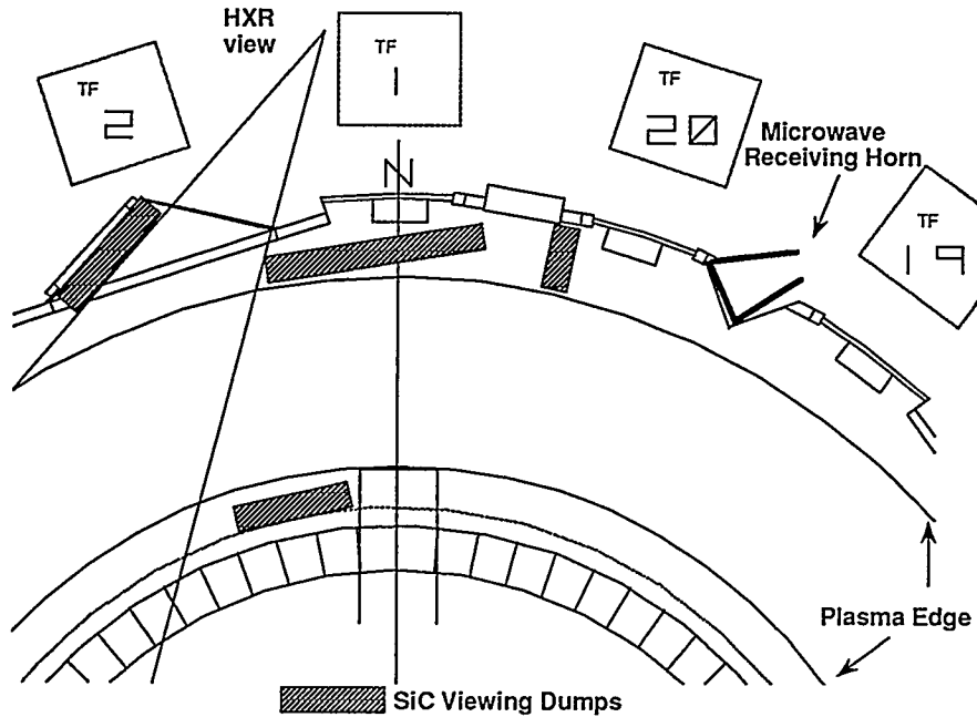
Figure 4: Toroidal view of PBX-M showing the arrangement of the microwave antenna and the SiC viewing dumps for the Oblique Electron Cyclotron Emission diagnostic.
