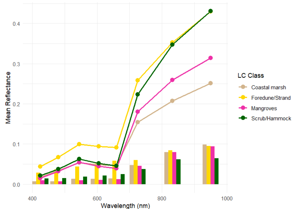
Figure 4. Spectral profiles of four vegetation classes: coastal marsh, mangroves, foredune/strand, and scrub/hammock. The spectral profiles are the mean reflectance values at the WorldView eight bands, calculated from the WorldView imagery of 8 October 2016 and 4 August 2023. Standard deviations within each band/class combination are displayed as bars below the lines.
