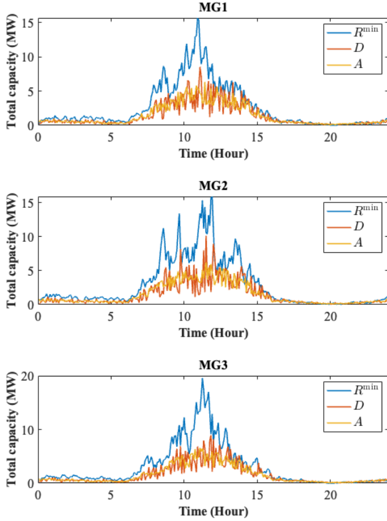
Fig. 10: Minimum required EVCS charging capacity ( R^{\min} ), capacity of EV arrival ( A ) and EV departure ( D ) of three MGs in one day
