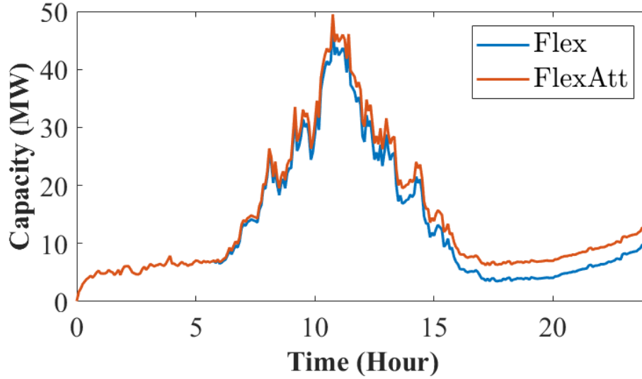
Fig. 14: Comparison of total EV capacity between Flex and FlexAtt .
