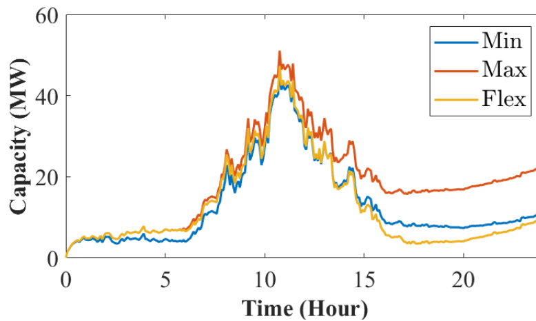
Fig. 11. Comparison of total EV capacity between three strategies
