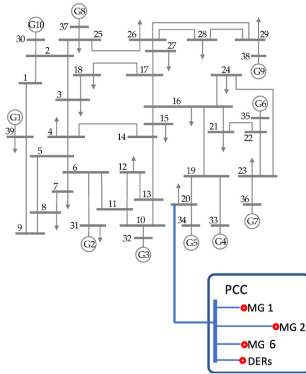
Fig. 3: IEEE 39-bus testcase with 6 microgrids connected to one distribution feeder at bus 20.
