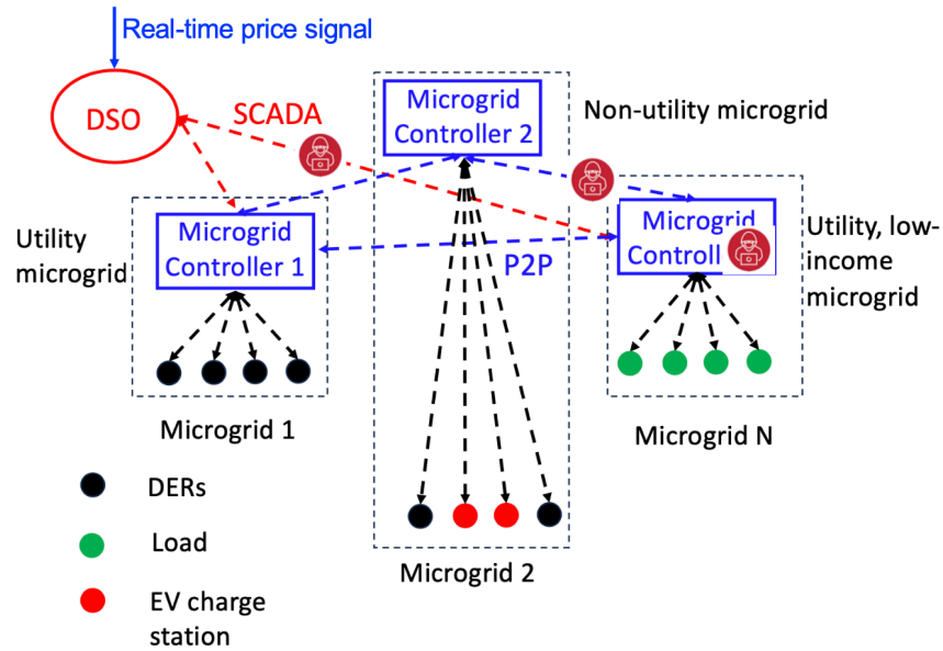
Fig. 5: Communication architecture to support the price signal-based operations of EV-rich networked microgrids with mixed ownership
