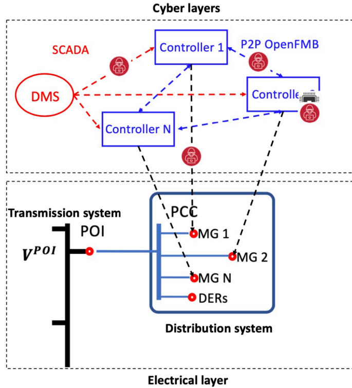
Fig. 1: Electrical and cyber architecture in operations of networked microgrids connected with the BPS.
