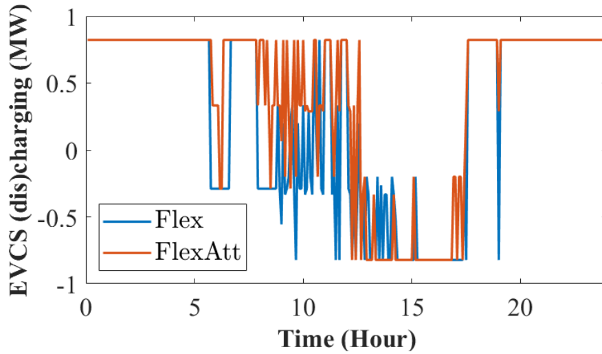
Fig. 15: Comparison of EVCS (dis)charging for the three MGs between Flex and FlexAtt .
