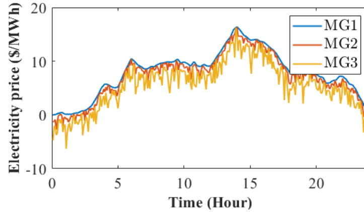
Fig. 13: (Estimated) price signals for each MG under attack
