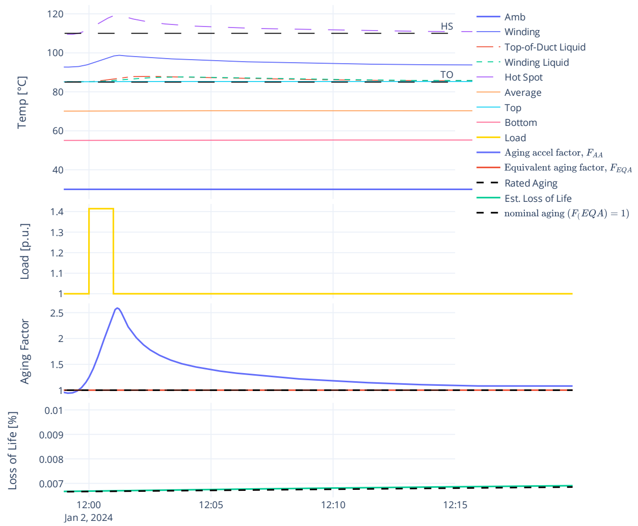
Figure 2 Results under same conditions in Figure 1 using the differential equations method.
