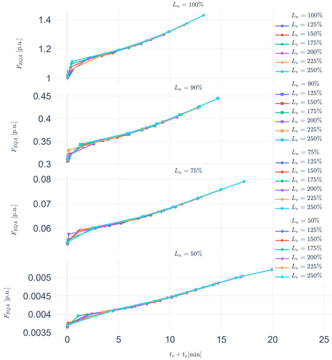
Figure 6 Results based on the analytical method from [3] showing the equivalent aging factor, F_{EQA} .
