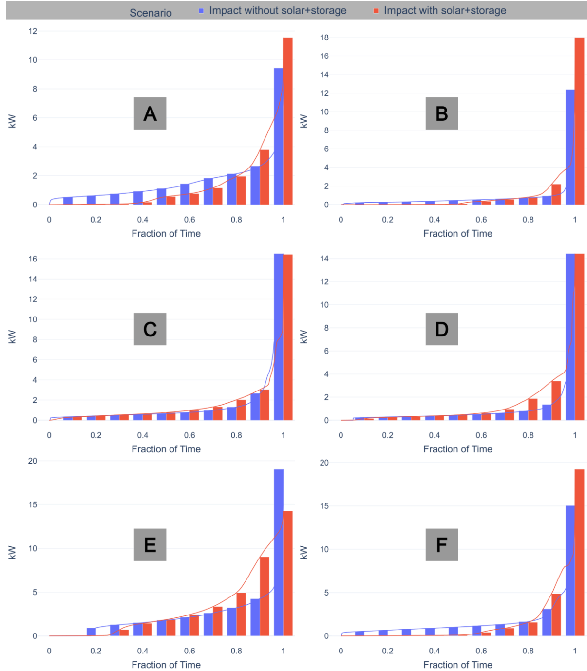
Figure 7 Ordered statistics for p^0[t] and p[t] . Bars are shown for each of the 10 th , 10 th , 20 th , ..., 90 th , 100 th percentiles, while the lines show the full ordered data.
