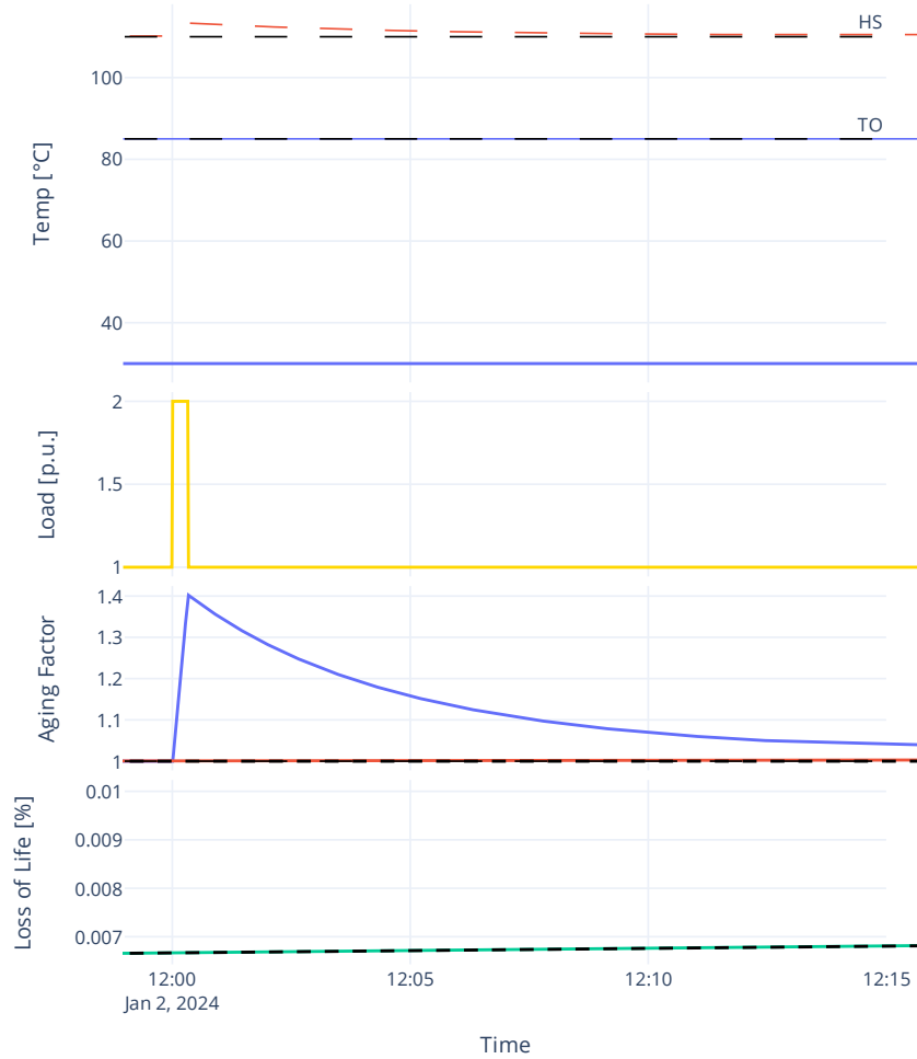
Figure 1 Comparison between results using the analytical method at the second level (left) and at loading averaged over a minute (right). The similarity between the two justifies the use of averaged minute load profiles.
