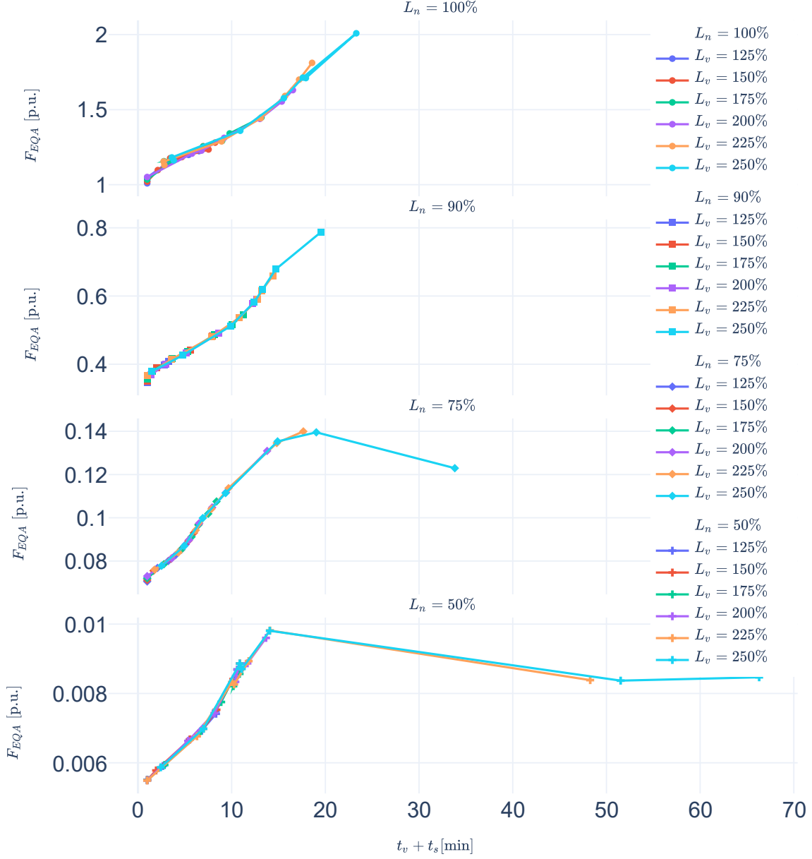
Figure 4 Results based on the differential equations method showing the equivalent aging factor, F_{EQA} .
