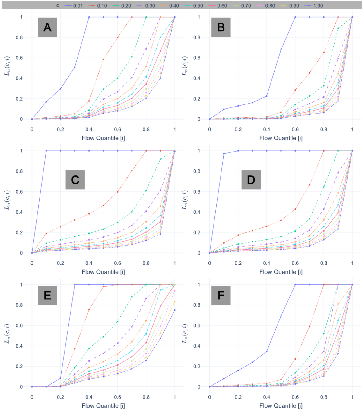
Figure 8 Estimated loading level based on assumed coincidence factor and chosen percentile flow, L_n(c, i) .
