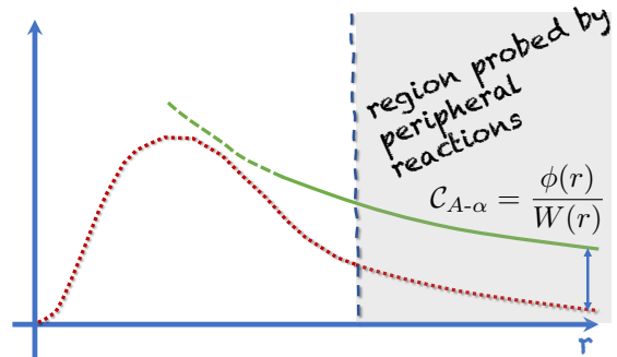
FIG. 1. Schematic representation of the radial part of the A - \alpha wavefunction \phi(r) (dotted red line) and the Whittaker function W(r) (green continuous line). They differ by a constant factor, namely the asymptotic normalization constant \mathcal{C}_{A-\alpha} . Peripheral reactions are only sensitive to the asymptotic behavior of the A - \alpha wavefunction (shaded area).
