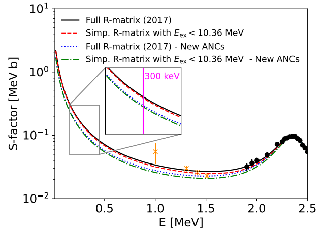
FIG. 3. Comparison of the ^{12}\text{C}(\alpha, \gamma)^{16}\text{O} S-factors as a function of the relative ^{12}\text{C} - \alpha relative energy, obtained with the R-matrix analysis of deBoer et al. [?] ] (solid black line), a simplified version in which only the low-energy states and the \alpha -channel are included (dashed red line), and predictions using our (C_{\alpha-^{12}\text{C}}^{J^\pi})^2 displayed in Table ?? (dotted blue and dash-dotted green lines). These S-factors have been obtained using the code AZURE2 [?] ], and the input files are provided in Supplemental Material [?] ]. The total S-factor data from Refs. [?] ] (black circles) and [?] ] (orange crosses) are also shown for comparison. The inset show the S-factors around the stellar energies (in magenta).
