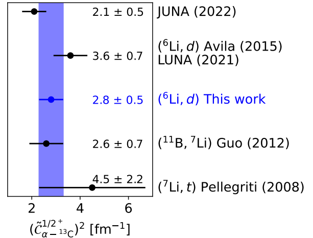
FIG. 2. Comparison of the square of the Coulomb-modified ANC of the 1/2^+ threshold state in {}^{17}\text{O} , (\tilde{C}_{\alpha-{}^{13}\text{C}}^{1/2^+})^2 , deduced from: the R-matrix analysis of the JUNA collaboration [?], the values extracted from ({}^6\text{Li}, d) data [?] using the (C_{\alpha-d})^2 of Ref. [?], our reinterpretation of the ({}^6\text{Li}, d) data [?] using a first-principle prediction of (C_{\alpha-d})^2 [?], the values inferred from ({}^{11}\text{B}, {}^7\text{Li}) data [? ?], ({}^7\text{Li}, t) data [?]. The numbers in the figure correspond to the values of the corresponding ANCs and their uncertainties.
