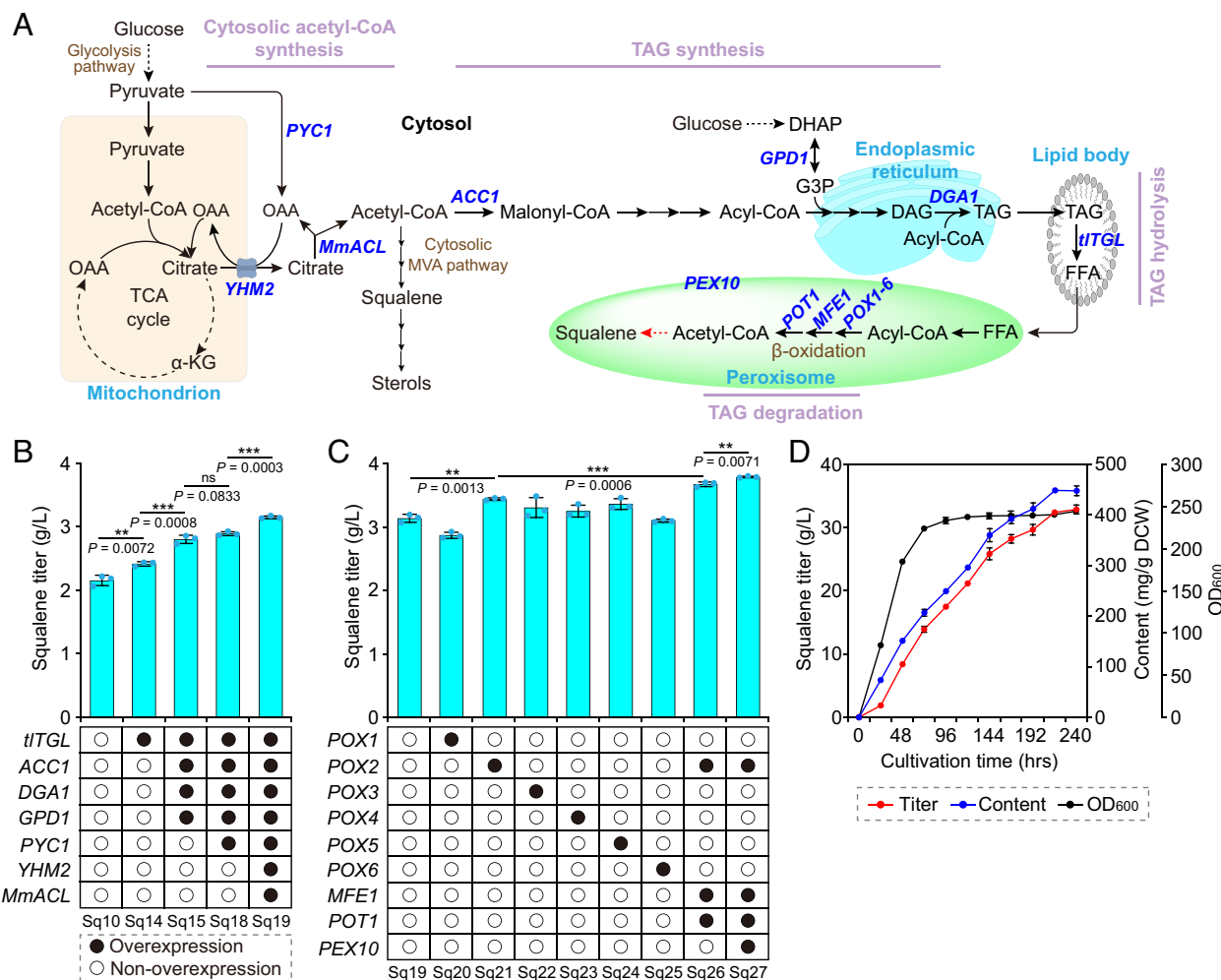
Fig. 3. Converting lipid by-product to peroxisomal squalene through lipid metabolism. (A) Schematic illustration of intracellular lipid metabolism, including its biosynthesis, hydrolysis, and degradation. Overexpressed genes in this study are shown in blue. PYC1, pyruvate carboxylase. YHM2, mitochondrial citrate carrier. MmACL, ATP: citrate lyase from Mus musculus . ACC1, acetyl-CoA carboxylase. GPD1, NAD + -dependent G3P dehydrogenase. DGA1, diacylglycerol acyltransferase. \alpha -TG, lipase from T. lanuginosus . POX1-6, acyl-CoA oxidases. MFE1, multifunctional \beta -oxidation protein. POT1, 3-ketoacyl-CoA thiolase. PEX10, peroxisome biogenesis factor. (B) Engineering lipid biosynthesis and hydrolysis by overexpressing rate-limiting enzymes increased squalene production in the peroxisome. (C) Engineering lipid degradation by strengthening the \beta -oxidation pathway increased squalene production in the peroxisome. (D) Fermentation profiles of squalene-producing strain Sq27 in a 3-L bioreactor. Statistical significance was tested using the two-sided Student's t test; ** P < 0.01 and *** P < 0.001 ; ns, not significant. All data are represented as mean \pm SD of three biologically independent experiments.
