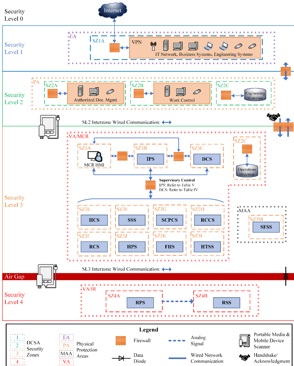
Figure 19. HTGR DCSA Template
