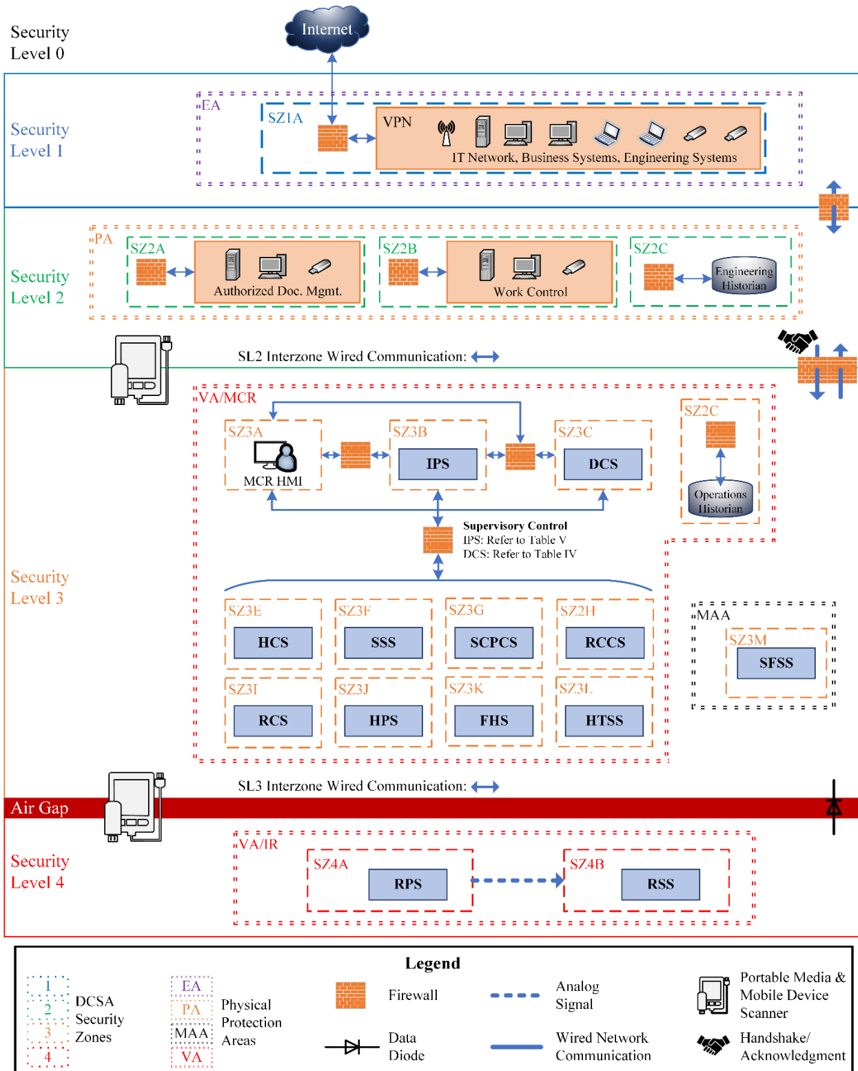
Figure 1. HTGR DCSA Template
