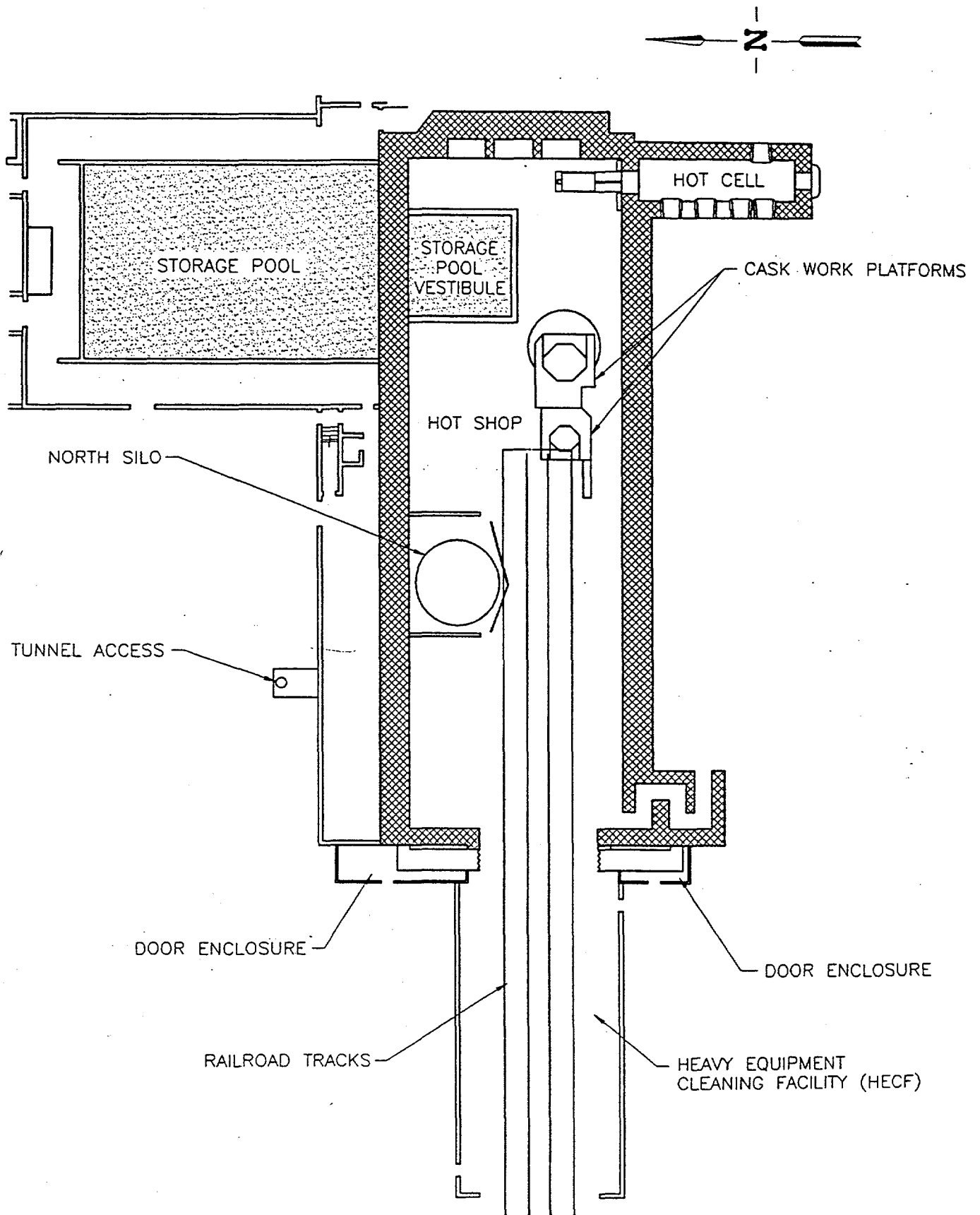
Figure 2. Diagram of the TAN Hot Shop and TAN Pool Area.
