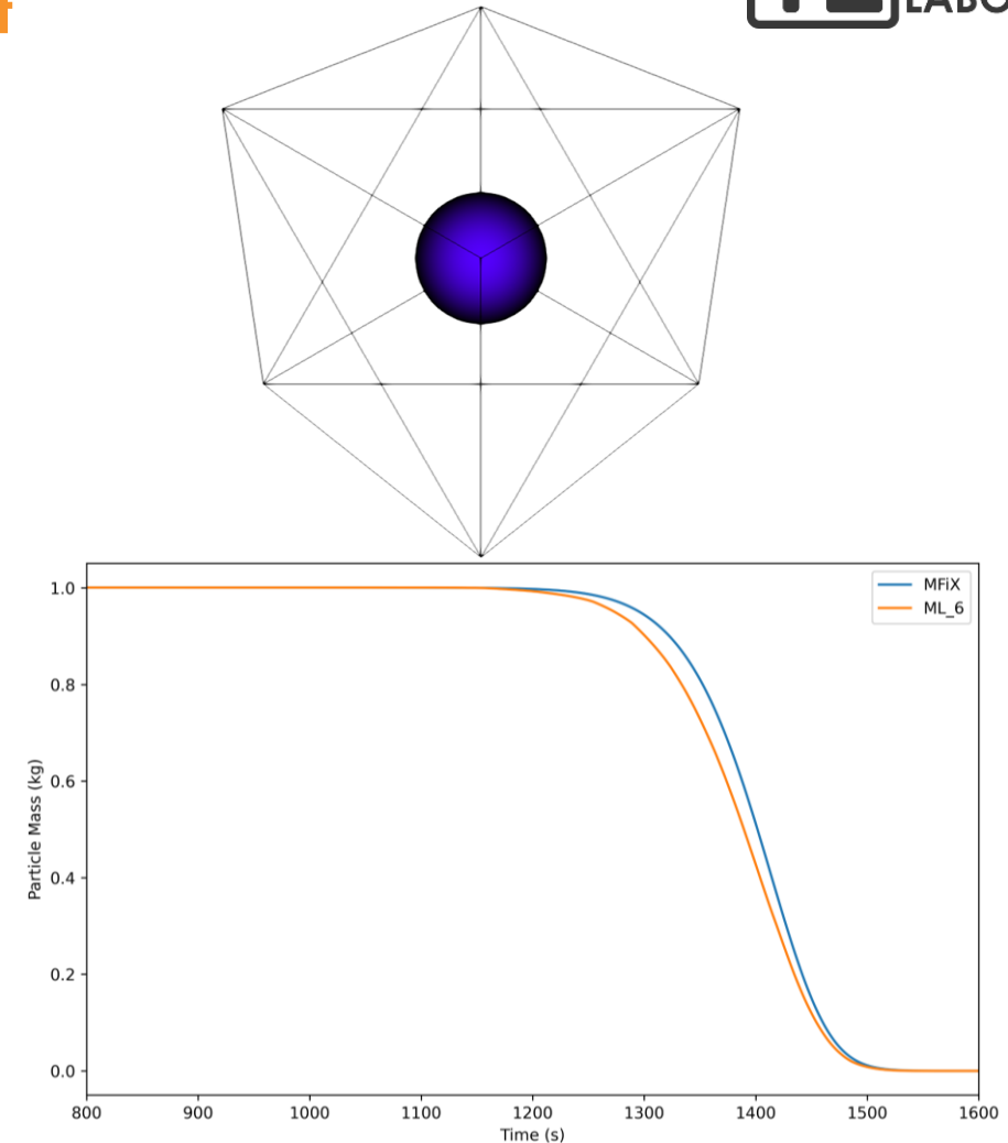
Figure 6. Top) Geometry setup of the MFiX simulation and bottom) prediction of particle mass loss compared to the stiff-solver.
