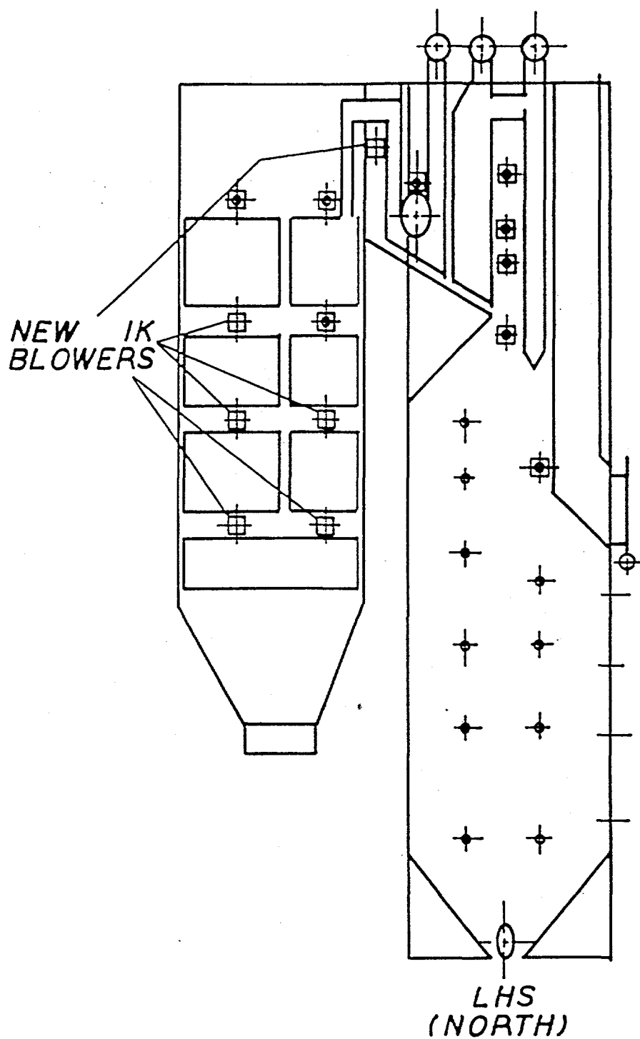
Figure 4-4. Edwards Unit 1 new sootblower locations
