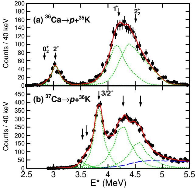
FIG. 1. Data points show the excitation-energy spectra of (a) ^{36}\text{Ca} from the invariant-mass of p+^{35}\text{K} events and (b) ^{37}\text{Ca} from p+^{36}\text{K} events. The red curves are from fits with multiple peaks each shown by the green dotted curves. No background was needed in fitting the ^{36}\text{Ca} data while the blue-dashed line in (b) indicates the background for the ^{37}\text{Ca} fit. Arrows indicate states included in the fits. The two states below the 3/2^+ level in (b) are fixed to the energies of states found in the \gamma -decay studies [20], while the states above the 3/2^+ state have not been previously observed.
