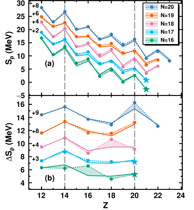
FIG. 7. (a) Proton separation energies for isotones from 16 \leq N \leq 20 . (b) Changes in proton separation energies for even Z isotones. Data are represented by points (or stars for new values) connected by dashed lines and are shifted up as indicated. Removing the Wigner energy results in the solid lines which show the trends for Z = 14 and Z = 20 .
