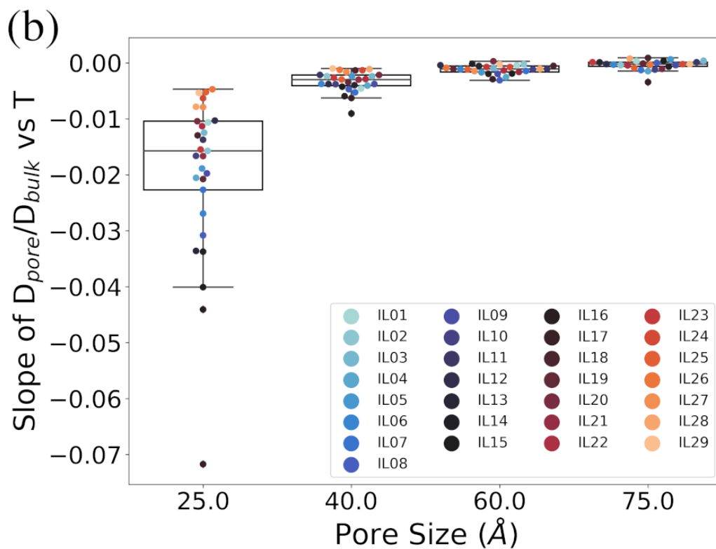
Supporting Figure 6: The slope of D_{pore} / D_{bulk} versus temperature for each ionic liquid ((a) cation, (b) anion) at each pore size. Box plots are shown to indicate the distribution of slopes across all ionic liquids for each pore size.
