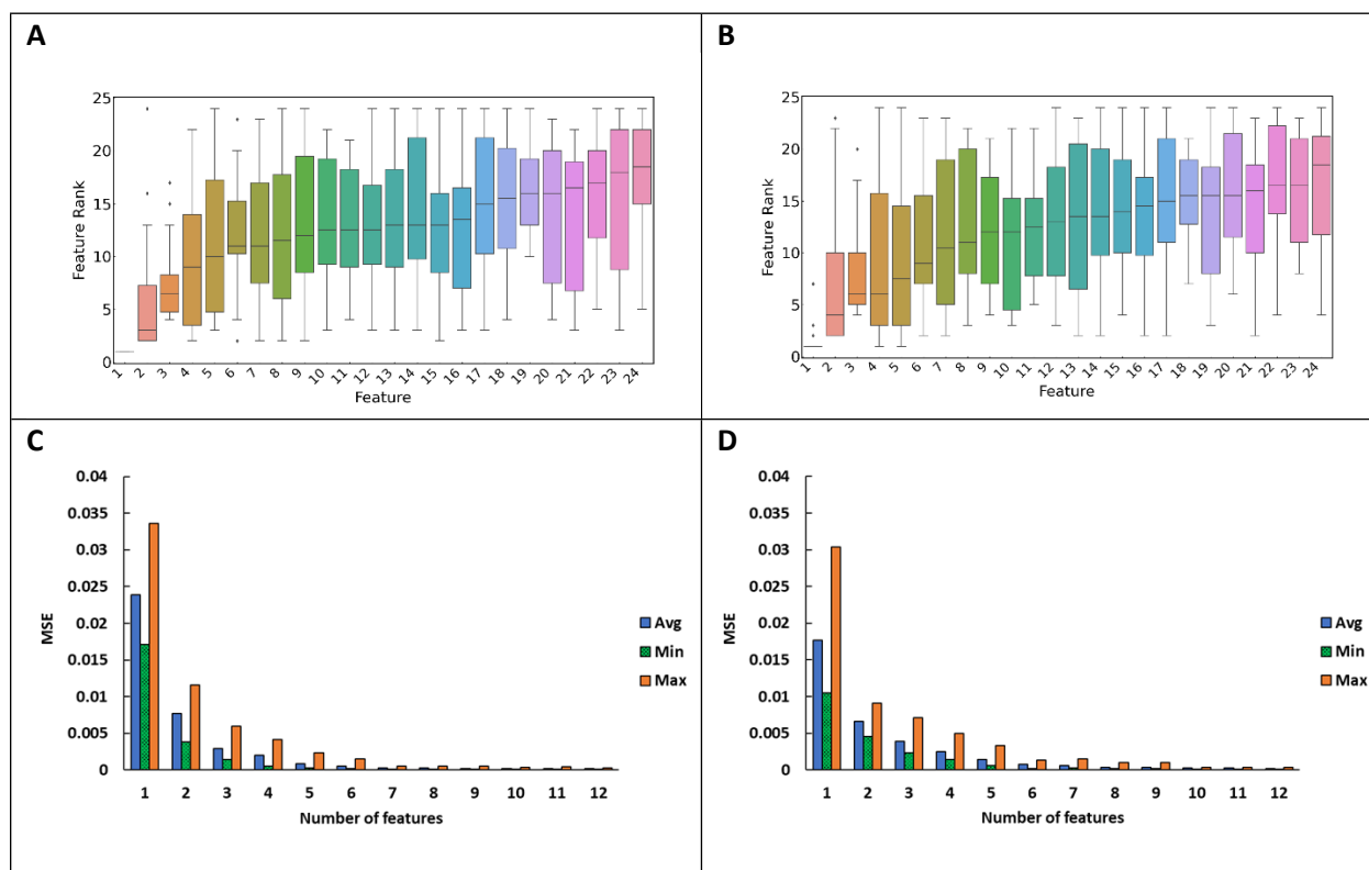
Figure 2: Results from feature importance testing. Boxplot of feature importance ranking for A) cations and B) anions. Trends in MSE with added C) cations and D) anions. The feature numbers on the x-axis in A and B correspond to the Meta Rank in Table 3.
