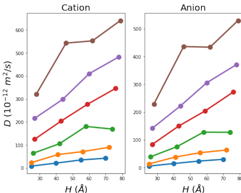
Figure 6: Results from MD simulations of IL7 confined in graphite slit pores, showing trends of cation and anion diffusion with slit pore height ( H ) and temperature (colors, blue 350 K, orange 380 K, green 410 K, red 440 K, purple 470 K, brown 500 K)
