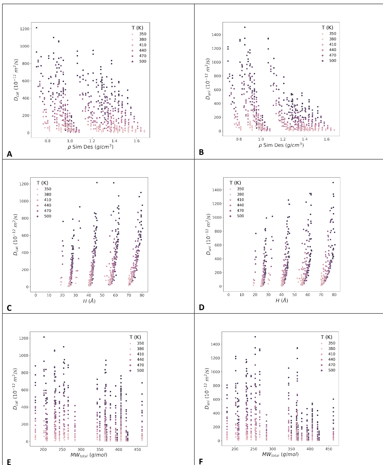
Supporting Figure 2: Correlations of D_{cat} and D_{anl} in confined ILs with fluid density (A, B), slit pore height (C, D), and IL molecular weight (E, F)
