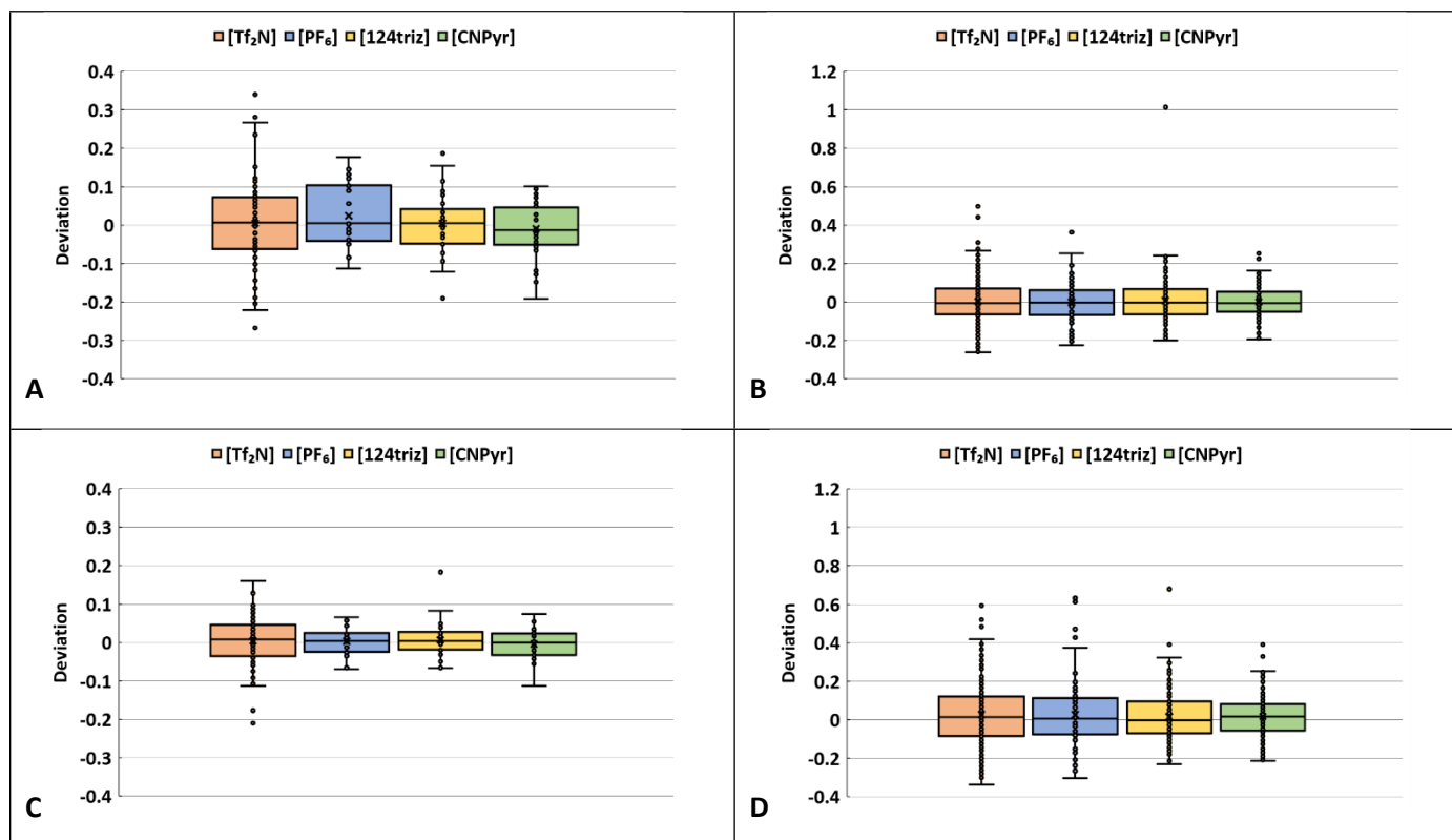
Figure 12: Box and whisker plots showing the relative deviation in D values for cations and anions for the ANN model trained on computed descriptors. The box represents the inner 50 percentile (ranging from 25 th -75 th percentile) and the whiskers are 1.5 times the 25 th and 75 th percentile. Each point represents one IL at a single temperature. The black horizontal line in the box is the median and the black X is the mean value. The ILs are sorted into four categories based on their respective anions: [Tf 2 N], [PF 6 ], [124triz], [CNPyr]. A) bulk IL, cation diffusion, B) confined IL, cation diffusion, C) bulk IL, anion diffusion, D) confined IL, anion diffusion
