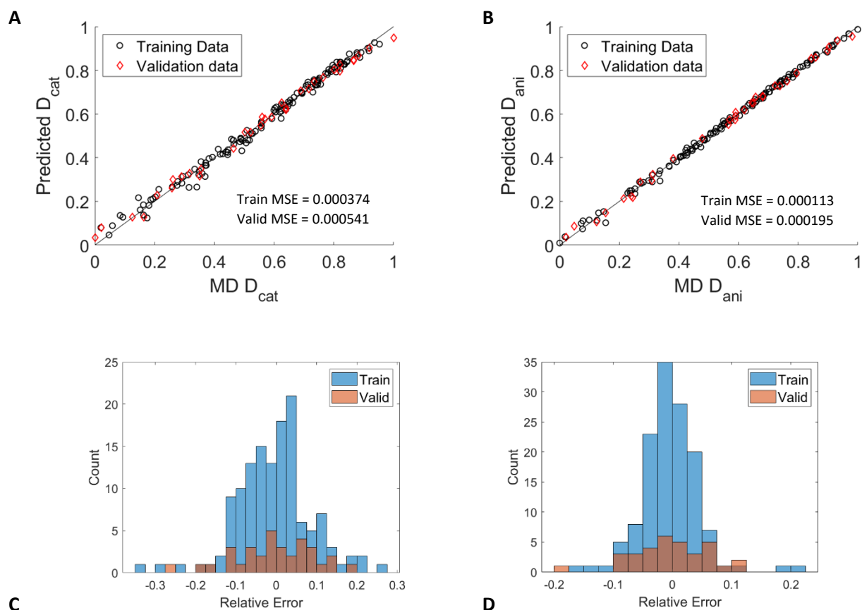
Figure 4: A) Parity plot of predicted diffusion (y-axis) for cations and diffusion from MD simulations (x-axis), B) parity plot results for anions, C) relative error distribution for cations, D) relative error distribution for anions
