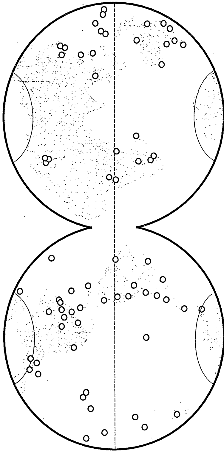
Figure 1. EML global fallout sampling stations during 1987 through 1990
