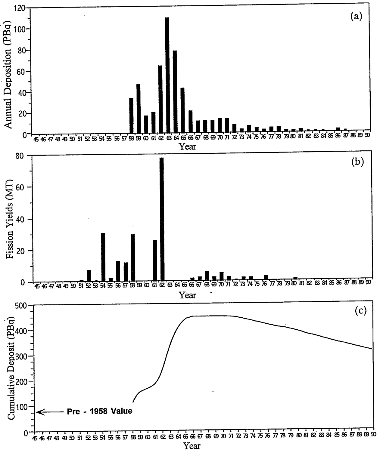
Figure 3. Temporal patterns of atmospheric weapons testing and ^{90}\text{Sr} deposition: (a) annual global ^{90}\text{Sr} deposition from 1958 to 1990 (b) annual fission yield from atmospheric weapons testing (c) cumulative global deposit of ^{90}\text{Sr} from 1958 to 1990
