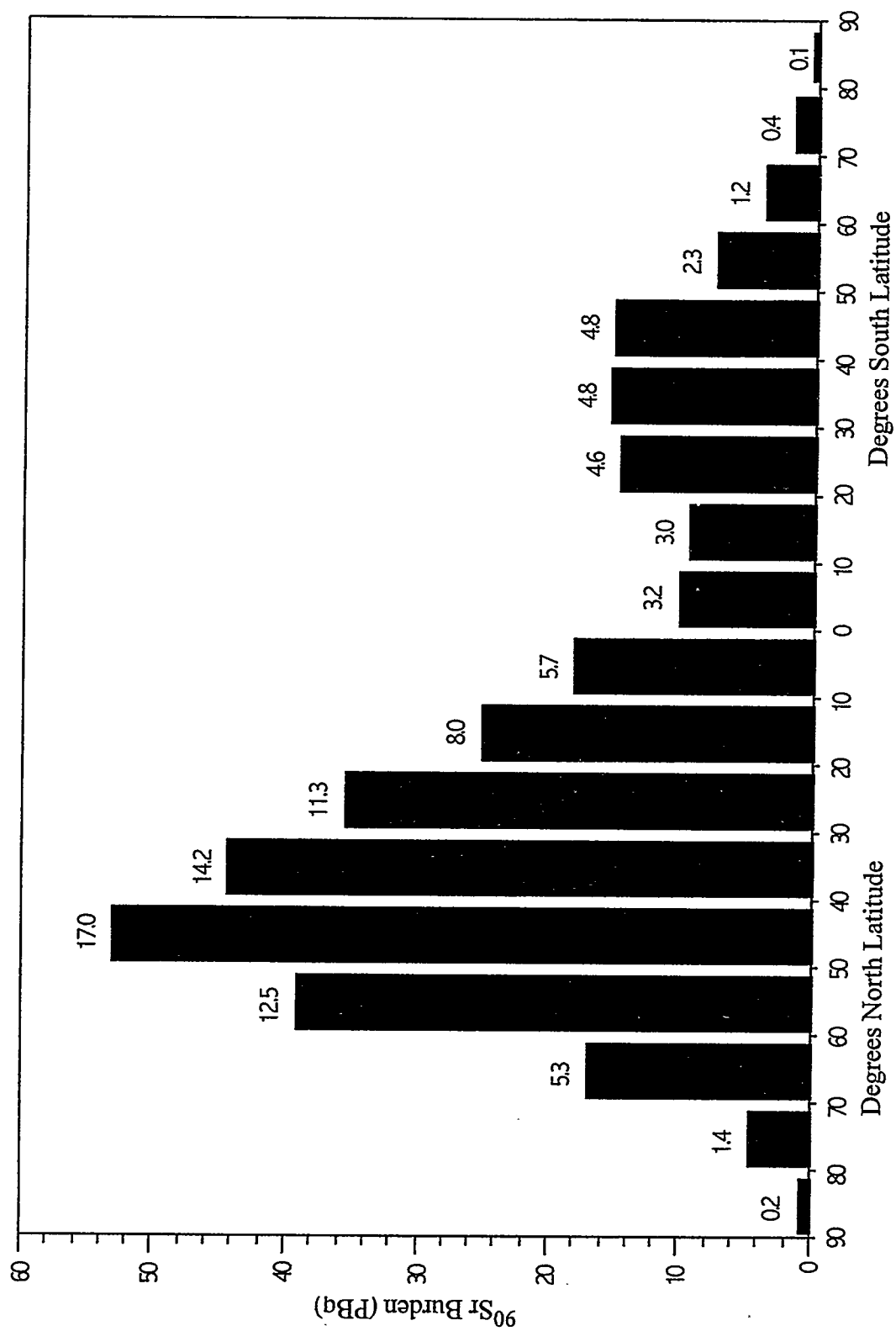
Figure 2. Latitudinal distribution of global ^{90}\text{Sr} burden at the end of 1990
