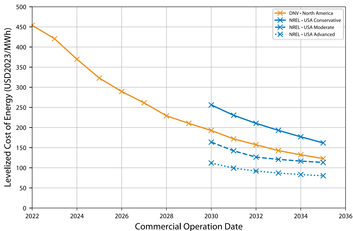
Figure 32. Unsubsidized levelized cost of energy estimates for floating offshore wind technologies in the United States.
