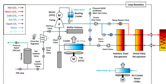
FIGURE 4: SUPERCRITICAL CARBON DIOXIDE COOLING LOOP PROCESS DIAGRAM
