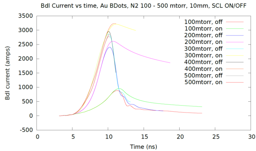
Figure 4.9 Bdl Current vs time for N_2 between 100 and 500 mTorr for a 10 mm Au B-Dot system, with SCL emission toggled on/off. These currents are much higher than Ne.
