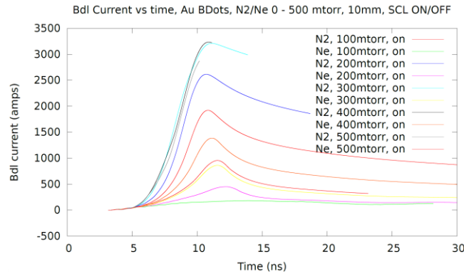
Figure 4.24 Bdl current vs time for 10 mm Au B-Dot, Ne and N 2 gas comparison, SCL on.
