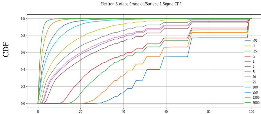
Figure 4.3 Convergence testing data from the MC electron/photon code for surface 1. The CDF shows the percent of energies with uncertainties below a given value.
