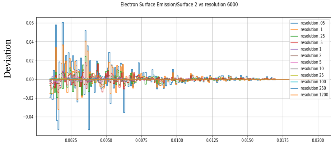
Figure 4.2 Convergence testing data from ITS for surface 2, a plot of the difference in the spectrum for different number of histories for the true spectrum of Au.
