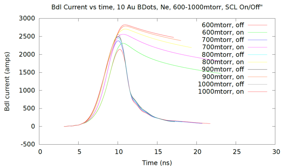
Figure 4.16 Bdl Current vs time for Ne between 600 and 1000 mTorr for a 10 mm Au B-Dot system, with SCL emission toggled on/off.
