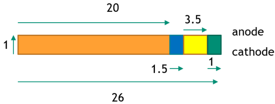
Figure 3.17 Sketch of the simplified 1 mm B-Dot photoemission cavity with dimensions in mm. The orange region is the photoemission region, with the top and bottom surfaces being the AK gap. All the distances are radii, and they are reflected about the far left of the sketch (like Figure 1.1). Photons come in from the top.
