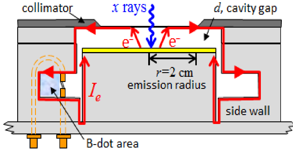
Figure 1.1 B-Dot sensor circuit schematic. The pulse creates a current, which induces a magnetic field in the sensor circuit, producing a voltage in the sensor circuit [3].
