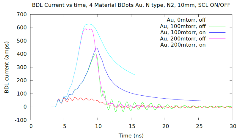
Figure 4.10 Bdl Current vs time for N_2 between vacuum and 200 mTorr for a 10 mm Au B-Dot system, with SCL emission toggled on/off. These currents are much higher than Ne.
