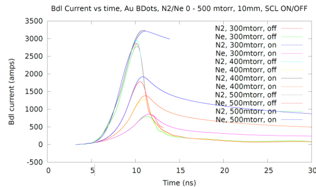
Figure 4.12 Direct comparison of Bdl Current vs time for Ne and N 2 fill gasses at high pressures.
