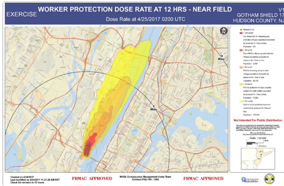
Figure 8. Worker Protection Dose Rate at 12 Hrs 0 - Near Field (Example)
