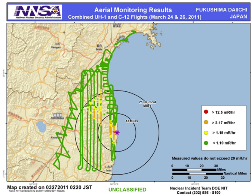
Figure 7. Aerial Monitoring Results (Example)
