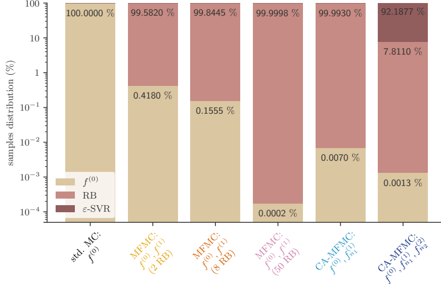
Figure 7: Thermal block: Sample distribution across models for budget p = 50 seconds.
