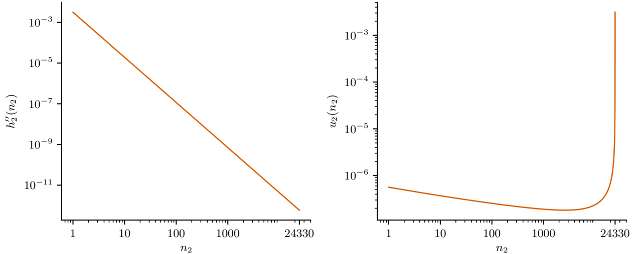
Figure 11: ASDEX Upgrade Experiment: On the left, we verify that h_2'' > 0 satisfies (3.14) up to budget p = 10^7 seconds. On the right, we plot the objective u_2 defined in (3.13), which has a unique global minimizer.
