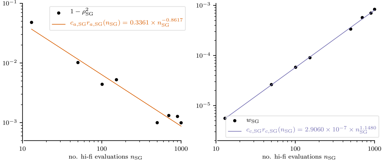
Figure 8: ASDEX Upgrade Experiment: Estimated accuracy (left) and evaluation cost rates (right) for the SG low-fidelity model.
