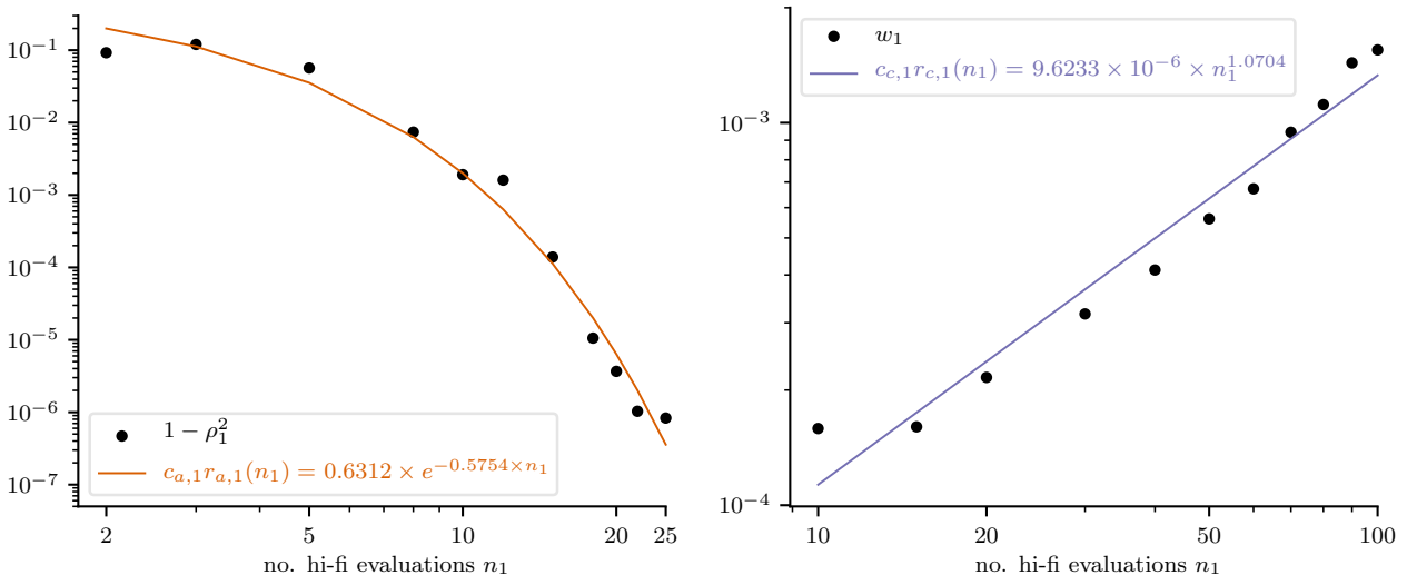
Figure 1: Thermal block: Estimated accuracy (left) and evaluation cost rates (right) for the RB low-fidelity model.
