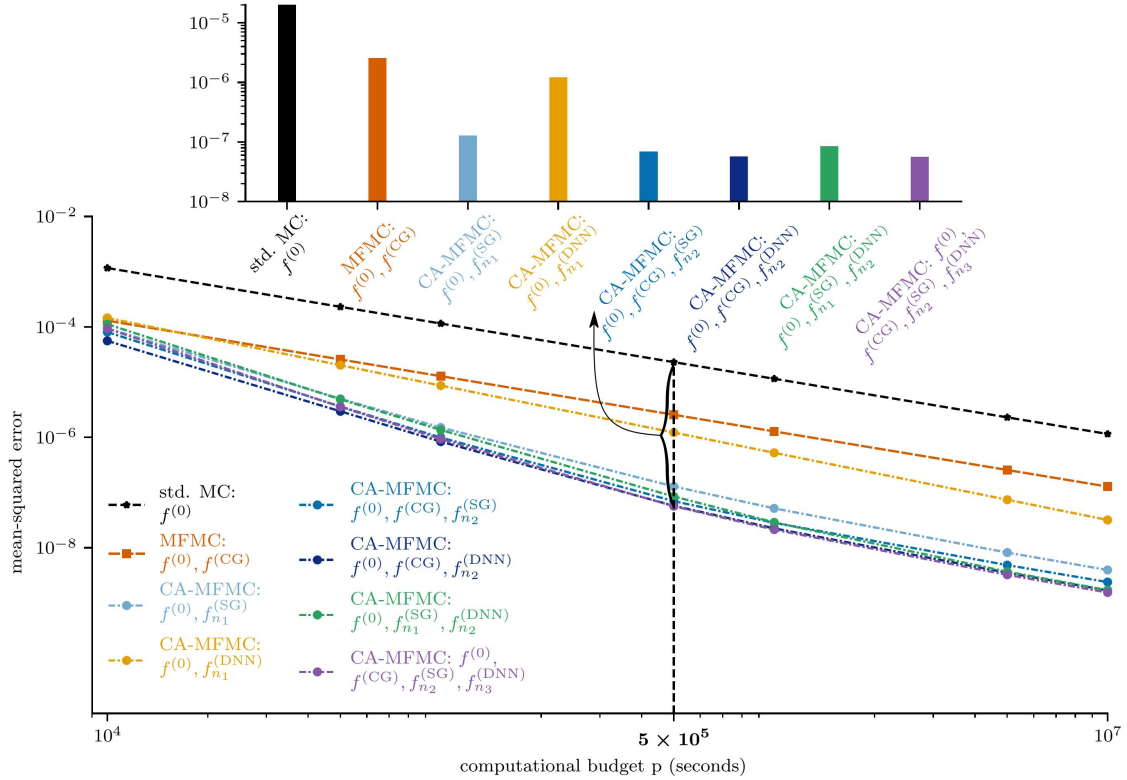
Figure 10: ASDEX Upgrade Experiment: Combinations of models can be selected based on the analytical MSE, which can be computed without additional model evaluations as long as the accuracy and cost rates are available. In this example, the CA-MFMC estimator with the high-fidelity model f^{(0)} , the coarse-grid low-fidelity model f^{(1)} = f^{(\text{CG})} and either the SG low-fidelity model f_{n_2}^{(2)} = f_{n_2}^{(\text{SG})} or the DNN low-fidelity model f_{n_2}^{(2)} = f_{n_2}^{(\text{DNN})} have the highest (best) cost/error ratio, which indicates a good model selection.
