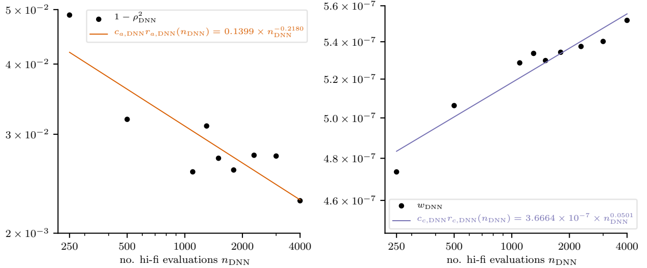
Figure 9: ASDEX Upgrade Experiment: Estimated accuracy (left) and evaluation cost rates (right) for the DNN low-fidelity model.
