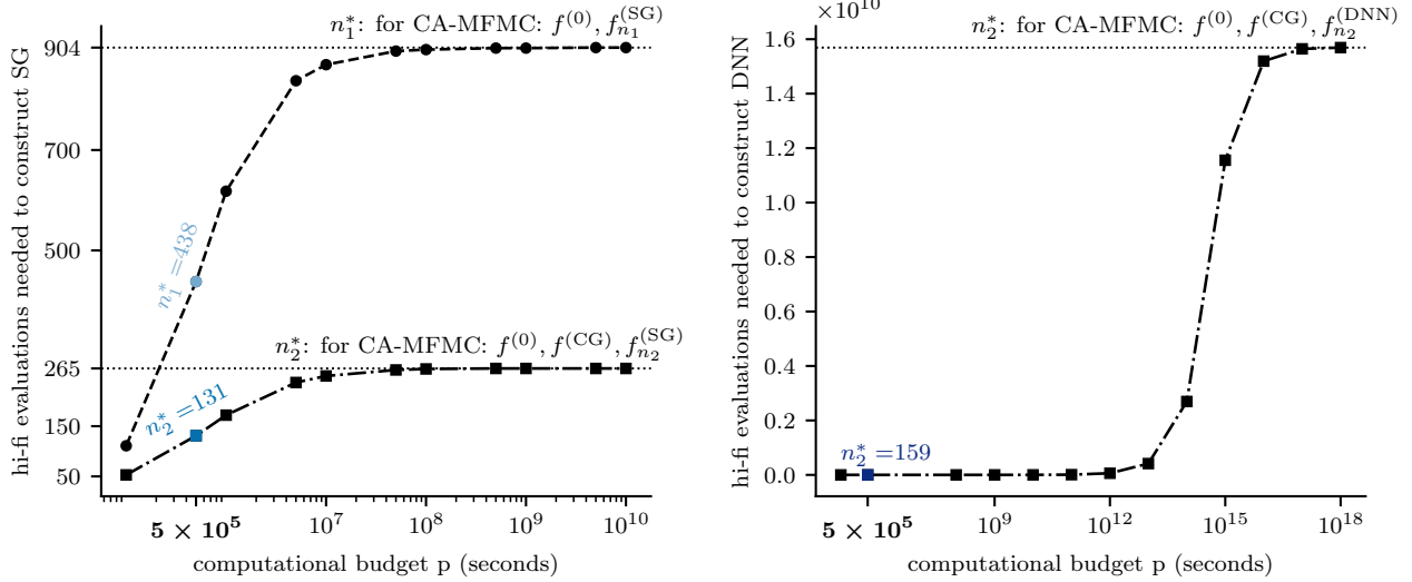
Figure 12: ASDEX Upgrade Experiment: The number of high-fidelity training samples selected by the proposed context-aware approach for obtaining a multi-fidelity estimator with highest (best) cost/error ratio.
