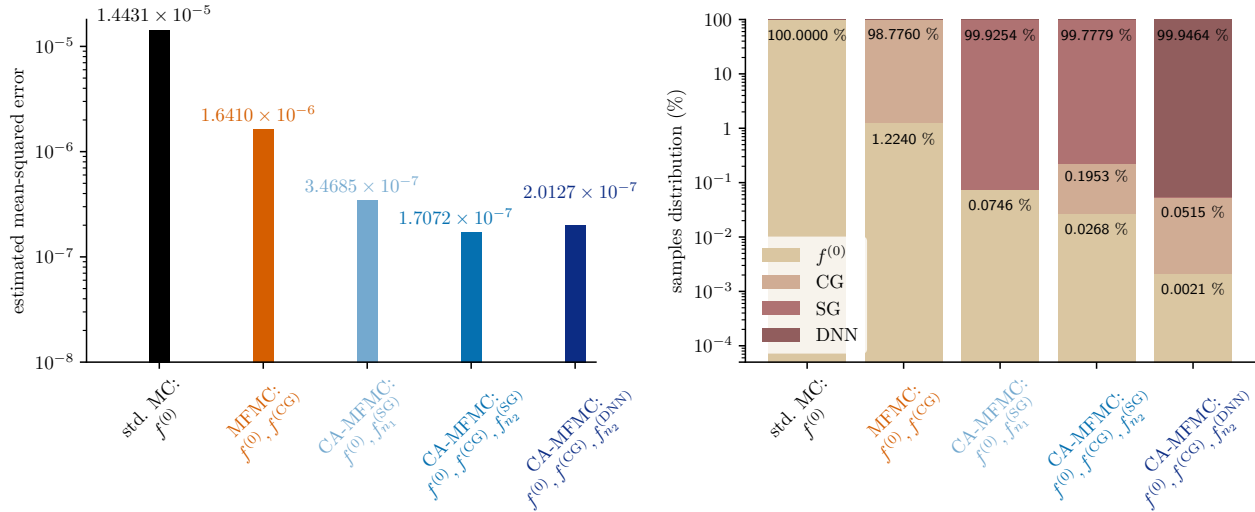
Figure 13: ASDEX Upgrade Experiment results for budget p = 5 \times 10^5 seconds : The left plots show that the CA-MFMC estimators achieve about two orders of magnitude speedup, which translates into a runtime reduction from 72 days to roughly four hours on one node of the Lonestar6 supercomputer. The right plot shows the sample distribution across models in the employed estimators. The static MC and MFMC estimators use the entire computational budget for sampling only, whereas the context-aware estimators use the remaining budget after the low-fidelity models are constructed.
