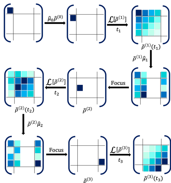
FIG. 2. Schematic illustration of the 2DES simulation algorithm, with one possible path [see Eq. (4) for all possible paths]. The color gradients imply the magnitude of the density matrix elements. \mathcal{L} indicates the overall time evolution by the \mathcal{L} -PLDM approach [see Eq. (29)], and \mu_i \tilde{\rho}^{(i)} (or \tilde{\rho}^{(i)} \mu_i ) indicate the dipole operator acting on the density matrix from the left-hand (right hand) side at time t = t_i .
