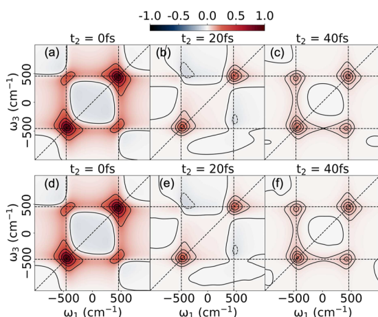
FIG. 11. 2DES spectra of a monomer coupled to the cavity. The same model parameters are used as in Fig. 10, except for the cavity loss rate \Gamma = 50 \text{ meV} . The spectra are calculated with (a)–(e) Lindblad and (d)–(f) \mathcal{L} -PLDM dynamics.
