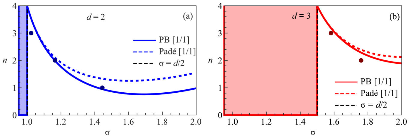
FIG. 1. Resummed values of n_c(\sigma) obtained by the Padé approximant [1/1] (dashed lines) and Padé-Borel resummation (solid lines) for d=2 (a) and 3 (b). For the region of values n and \sigma above the lines, the pure long-range universality class holds, while the new disorder long-range universality class is induced for the values below the lines. Dots show results that follow from the interpolation of the NPRG data of Ref. 15. The mean-field behavior holds for \sigma < d/2 (regions separated by vertical dashed lines).
