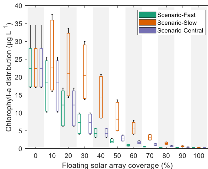
Fig. 4. Total chlorophyll- a (based on the mean of a window, \pm five days, around the day of maximum total chlorophyll- a ) versus floating solar array coverage. Whiskers represent the minimum and maximum of the simulation results presented. The box represents the 2.5th & 97.5th percentiles, which gives a 95% confidence interval that simulation estimates fall within this range. 0% floating solar coverage represents QEII reservoir simulated as a baseline.
