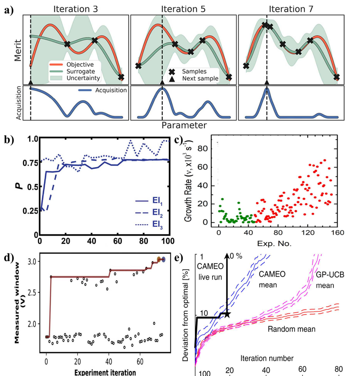
Figure 11. (a) Schematics of BO. Reproduced with permission from Ref.[103], Copyright 2021 American Chemical Society. (b) Evolution of the performance of the mechanical structures obtained from BEAR. Reproduced under a Creative Commons Attribution License 4.0 (CC BY 4.0) from Ref.[70], Copyright 2020 AAAS. (c) Evolution of the growth rates of CNTs obtained from BO. Reproduced under a Creative Commons Attribution 4.0 International License (CC BY 4.0) from Ref. [427], Copyright 2020 Springer Nature. (d) Evolution of the potential window of
