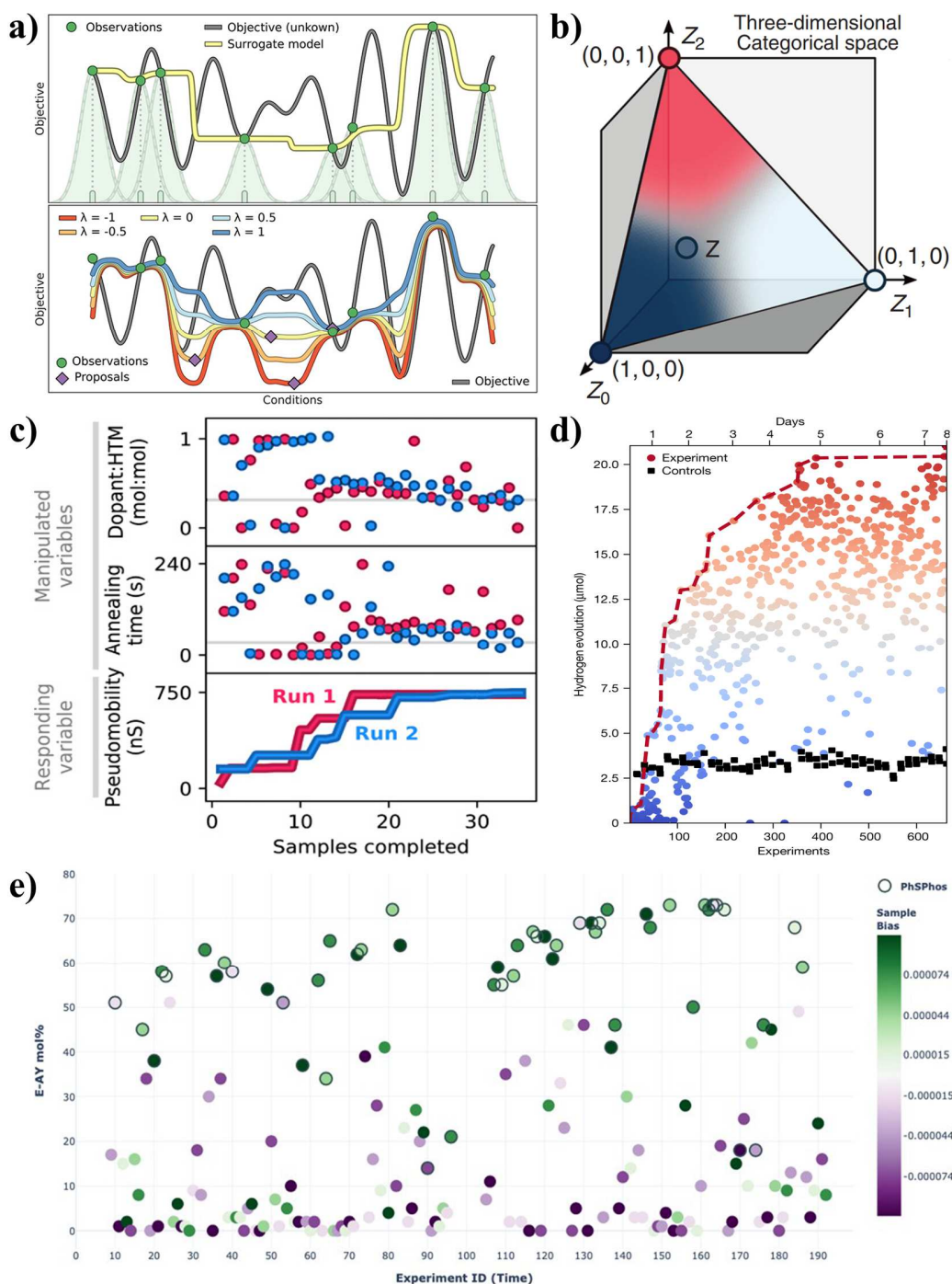
Figure 12. (a) Schematics of Phoenix for optimizing continuous parameters. Reproduced with permission from Ref.[453], Copyright 2018 American Chemical Society. (b) Schematics of Gryffin for optimizing categorical inputs. Reproduced with permission from Ref.[454], Copyright 2021 AIP Publishing. (c) Evolution of the pseudomobilty of thin-film materials
