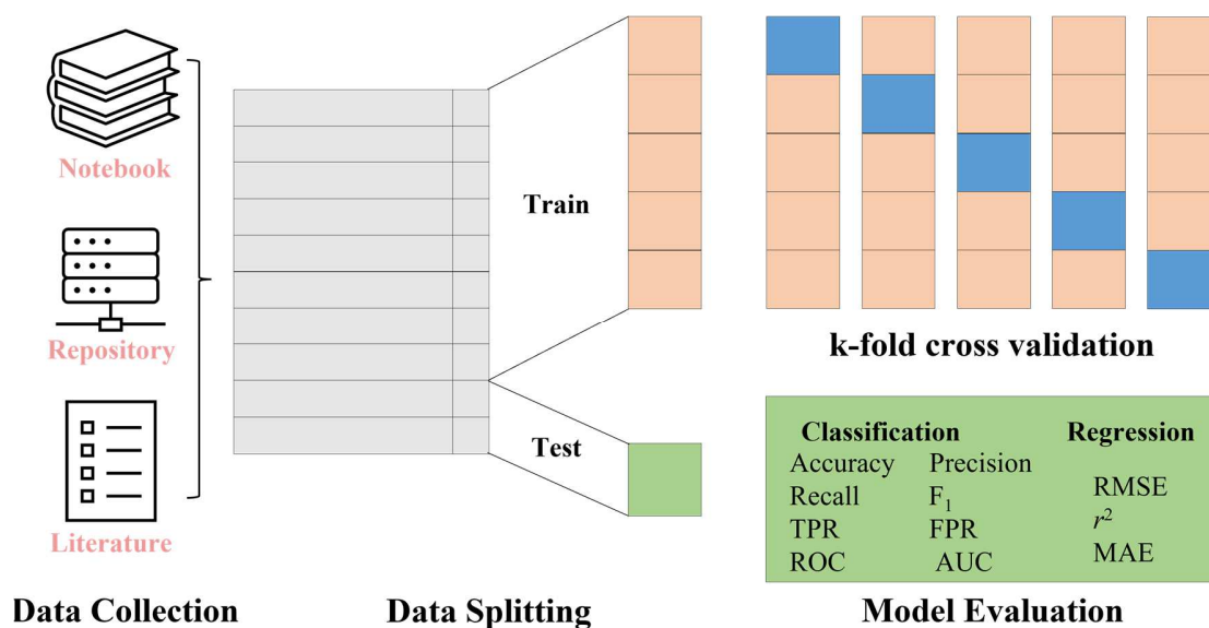
Figure 4. Workflow of building ML/DL models.
