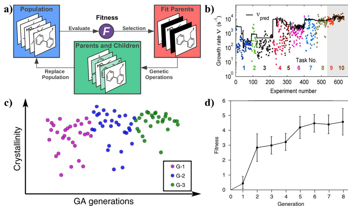
Figure 15. (a) Schematic of a typical GA. Reproduced under Creative Common Attribution 4.0 International License (CC BY 4.0) from Ref.[103], Copyright 2021 American Chemical Society. (b) Evolution of the growth rates of CNTs by GA/RF. Reproduced under Creative Common Attribution 4.0 International License (CC BY 4.0) from Ref.[433], Copyright 2016 Springer Nature. (c) Evolution of the crystallinity of MOFs by GA/RF. Reproduced under Creative Common Attribution 4.0 International License (CC BY 4.0) from Ref.[47], Copyright 2019 Springer Nature. (d) Evolution of the fitness function of gold nanoparticles with octahedron shape by GA. Reproduced under Creative Common Attribution 4.0 International License (CC BY 4.0) from Ref.[434], Copyright 2020 Springer Nature.
