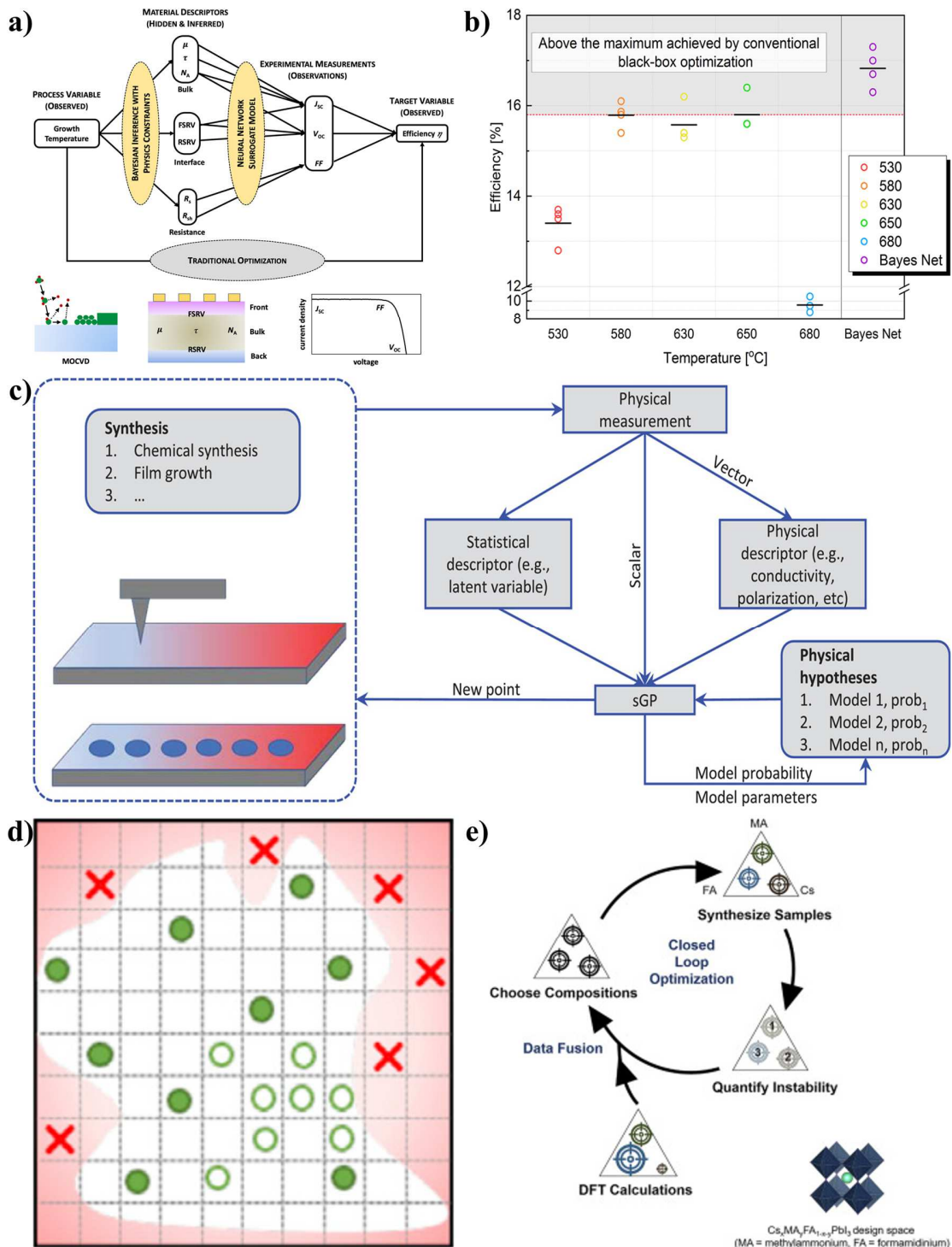
Figure 17. (a) Workflow of a two-step BO network. (b) Comparison of photovoltaic efficiency obtained from the BO net and the random search method. Reproduced under a Creative Commons Attribution 4.0 International License (CC BY 4.0) from Ref.[482], Copyright 2020
