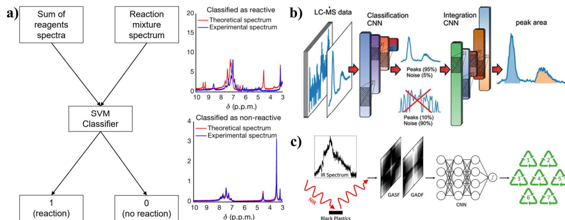
Figure 9. (a) Schematic showing workflow and results of an SVM classifier for reaction outcome detection from NMR spectra. Reproduced with permission from Ref.[64], Copyright 2018 Springer Nature. (b) The architecture of the peakonly model for peak classification and integration. Reproduced with permission from Ref.[99], Copyright 2020 American Chemical Society. (c) Workflow of a CNN framework for classifying different types of plastic using a GAF transformation method. Reproduced with permission from Ref.[239], Copyright 2021 American Chemical Society.
