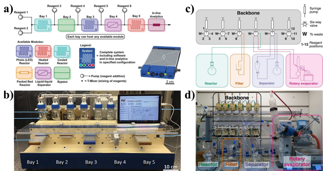
Figure 6. (a) Schematics and (b) photograph of a plug-and-play, reconfigurable, continuous-flow chemical synthesis system. Reproduced with permission from Ref. [344] , Copyright 2018 AAAS. (c) Schematics and (d) photograph of the Chemputer setup. Reproduced with permission from Ref. [68] , Copyright 2019 AAAS.
